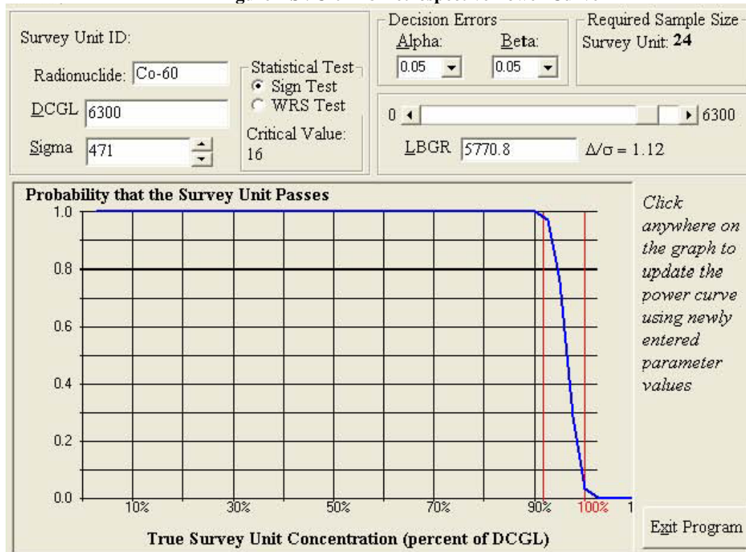
Figure 2 SVC-01-18 Retrospective Power Curve
