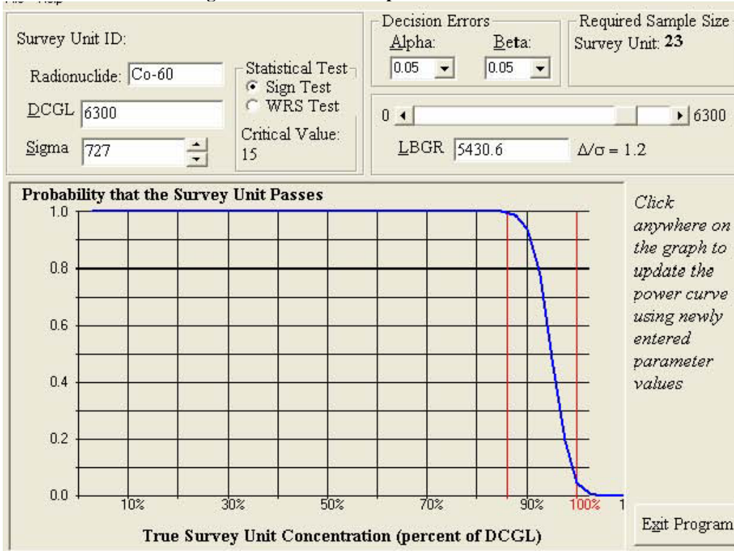
Figure 1 SVC-01-18 Prospective Power Curve
