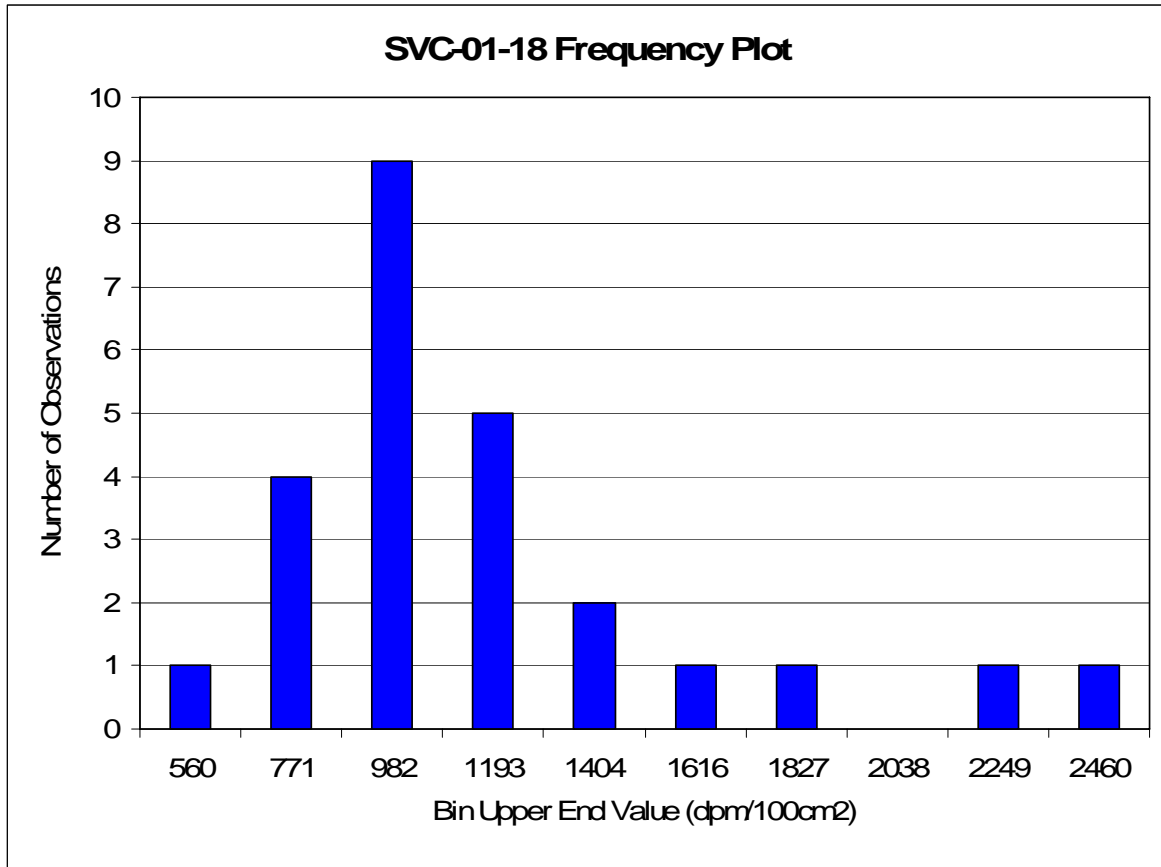
Figure 5 SVC-01-18 Total Activity Frequency Plot
