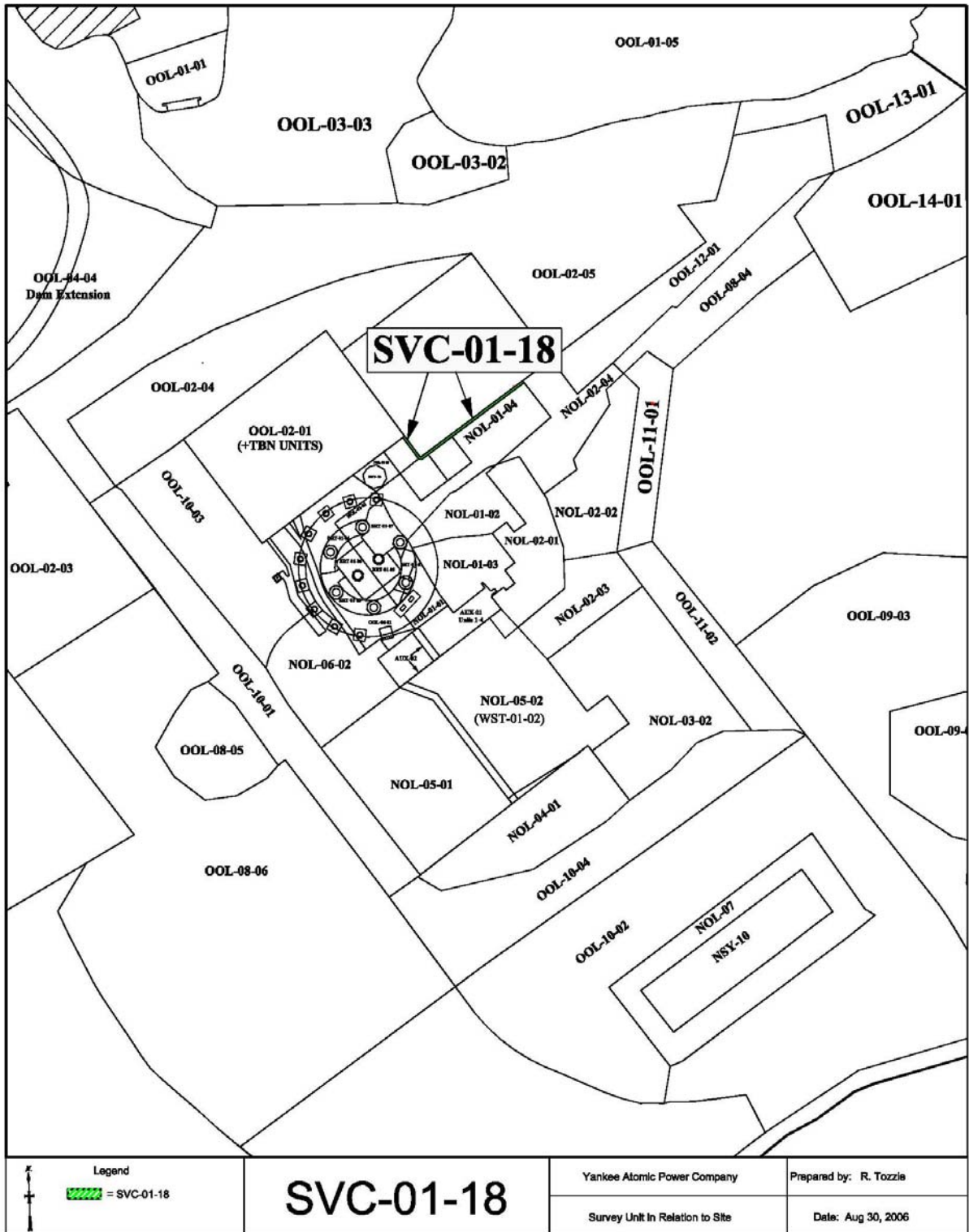
Figure 1 SVC-01 Relative to Structures
