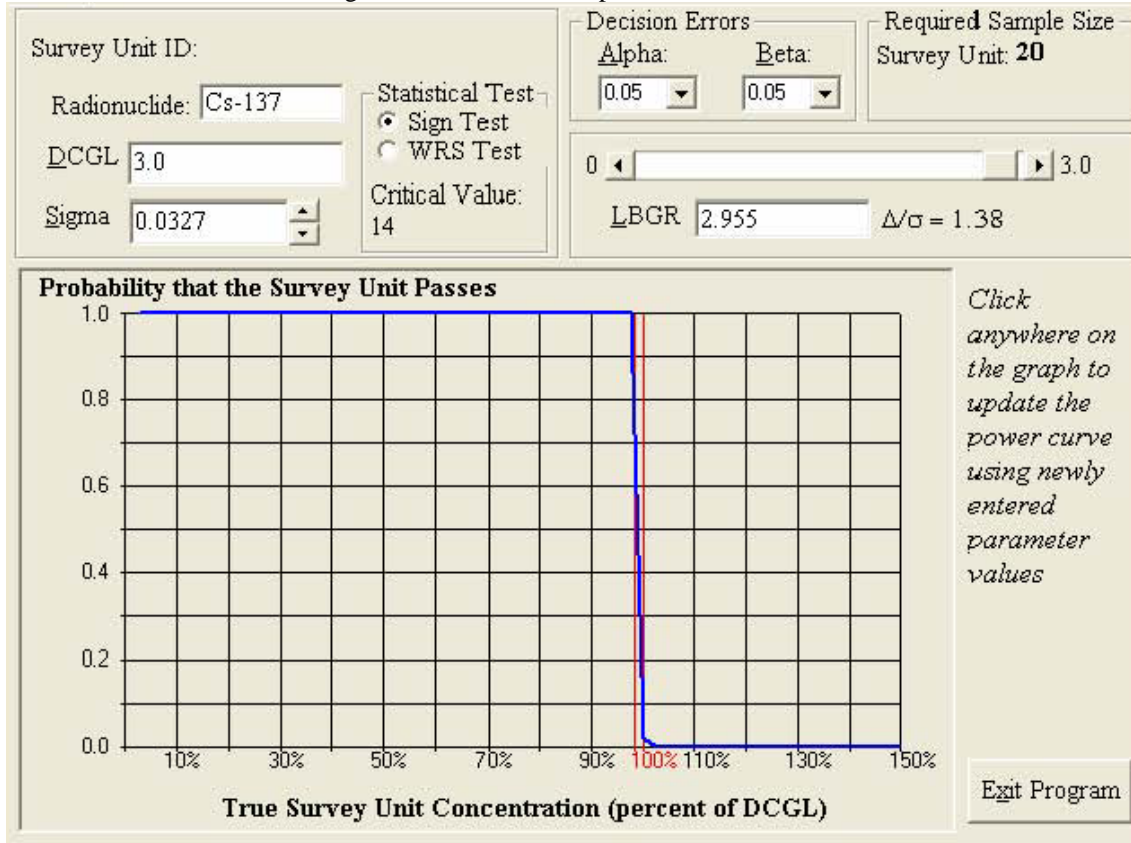
Figure 1 OOL-16-01 Prospective Power Curve
