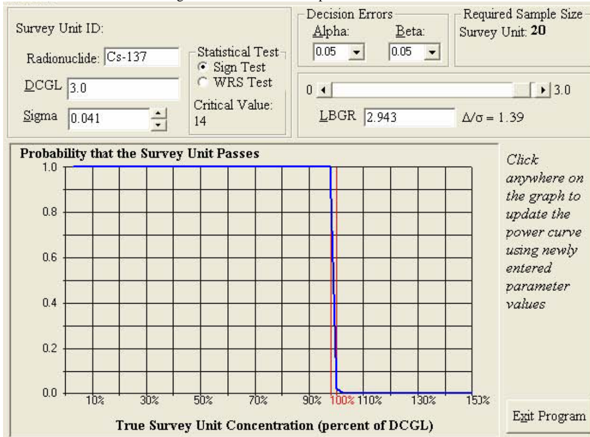
Figure 2 OOL-16-01 Retrospective Power Curve
