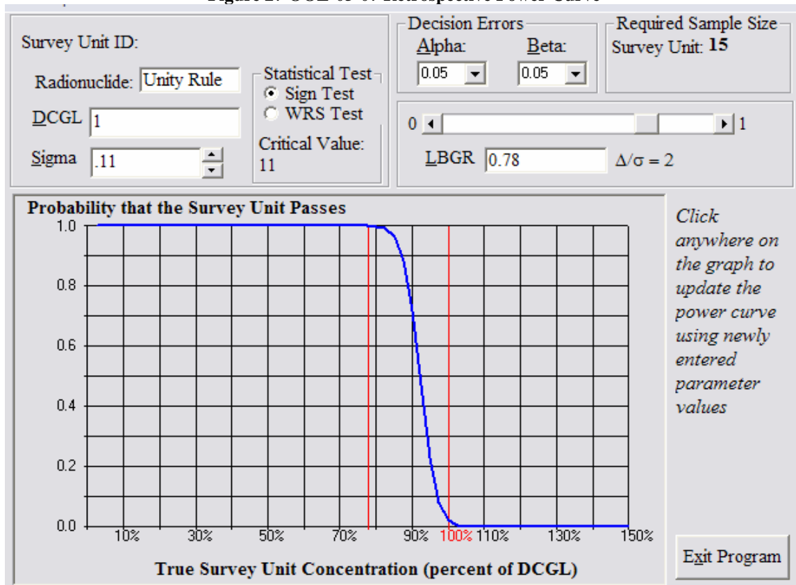
Figure 27 OOL-05-07 Retrospective Power Curve
