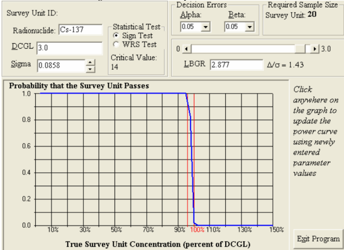
Figure 21 OOL-05-06 Prospective Power Curve
