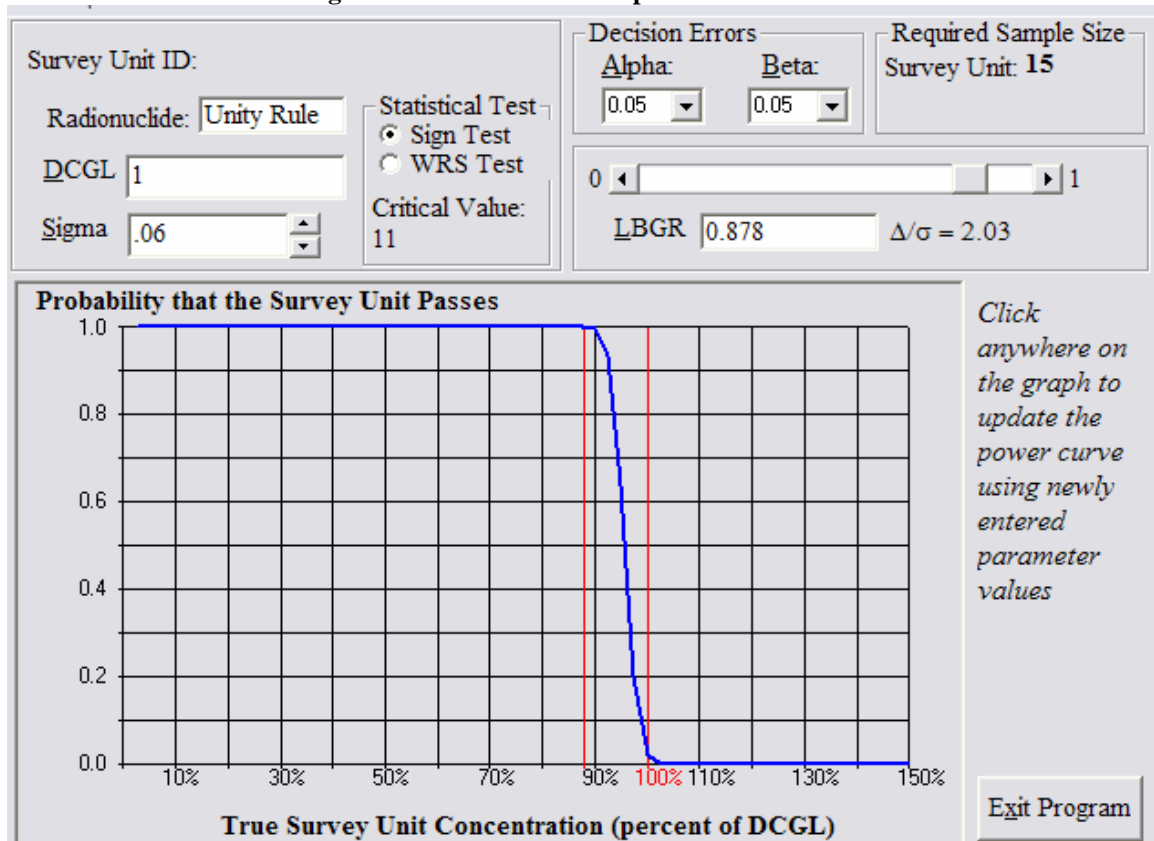
Figure 12 OOL-05-04 Retrospective Power Curve
