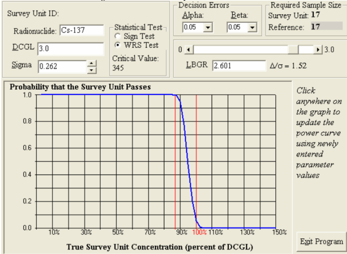
Figure 1 OOL-05-01 Prospective Power Curve
