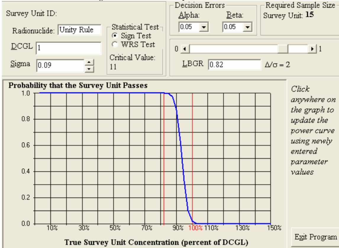
Figure 26 OOL-05-07 Prospective Power Curve
