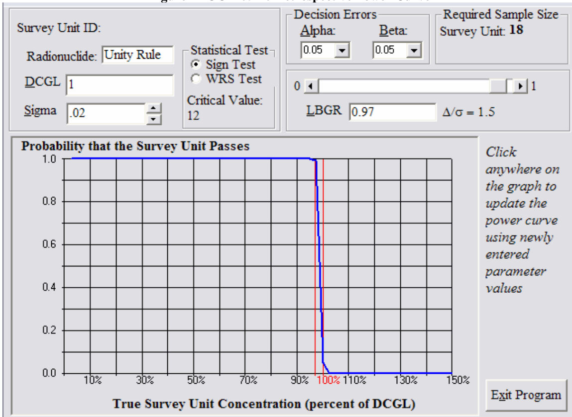
Figure 42 OOL-05-10 Retrospective Power Curve
