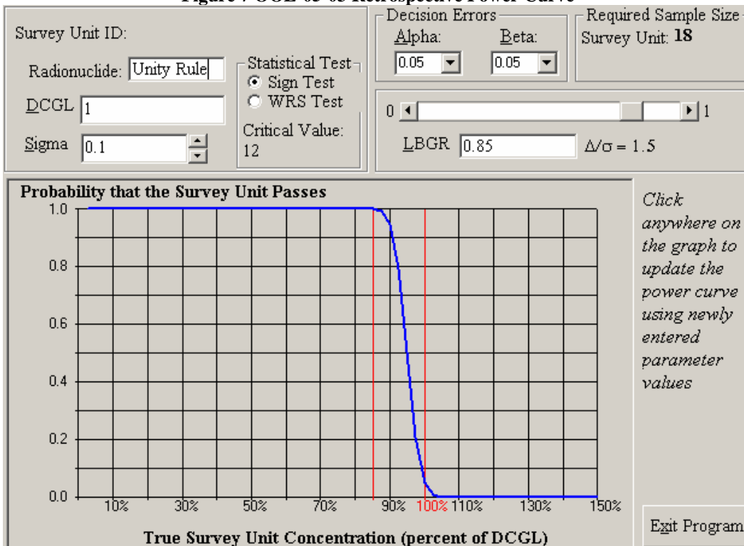
Figure 7 OOL-05-03 Retrospective Power Curve
