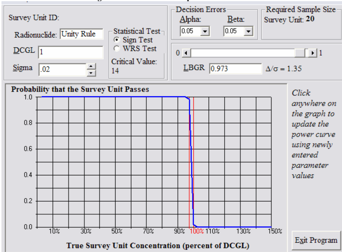
Figure 37 OOL-05-09 Retrospective Power Curve
