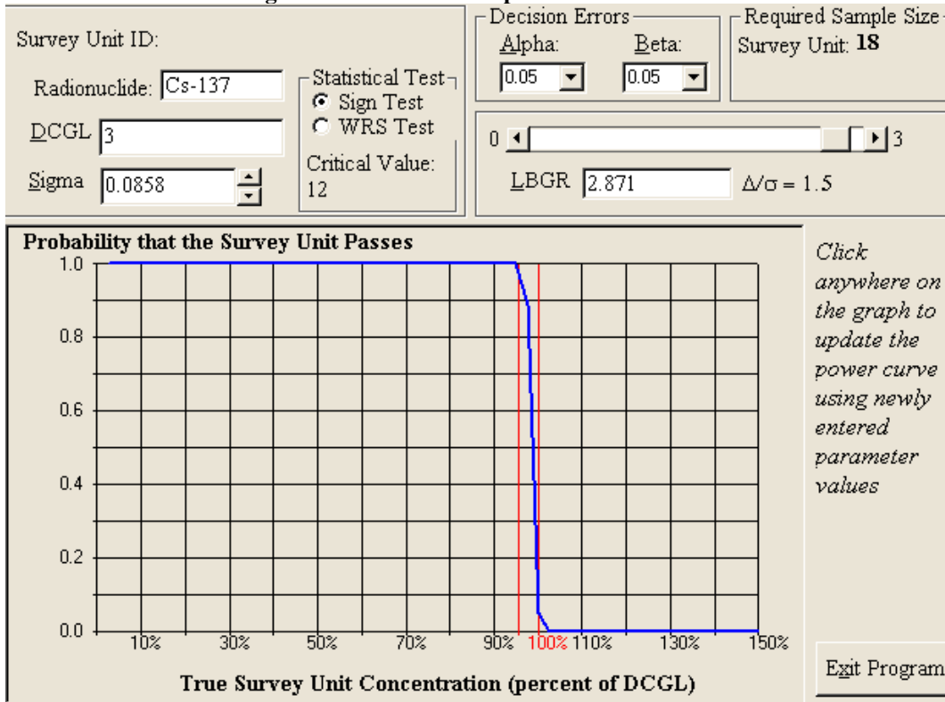
Figure 6 OOL-05-03 Prospective Power Curve
