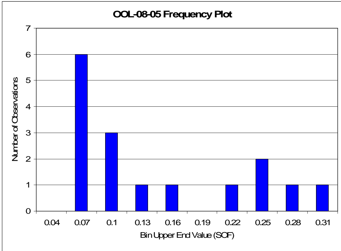
Figure 25 OOL-08-05 Sum of Fractions Frequency Plot
