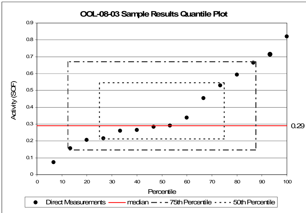
Figure 14 OOL-08-03 Sum of Fractions Quantile Plot
