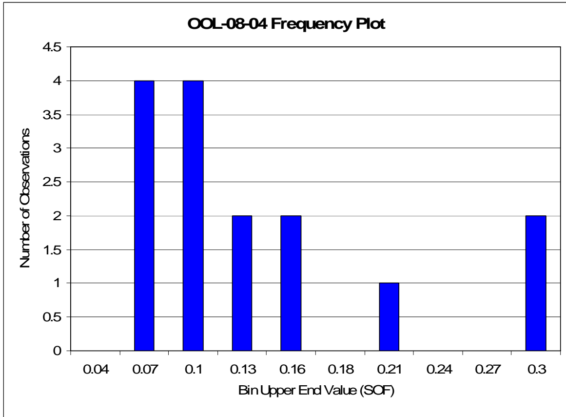
Figure 20 OOL-08-04 Sum of Fractions Frequency Plot
