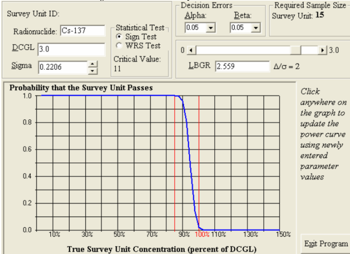
Figure 16 OOL-08-04 Prospective Power Curve
