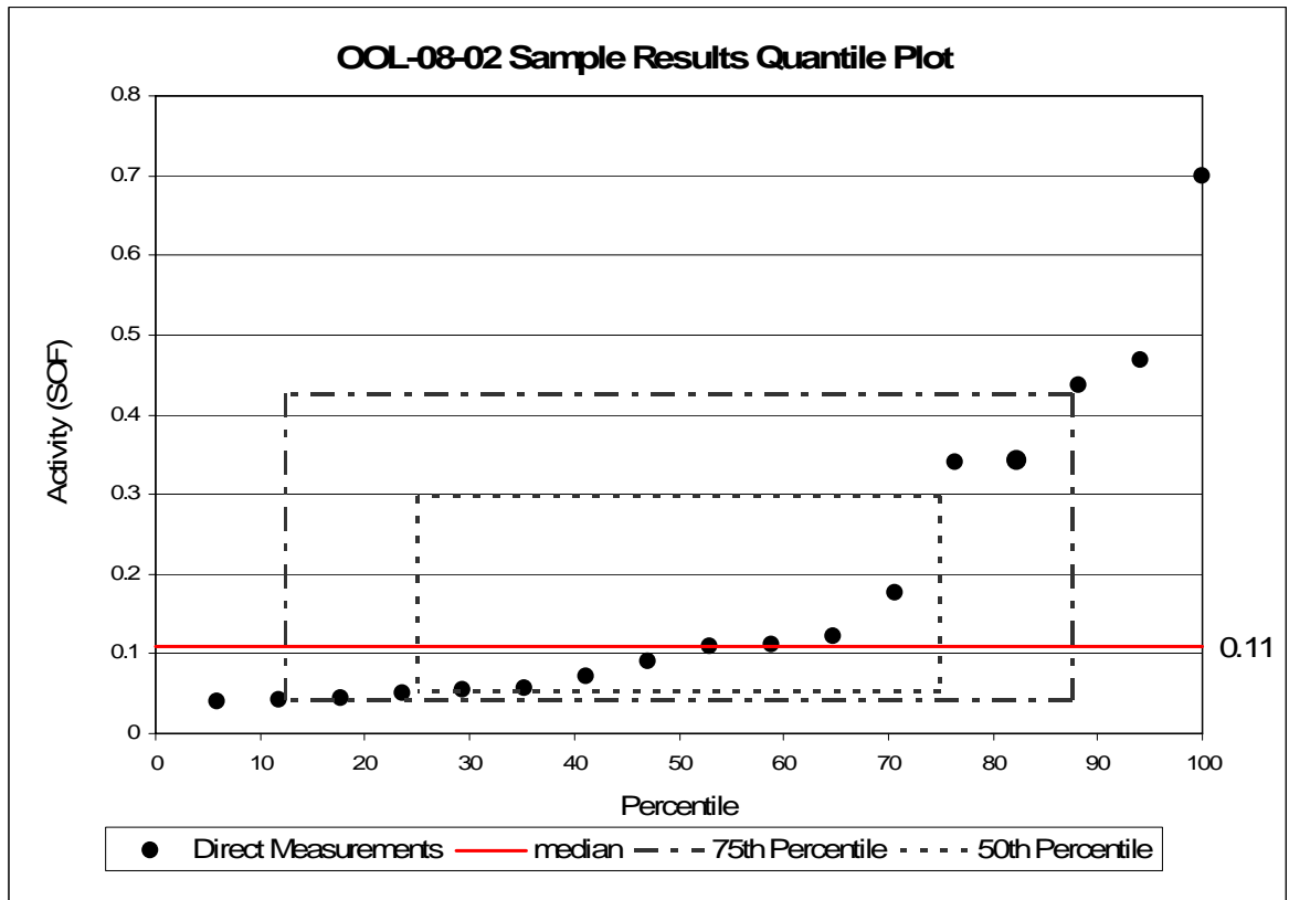
Figure 9 OOL-08-02 Sum of Fractions Quantile Plot
