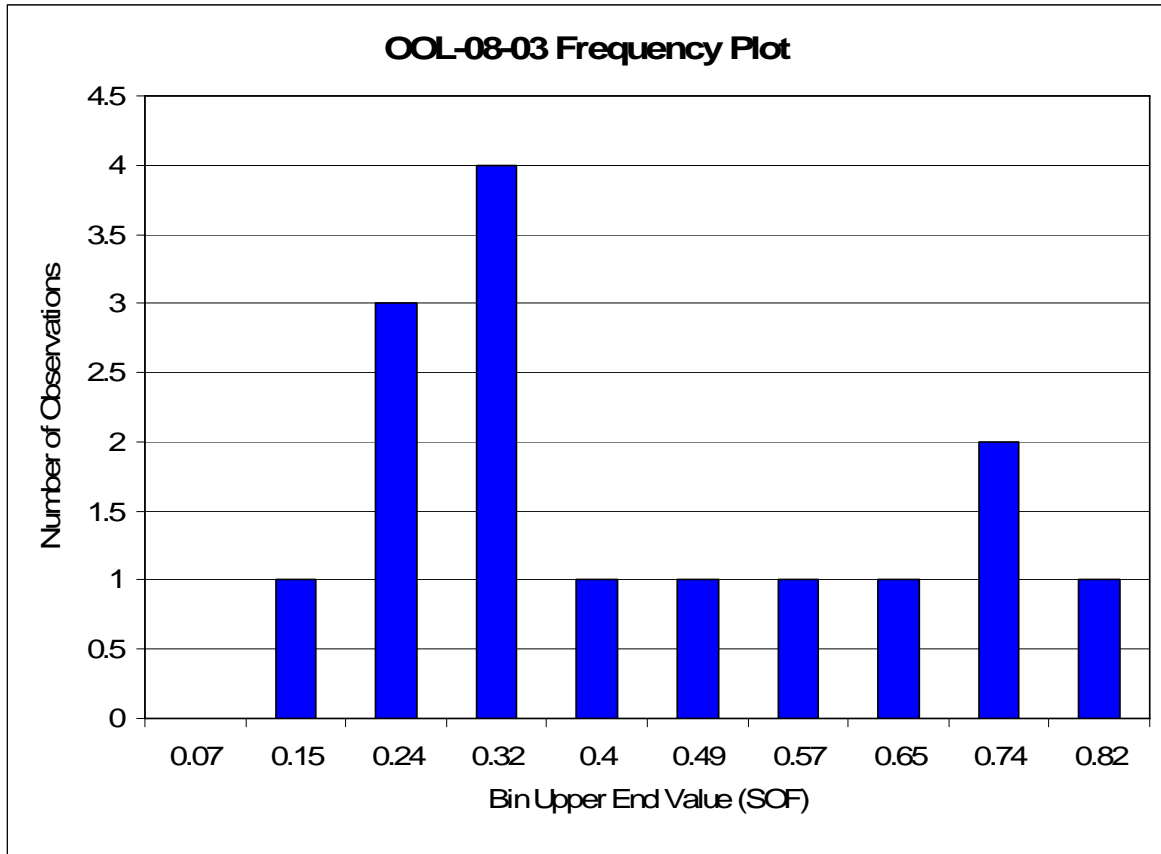
Figure 15 OOL-08-03 Sum of Fractions Frequency Plot
