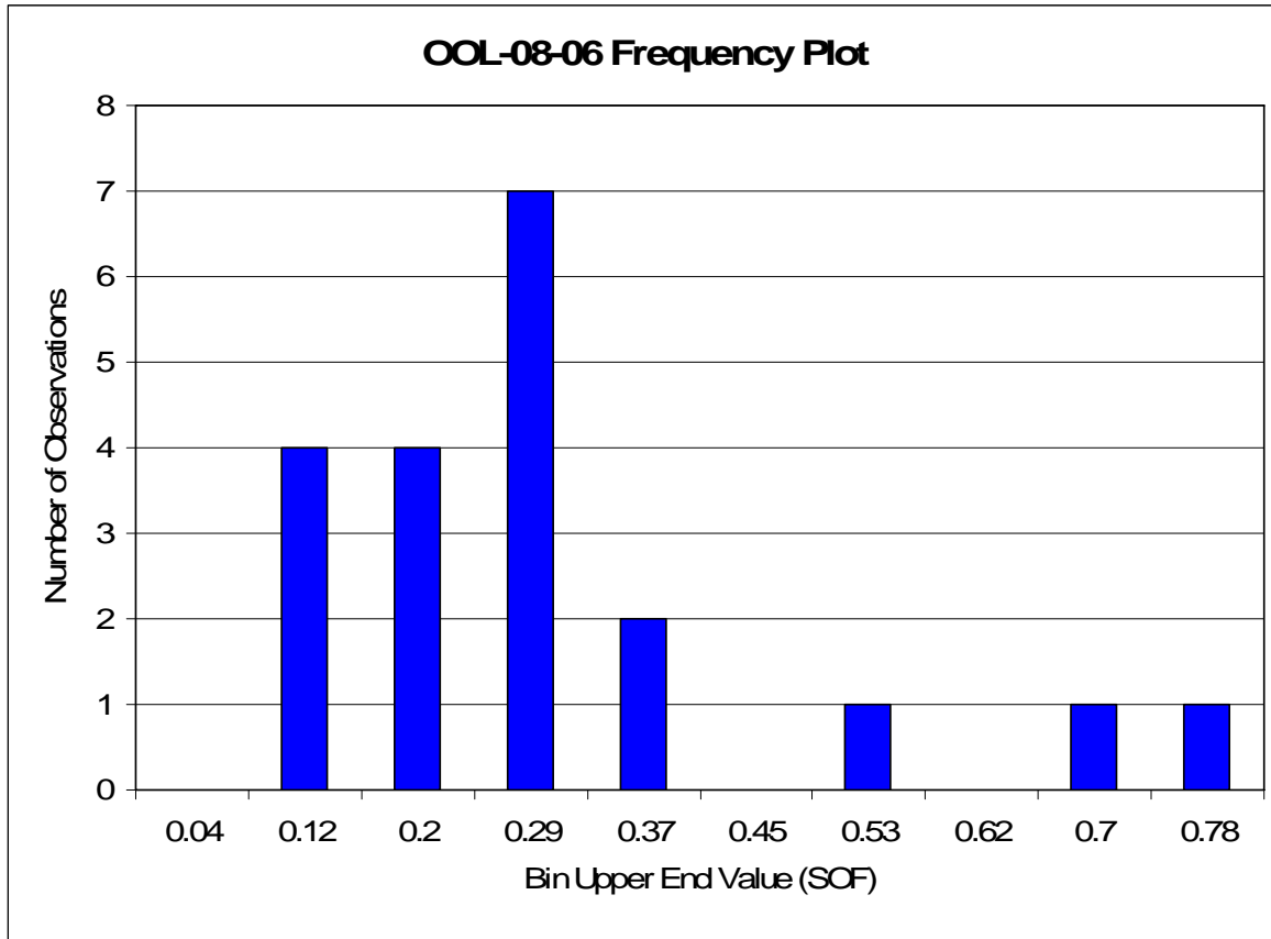
Figure 30 OOL-08-06 Sum of Fractions Frequency Plot
