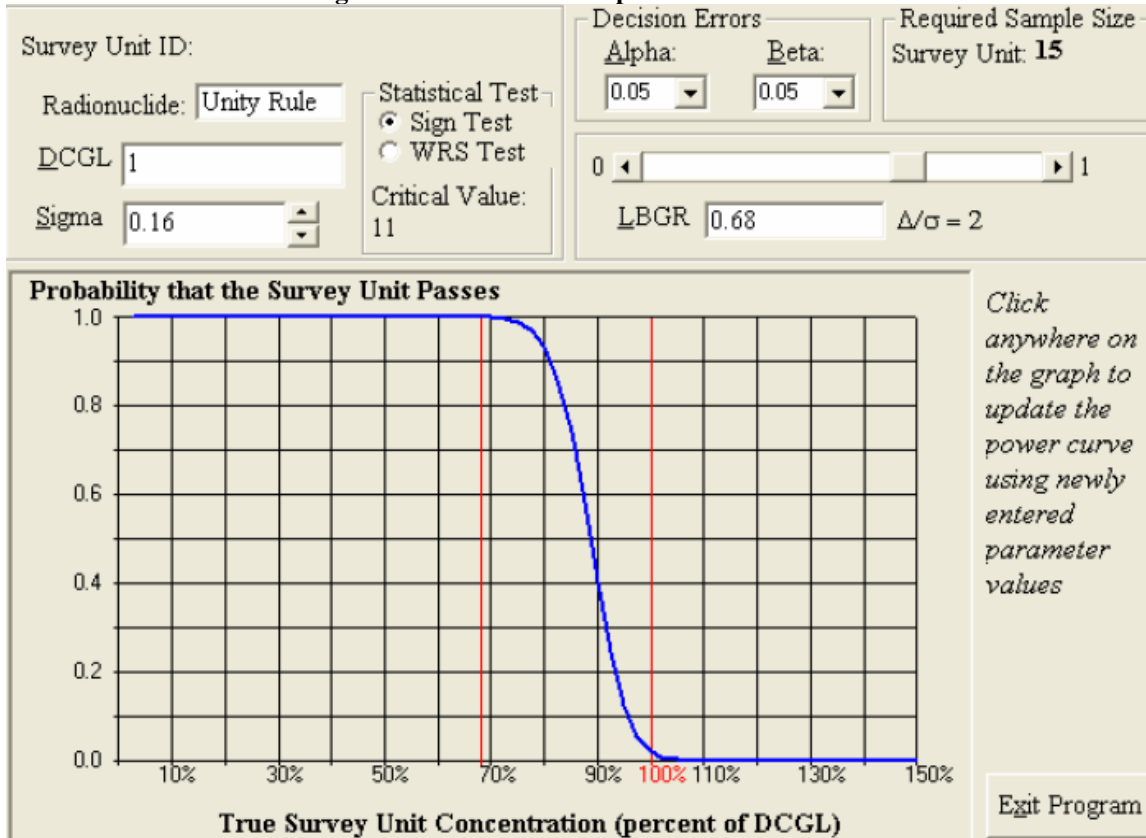
Figure 32 OOL-08-07 Retrospective Power Curve
