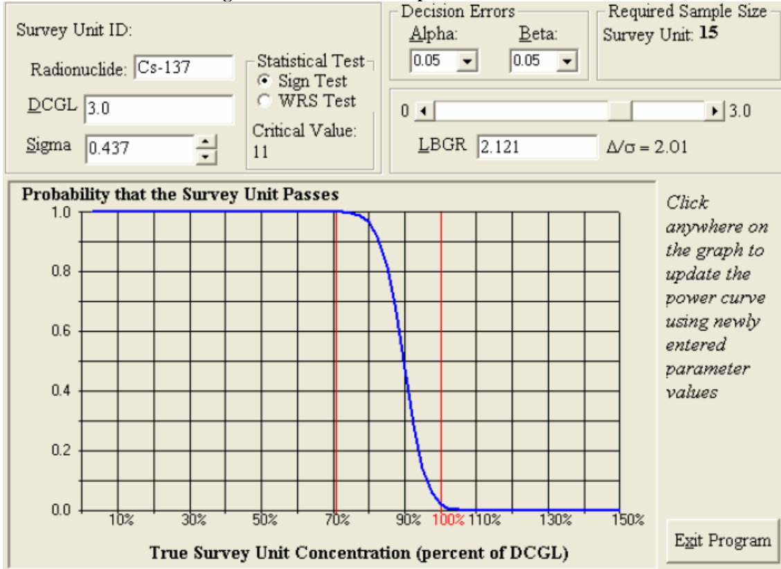
Figure 11 OOL-08-03 Prospective Power Curve
