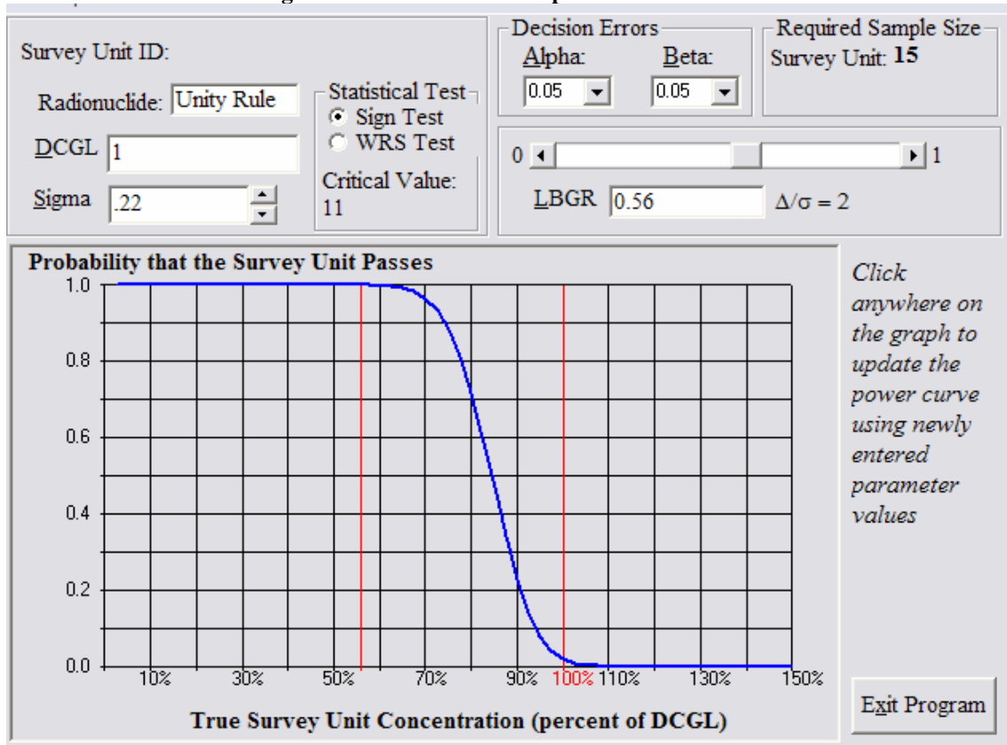
Figure 12 OOL-08-03 Retrospective Power Curve
