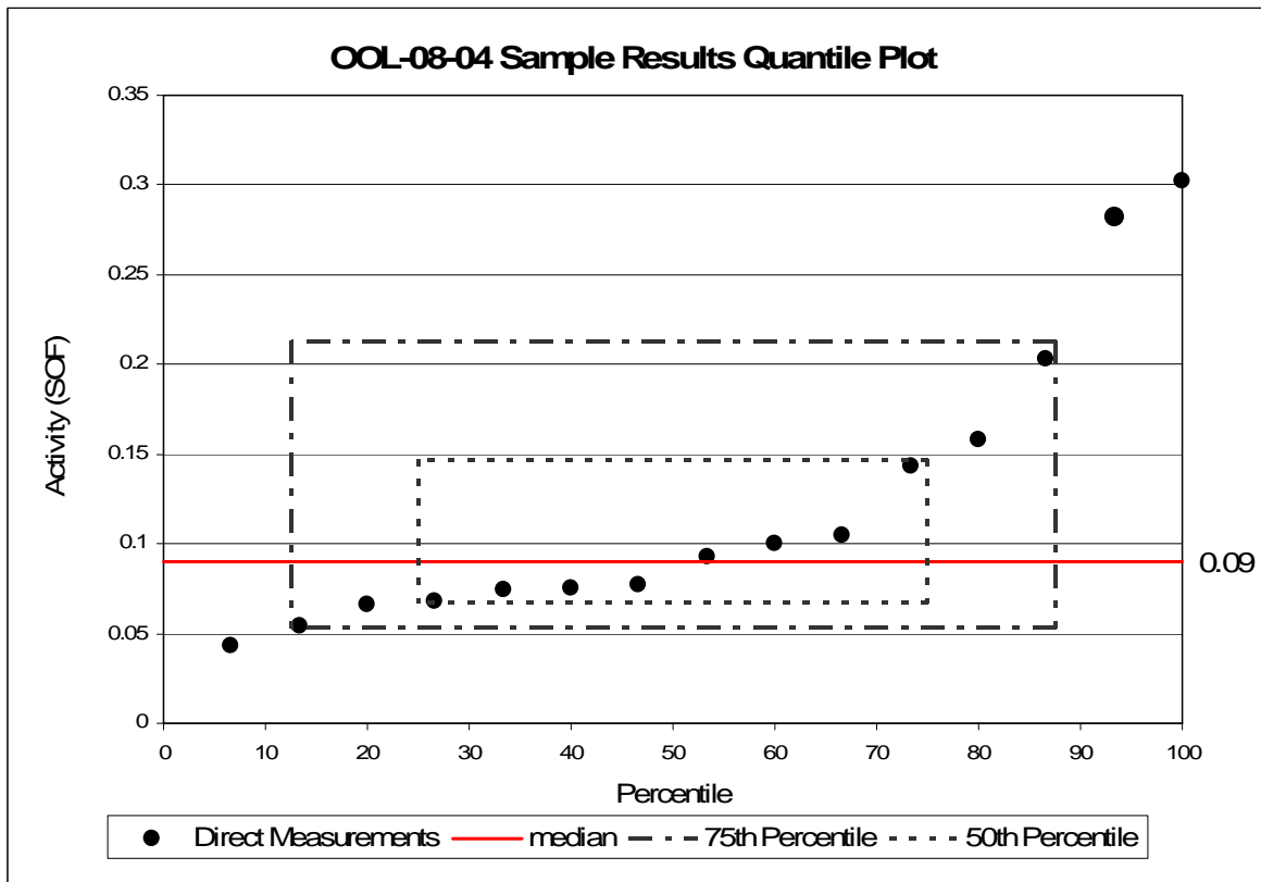
Figure 19 OOL-08-04 Sum of Fractions Quantile Plot
