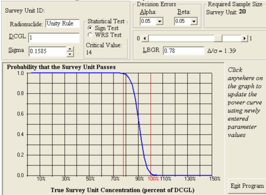
Figure 26 OOL-08-06 Prospective Power Curve
