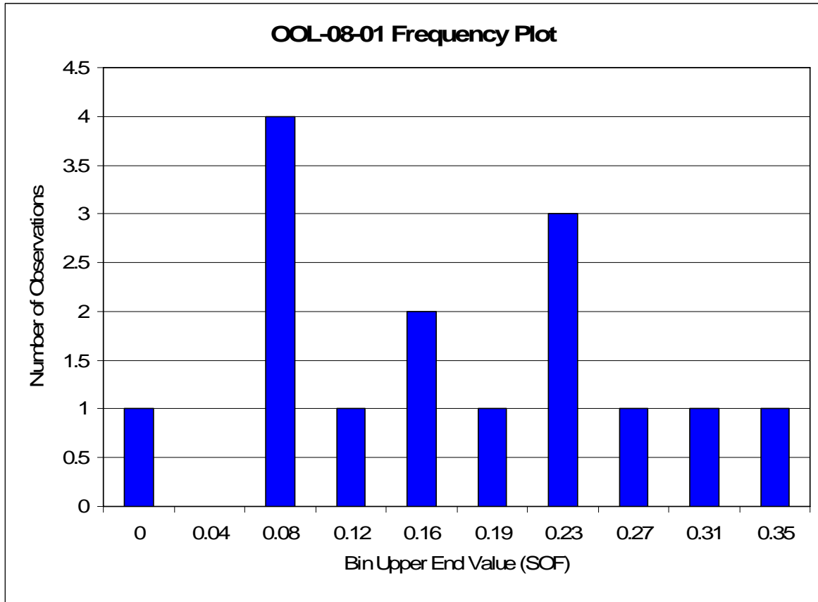
Figure 5 OOL-08-01 Sum of Fractions Frequency Plot
