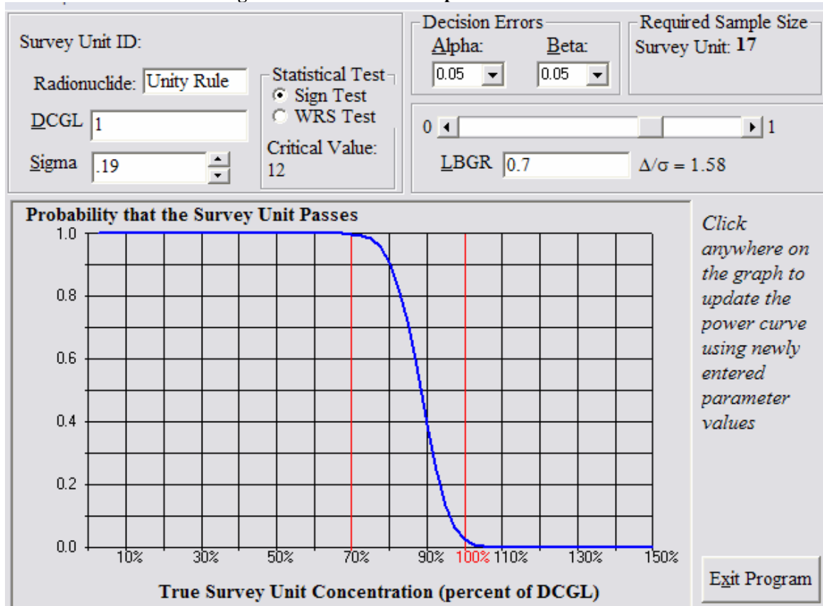
Figure 7 OOL-08-02 Retrospective Power Curve
