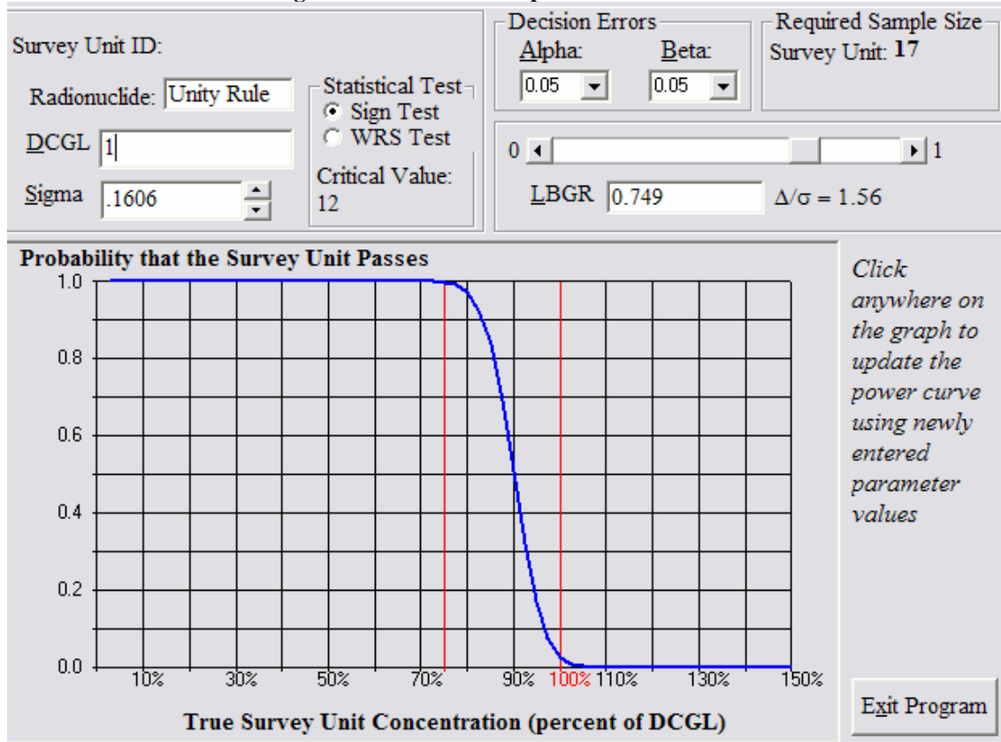
Figure 6 OOL-08-02 Prospective Power Curve
