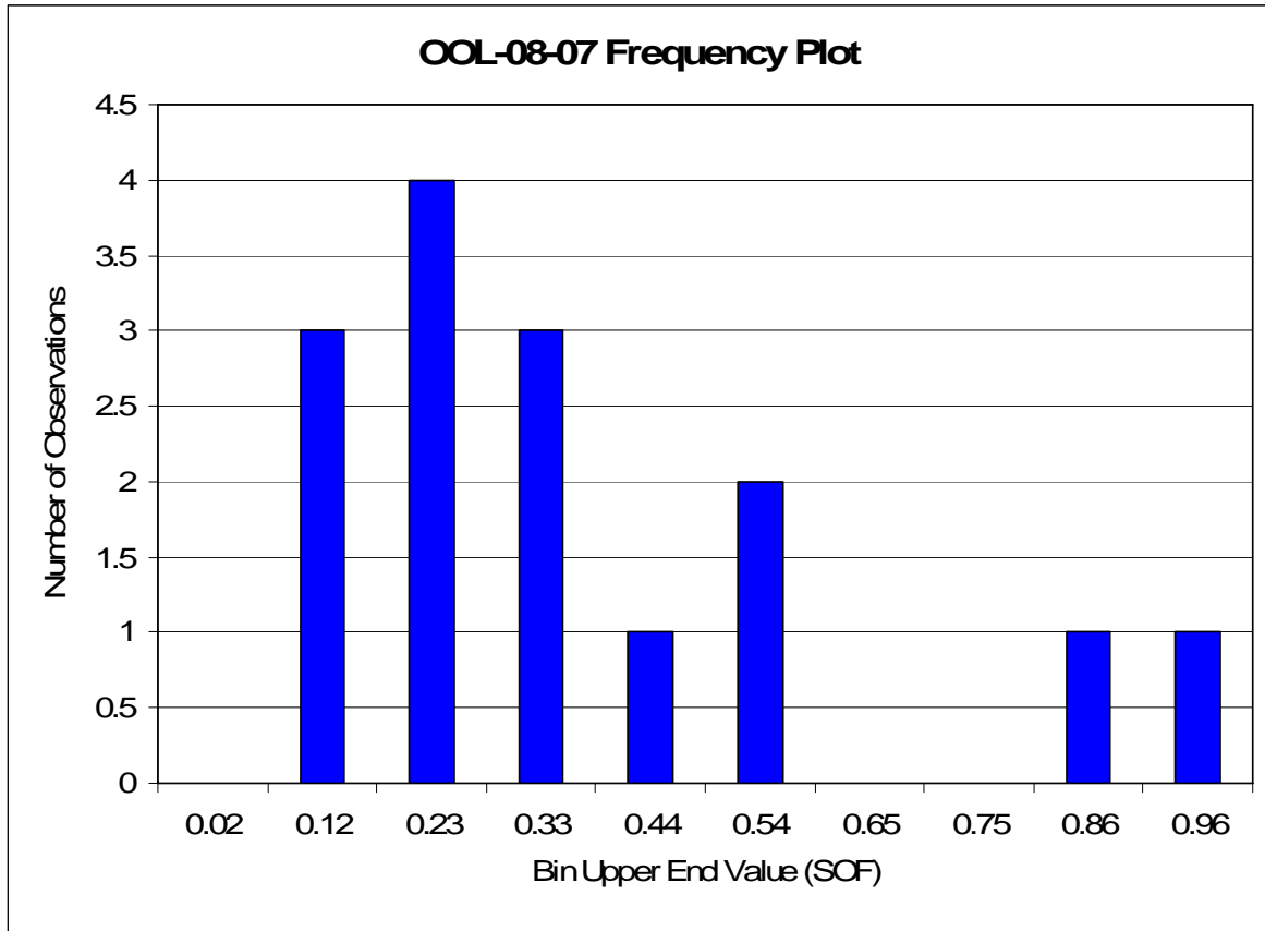
Figure 35 OOL-08-07 Sum of Fractions Frequency Plot
