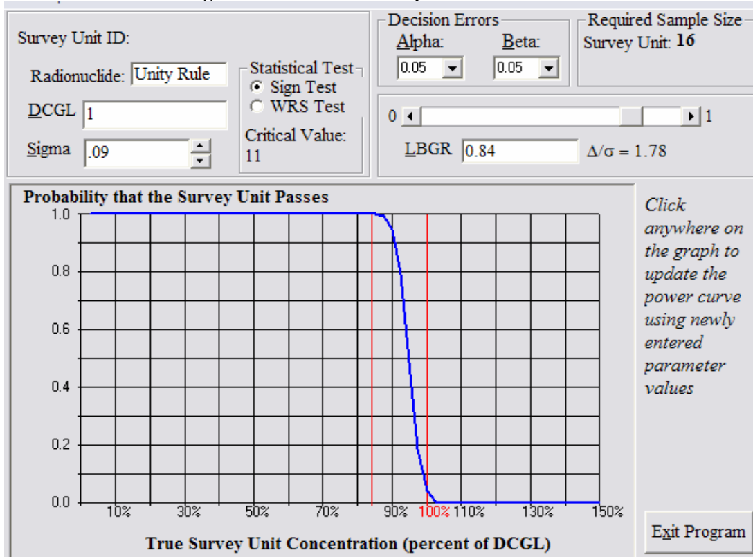
Figure 22 OOL-08-05 Retrospective Power Curve
