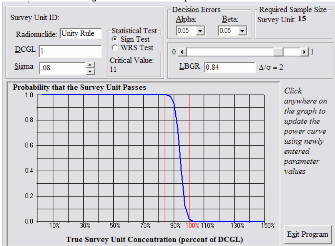
Figure 17 OOL-08-04 Retrospective Power Curve
