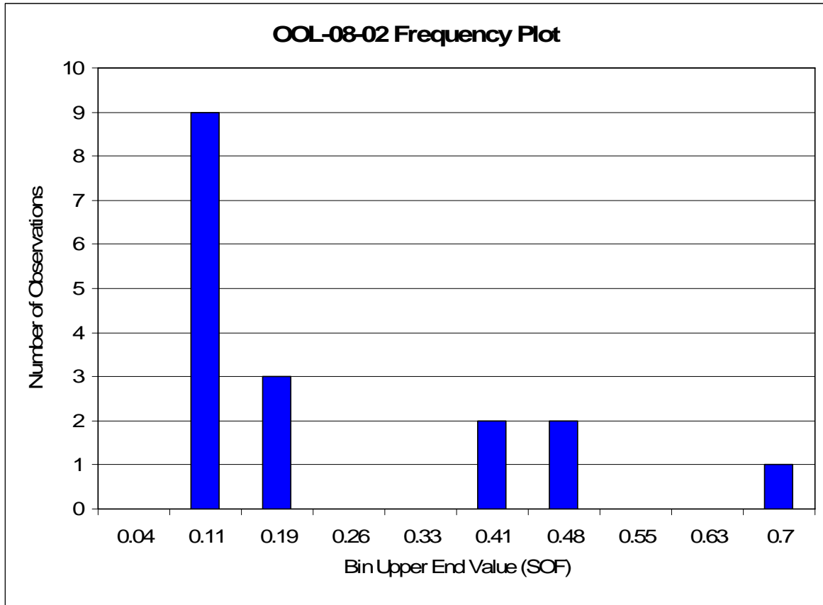
Figure 10 OOL-08-02 Sum of Fractions Frequency Plot
