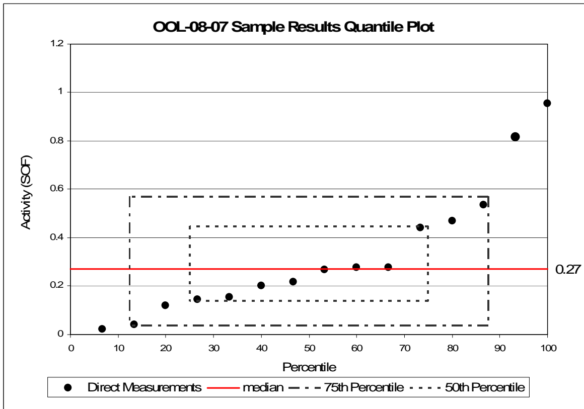
Figure 34 OOL-08-07 Sum of Fractions Quantile Plot
