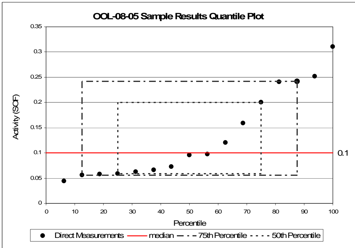
Figure 24 OOL-08-05 Sum of Fractions Quantile Plot
