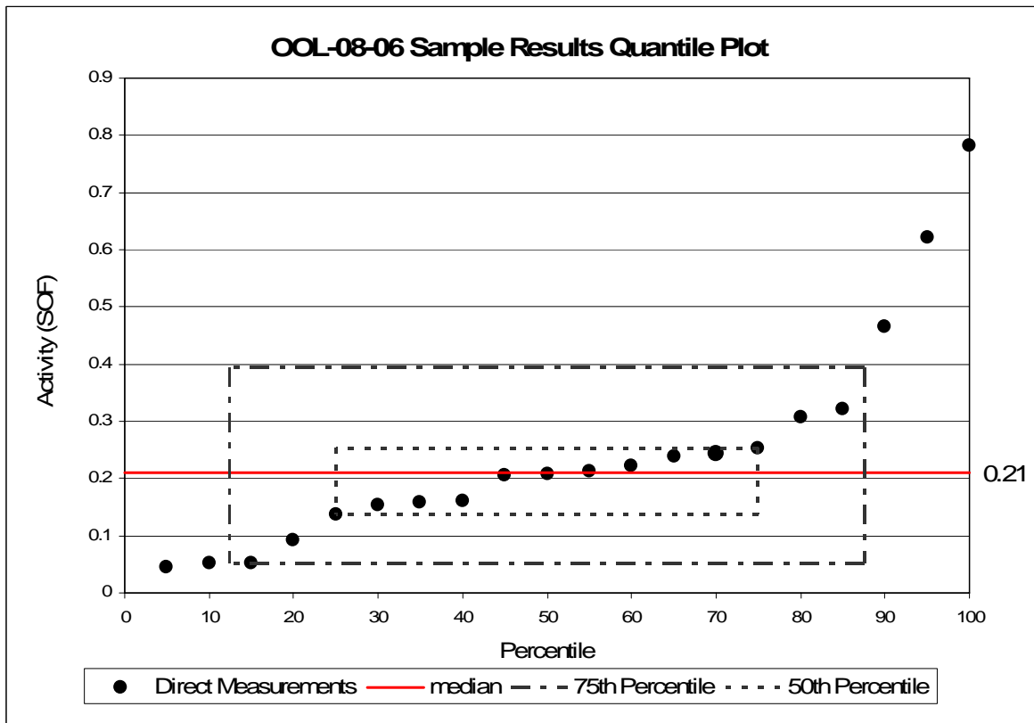
Figure 29 OOL-08-06 Sum of Fractions Quantile Plot
