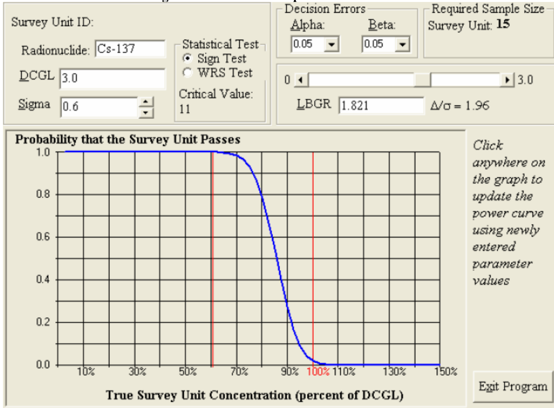
Figure 2 OOL-08-01 Retrospective Power Curve
