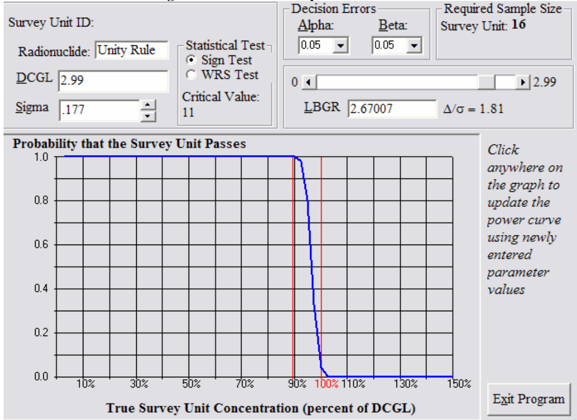
Figure 21 OOL-08-05 Prospective Power Curve
