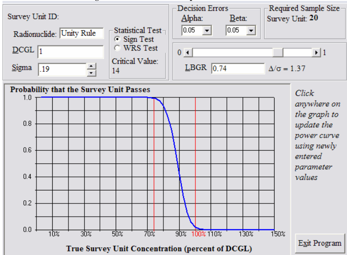
Figure 27 OOL-08-06 Retrospective Power Curve
