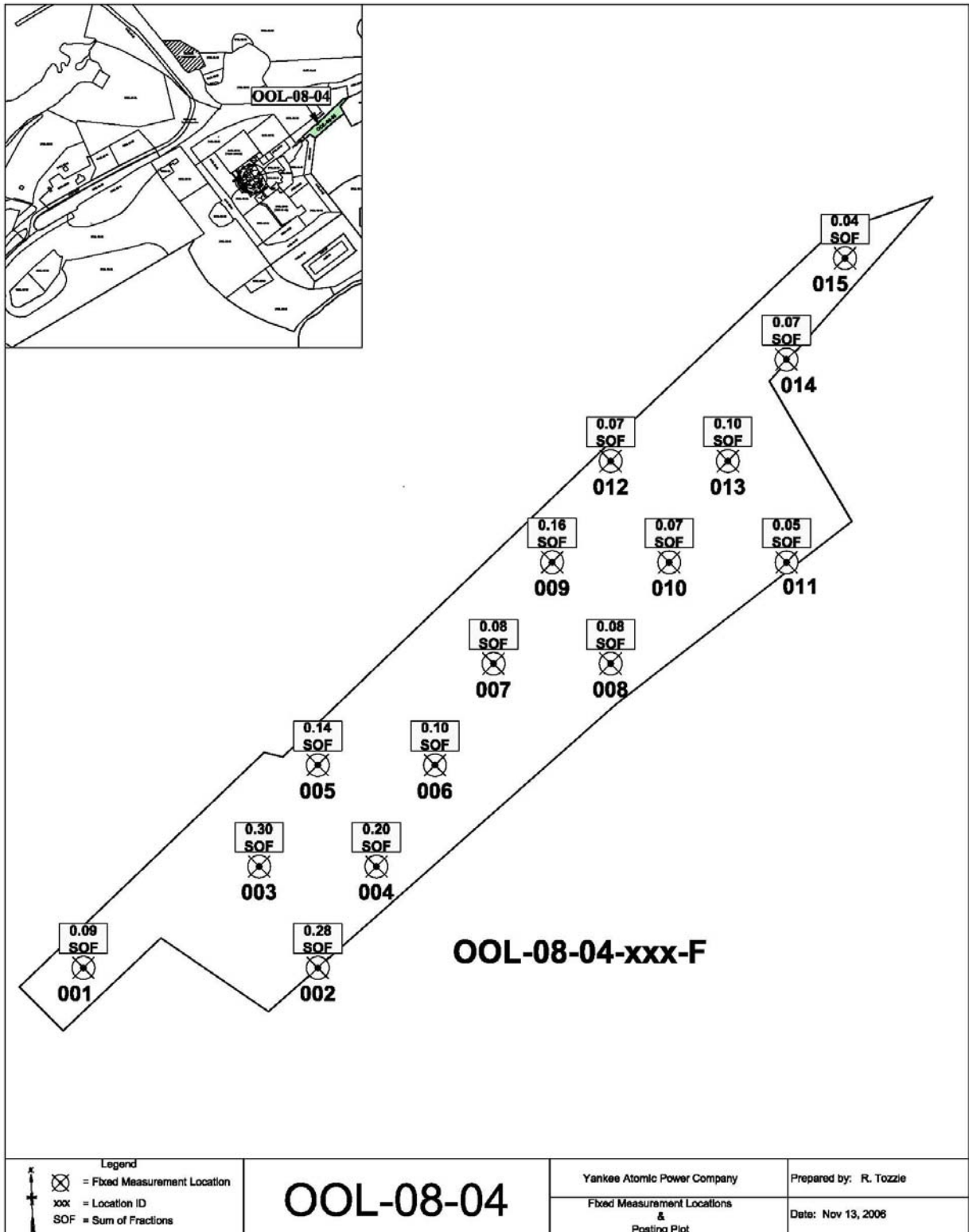
Figure 5 OOL-08-04 Posting Plot
