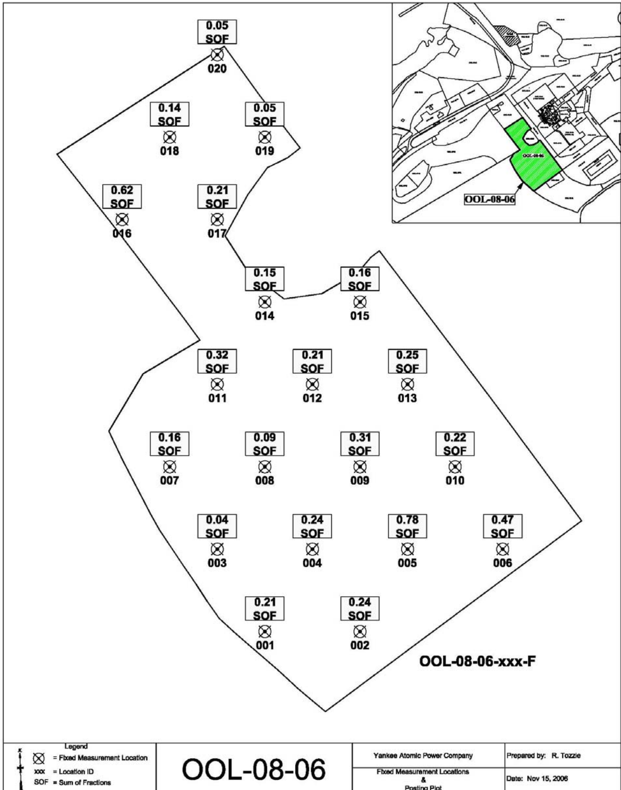
Figure 7 OOL-08-06 Posting Plot
