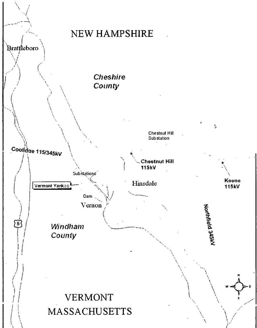
Figure 3-2 Chestnut Hill 115-Kv Transmission Line
