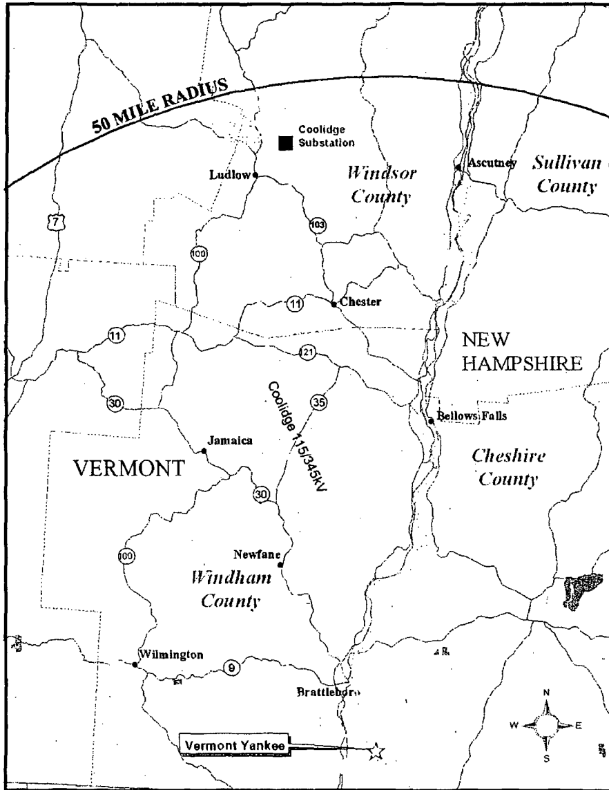
Figure 3-3 Coolidge 115/345-Kv Transmission Line
