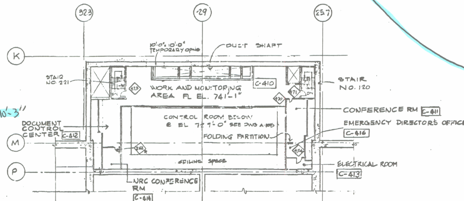
PLAN - TECHNICAL SUPPORT CENTER @ EL 741'-1" NOTE: SEE DWG A-105 FOR LARGE SCALE PLAN
