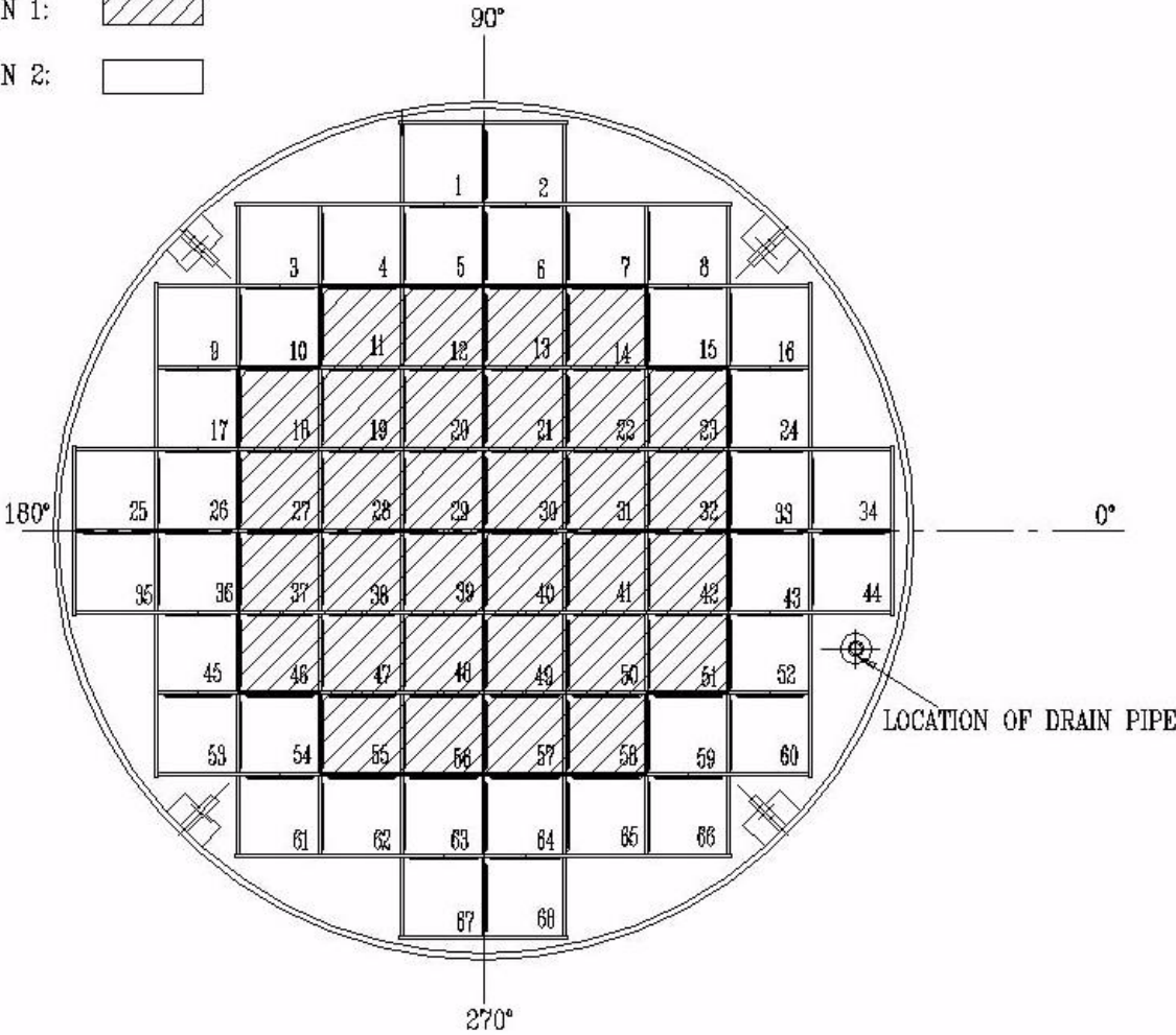
Figure 2.1-4 Fuel Loading Regions - MPC-68/68FF
