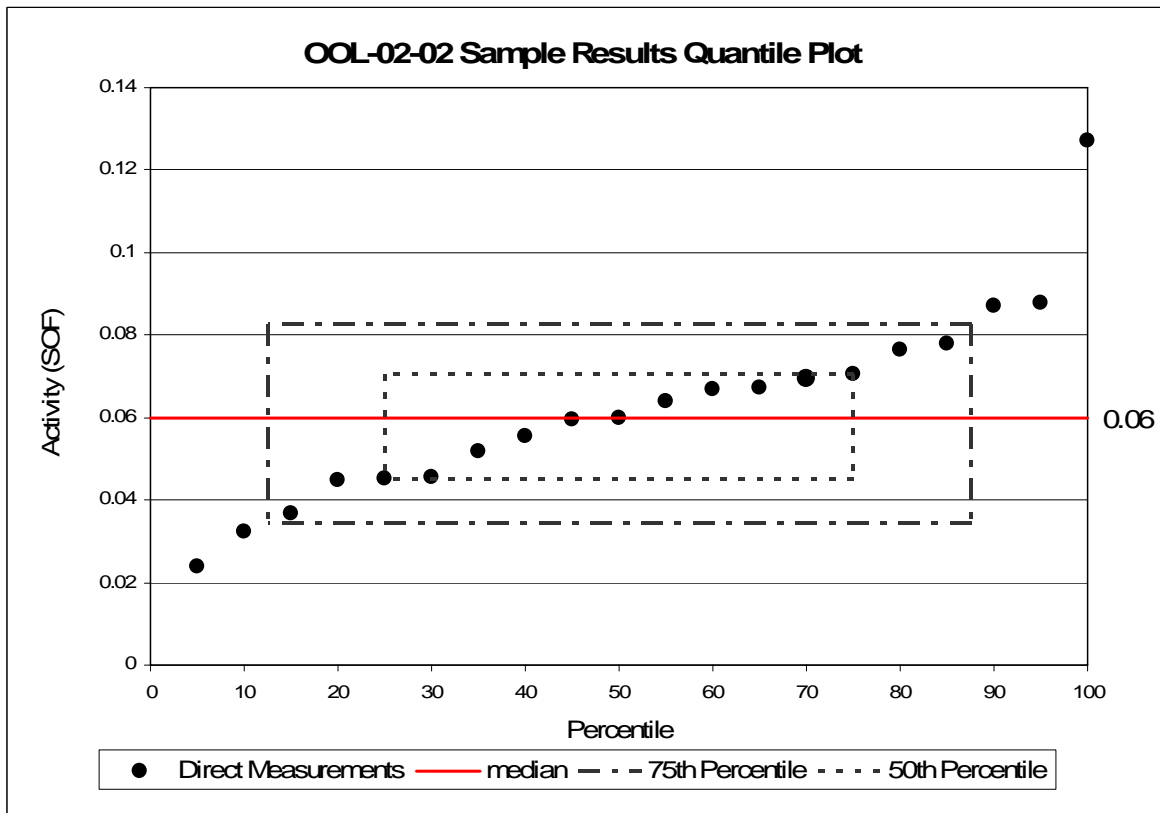
Figure 9 OOL-02-02 Sum of Fractions Quantile Plot
