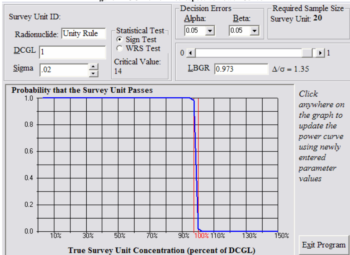
Figure 17 OOL-02-04 Retrospective Power Curve
