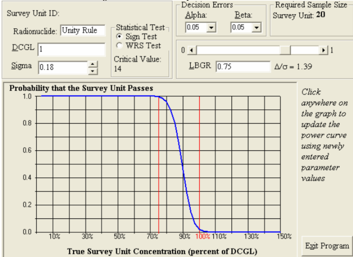
Figure 6 OOL-02-02 Prospective Power Curve
