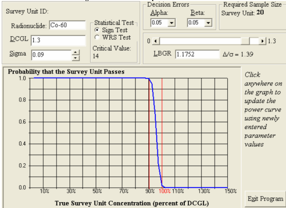
Figure 2 OOL-02-01 Retrospective Power Curve
