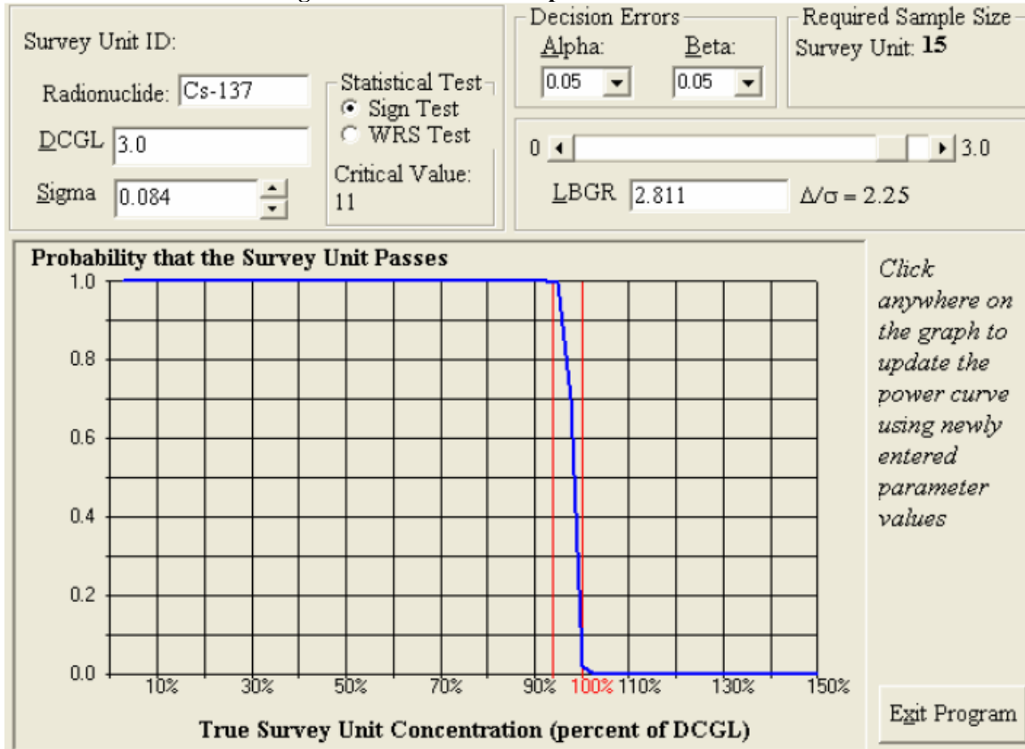
Figure 16 OOL-02-04 Prospective Power Curve
