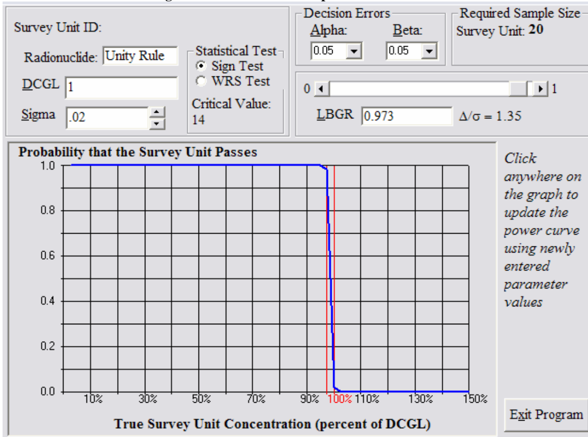
Figure 22 OOL-02-05 Retrospective Power Curve
