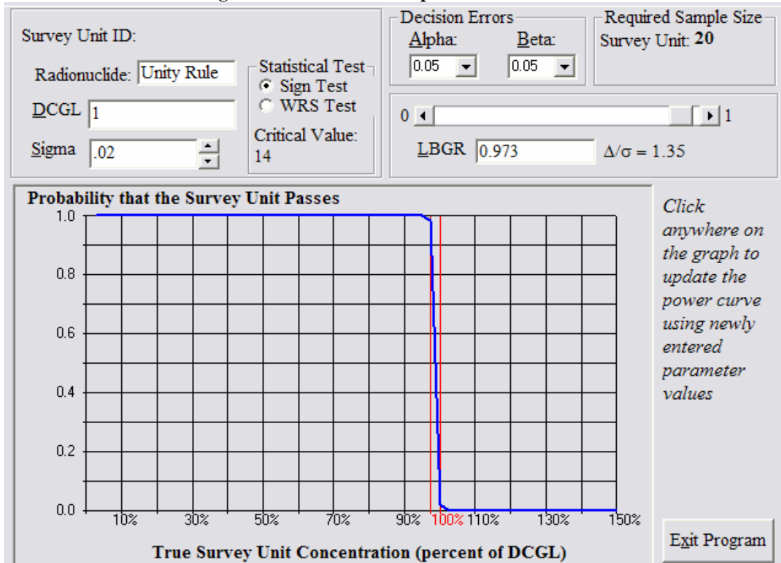
Figure 7 OOL-02-02 Retrospective Power Curve
