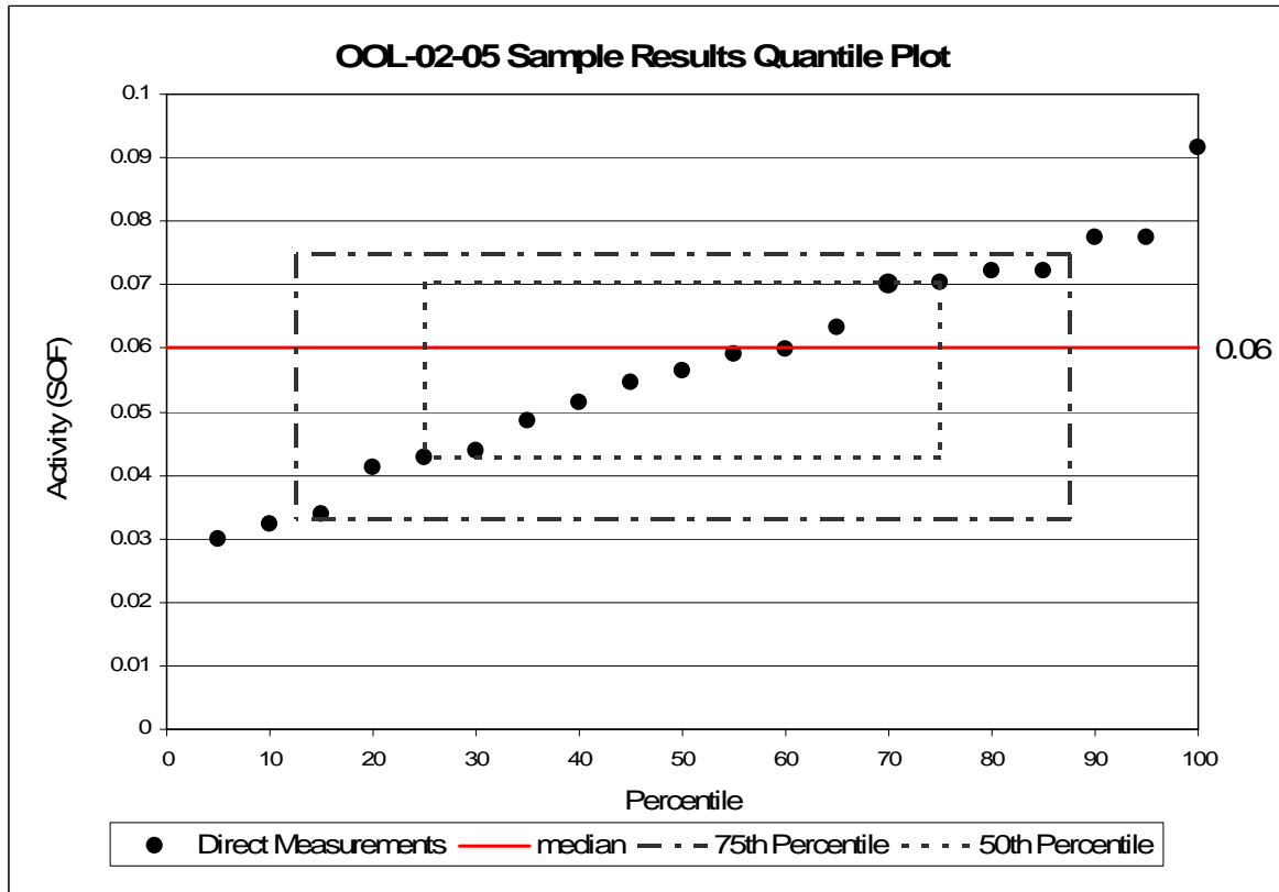
Figure 24 OOL-02-05 Sum of Fractions Quantile Plot
