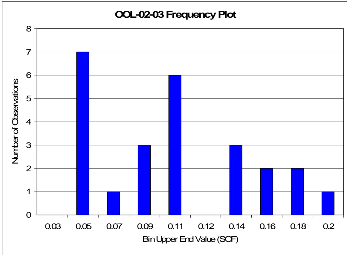
Figure 15 OOL-02-03 Sum of Fractions Frequency Plot
