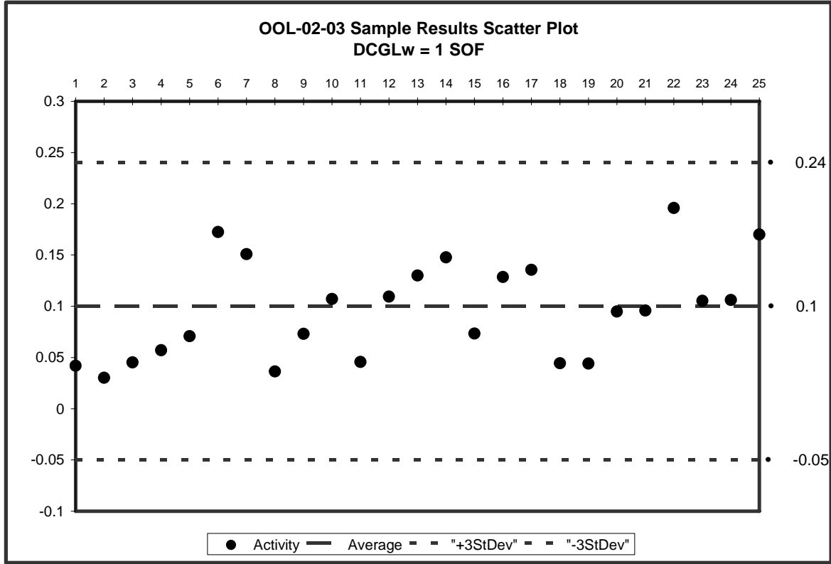
Figure 13 OOL-02-03 Sum of Fractions Scatter Plot
