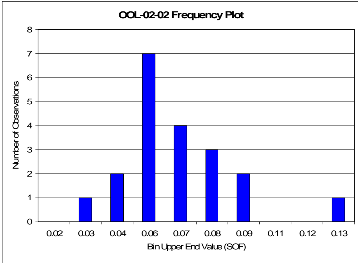
Figure 10 OOL-02-02 Sum of Fractions Frequency Plot
