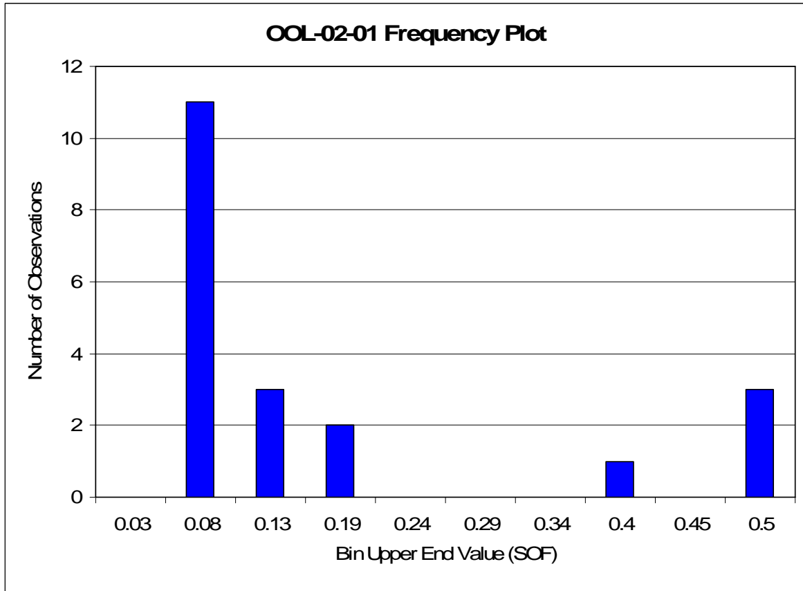
Figure 5 OOL-02-01 Sum of Fractions Frequency Plot
