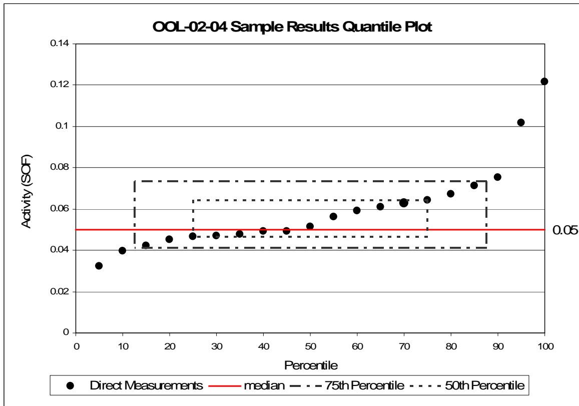
Figure 19 OOL-02-04 Sum of Fractions Quantile Plot
