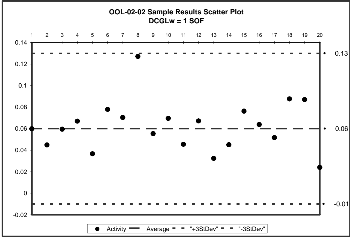
Figure 8 OOL-02-02 Sum of Fractions Scatter Plot
