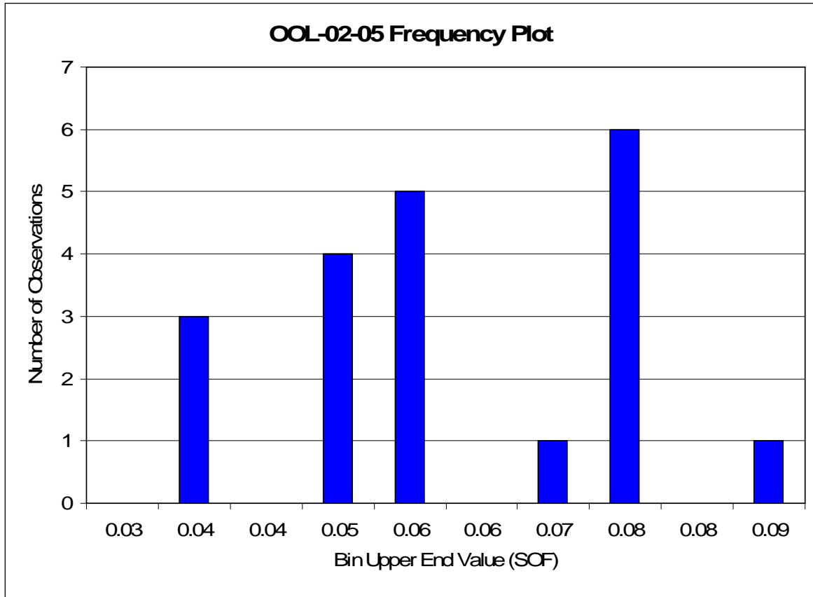
Figure 25 OOL-02-05 Sum of Fractions Frequency Plot
