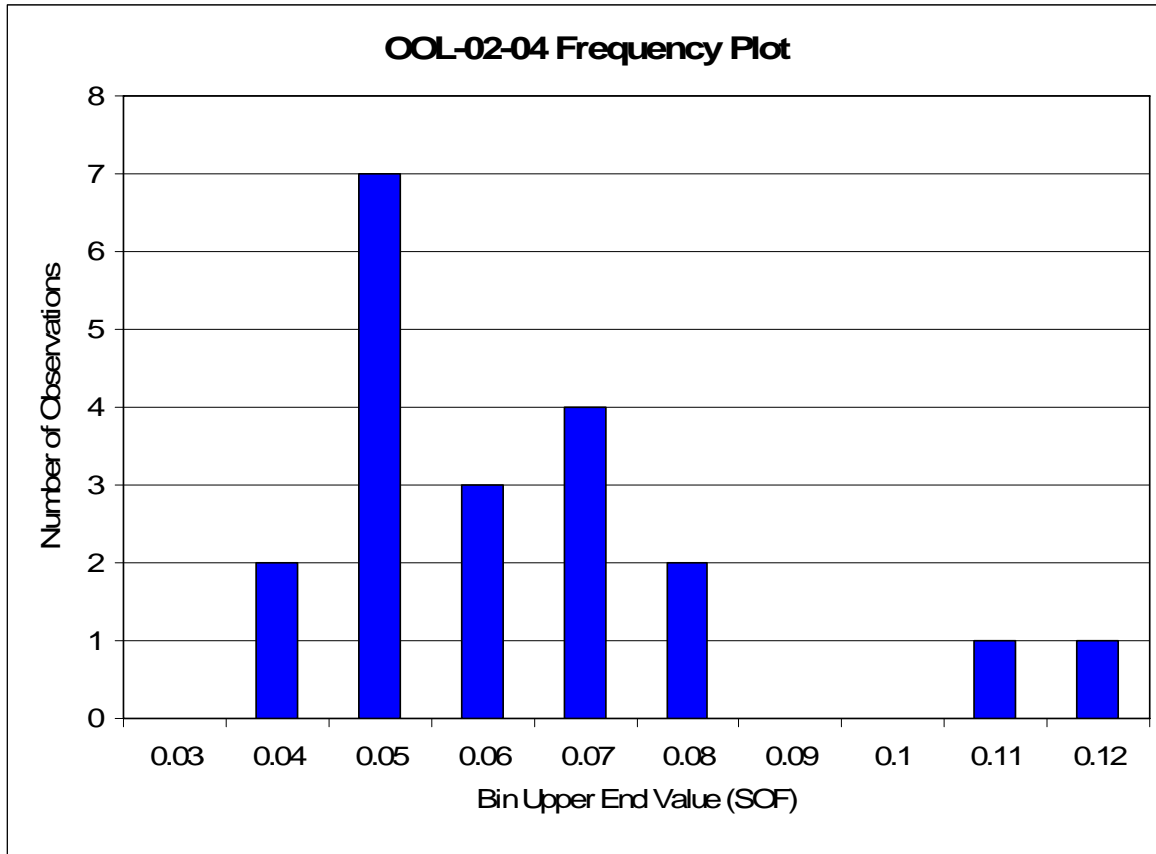
Figure 20 OOL-02-04 Sum of Fractions Frequency Plot
