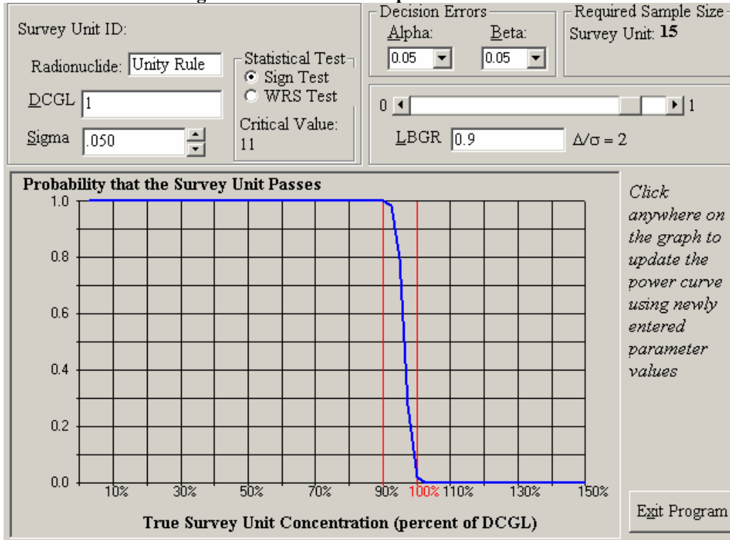
Figure 12 OOL-02-03 Retrospective Power Curve
