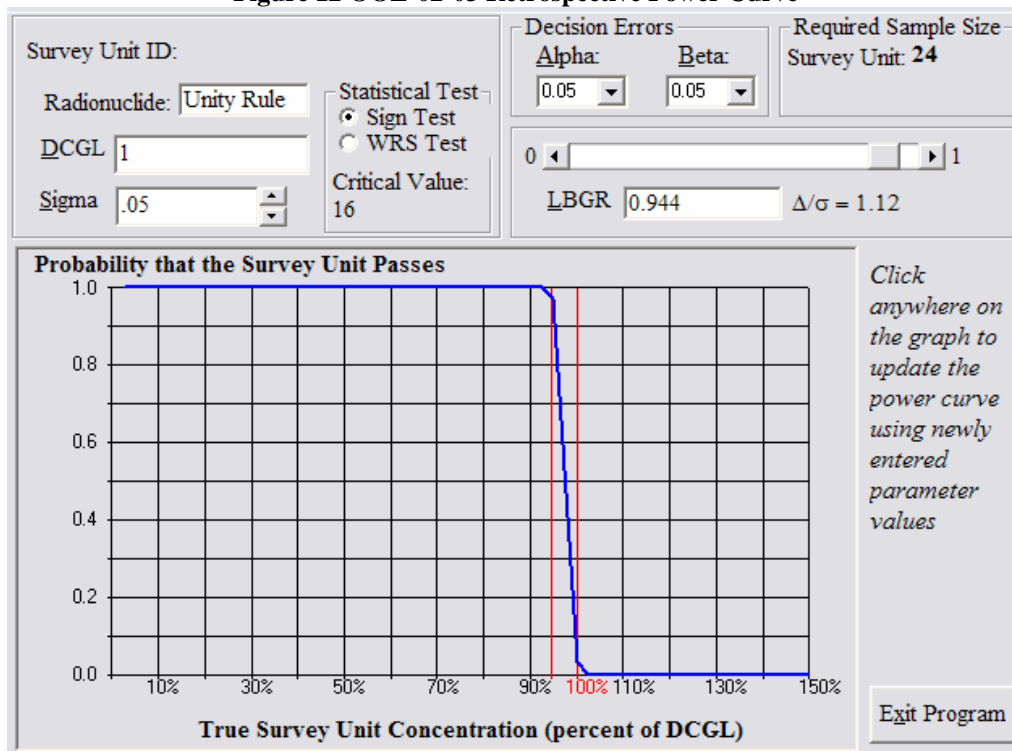
Figure 12 OOL-02-03 Retrospective Power Curve
