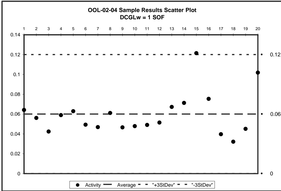
Figure 18 OOL-02-04 Sum of Fractions Scatter Plot
