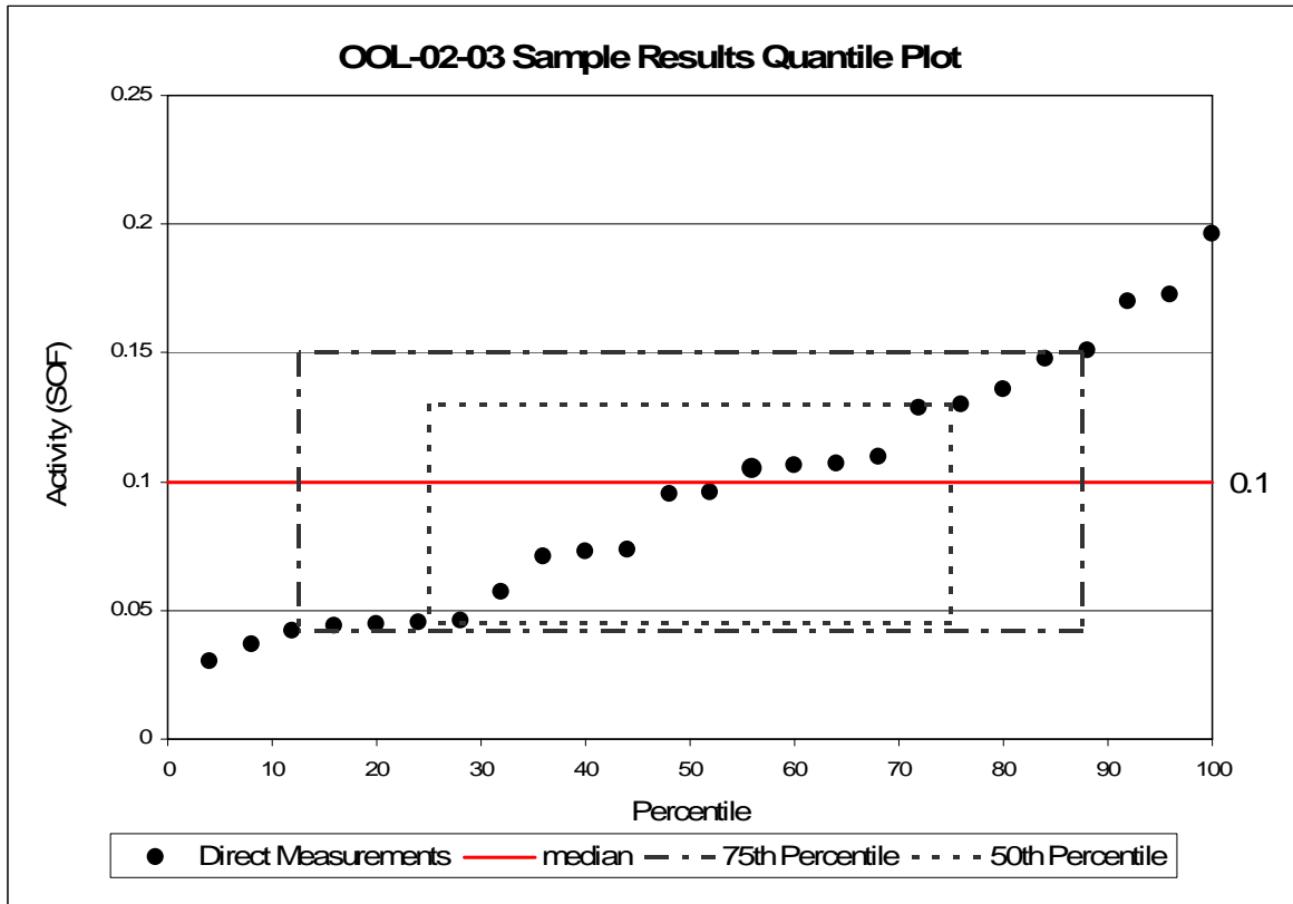
Figure 14 OOL-02-03 Sum of Fractions Quantile Plot
