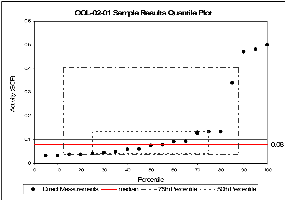
Figure 4 OOL-02-01 Sum of Fractions Quantile Plot
