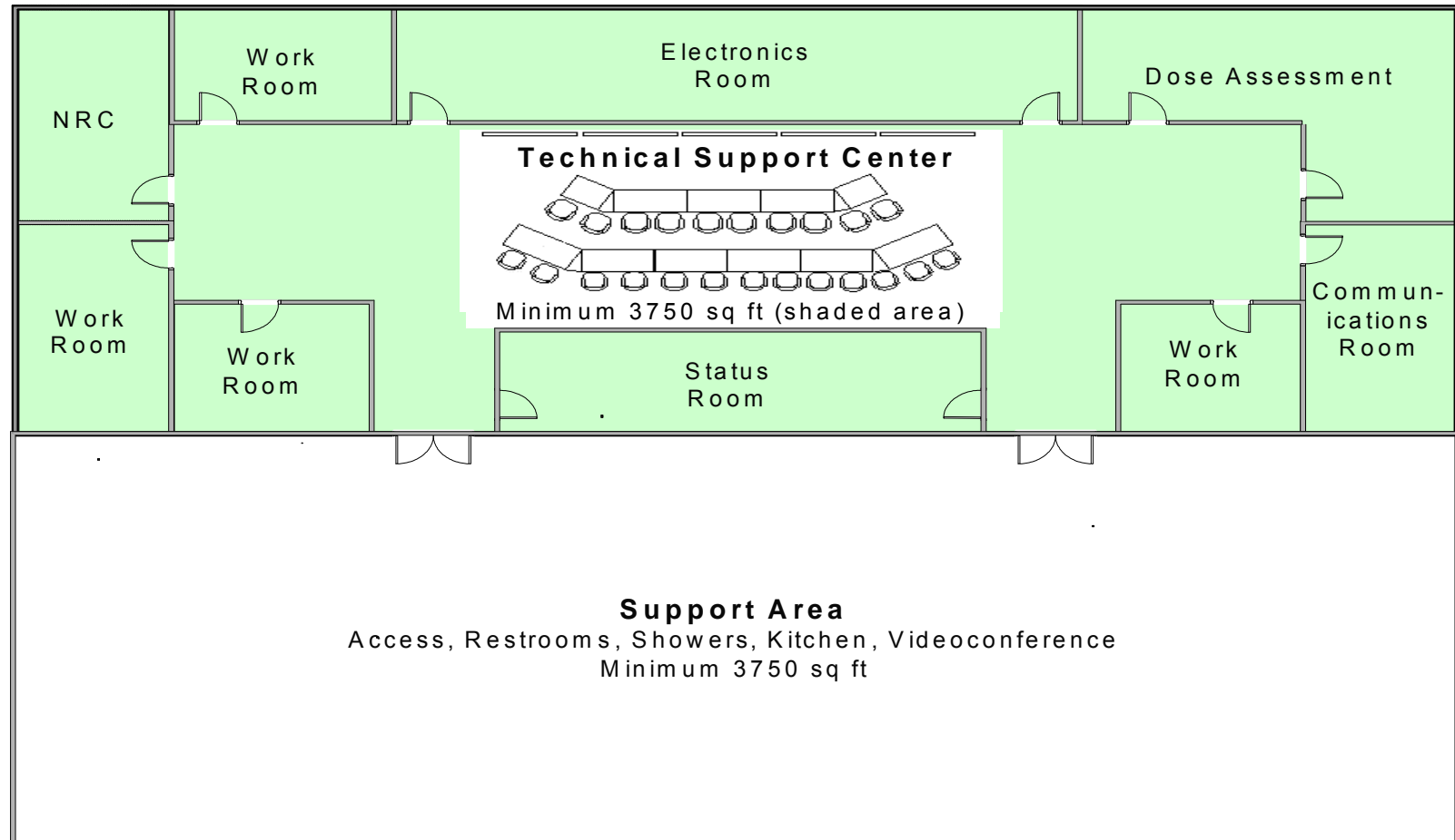
Figure H-1 VEGP TSC Layout
