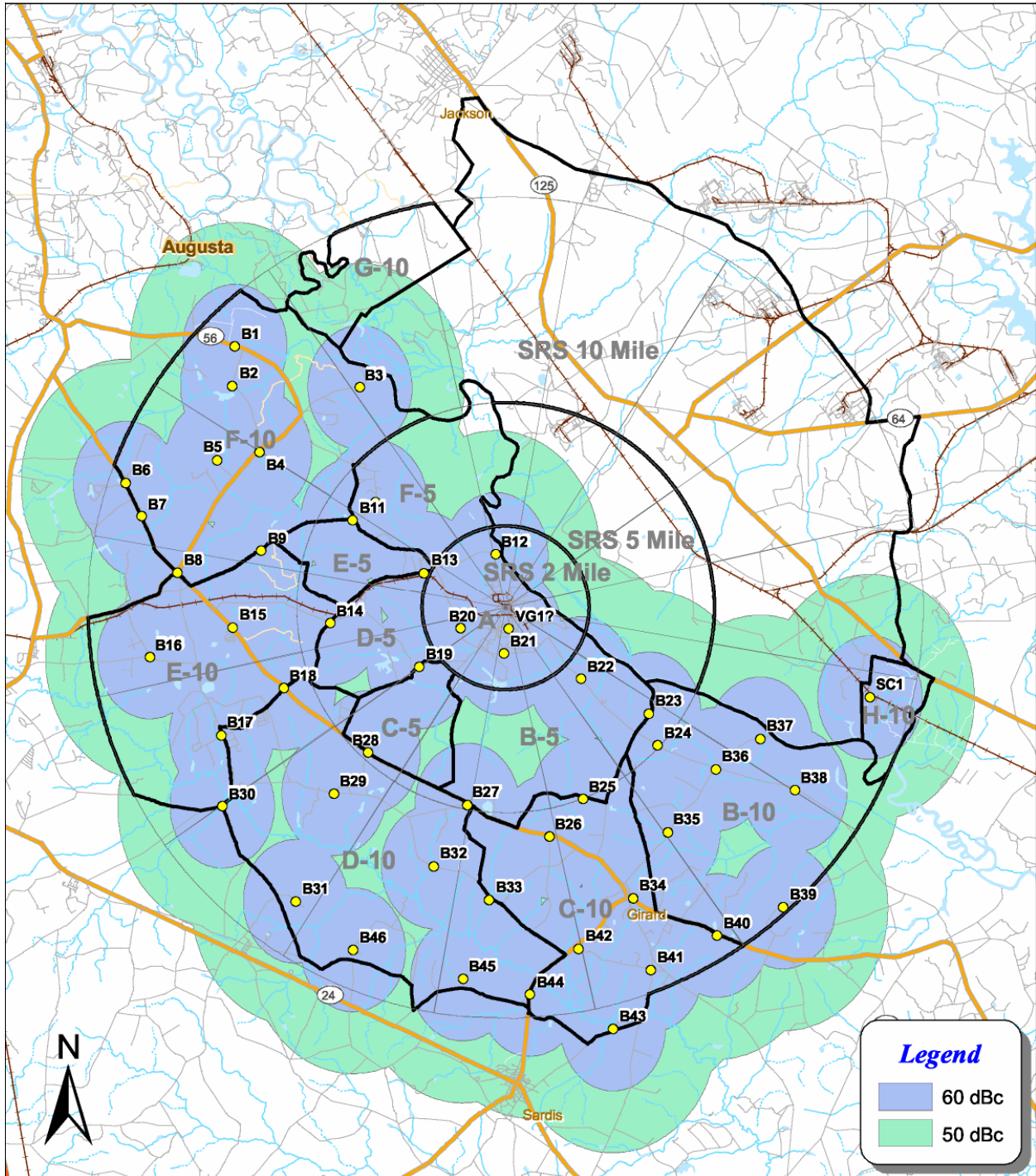
Figure A3-1 60 and 50 dBc Design Coverage Contours
