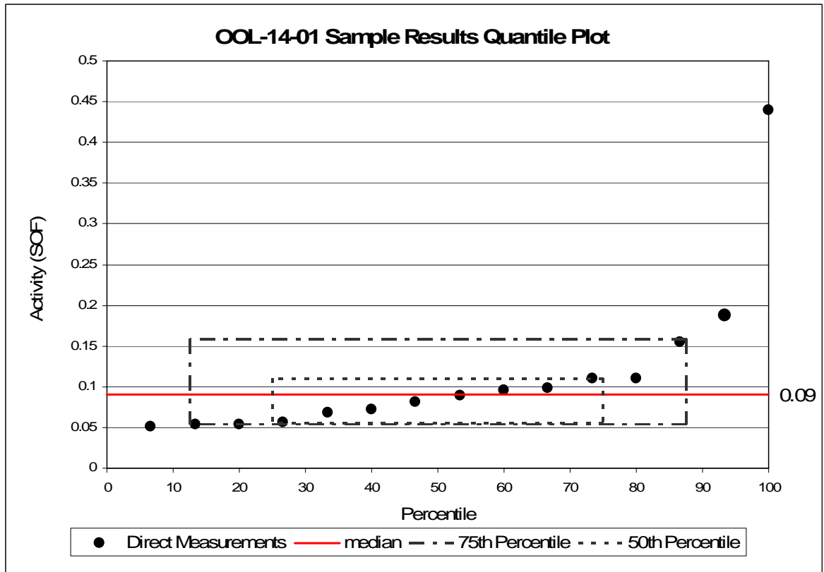
Figure 4 OOL-14-01 Sum of Fractions Quantile Plot
