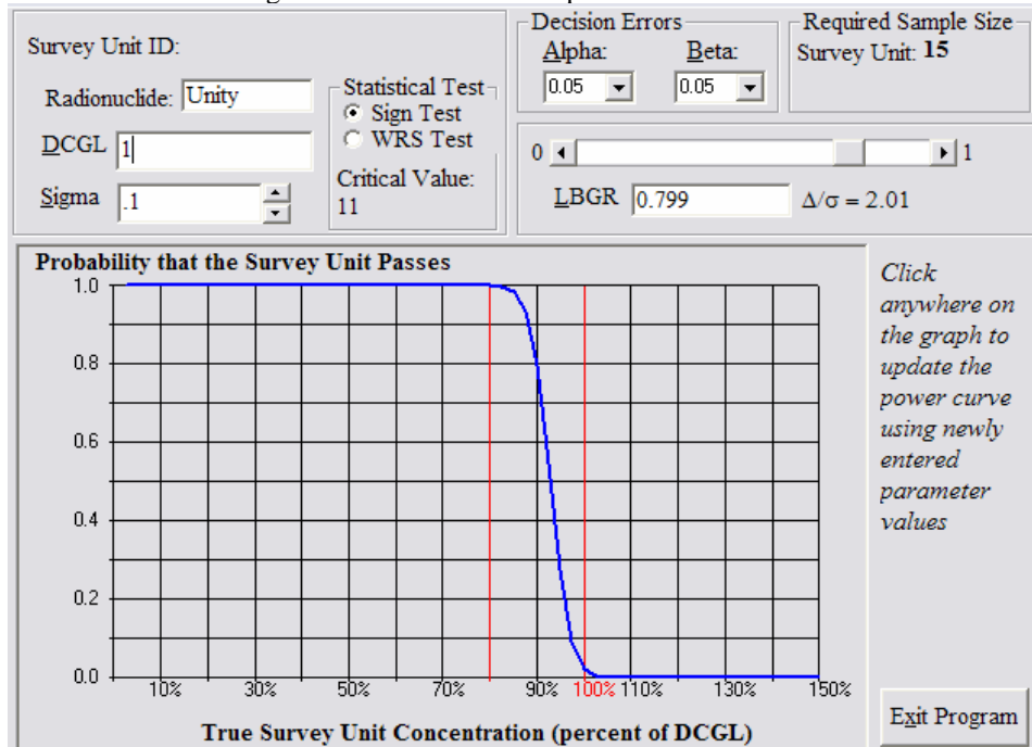
Figure 2 OOL-14-01 Retrospective Power Curve
