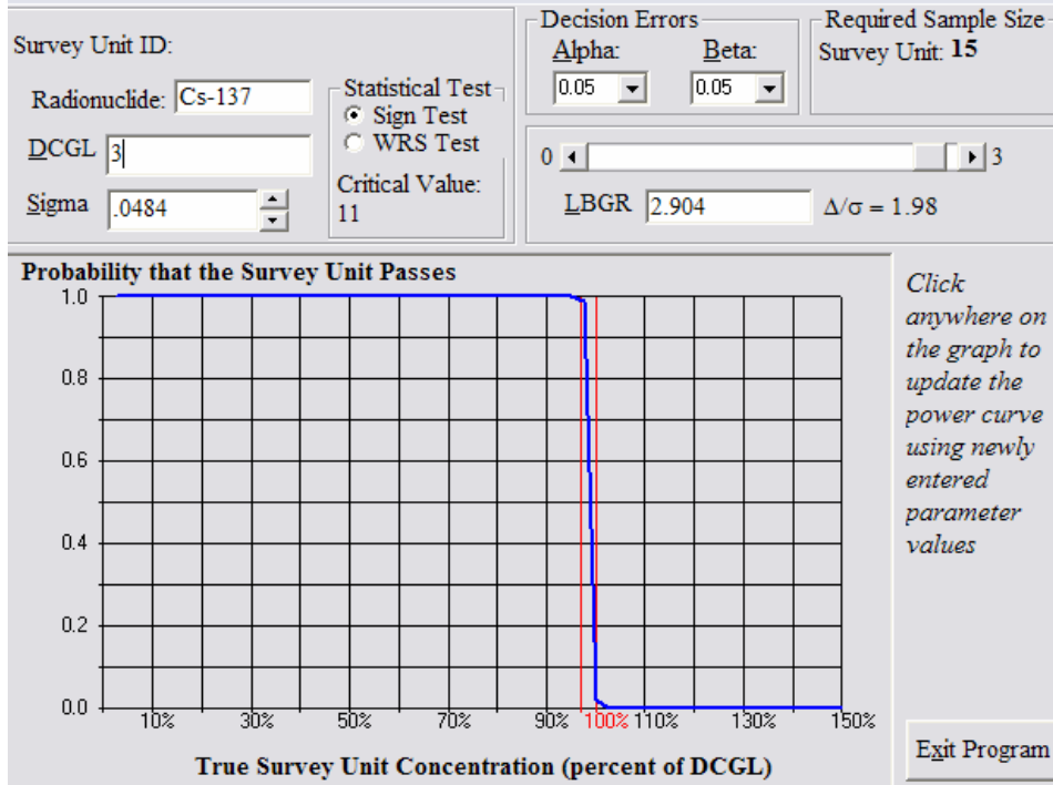
Figure 1 OOL-14-01 Prospective Power Curve
