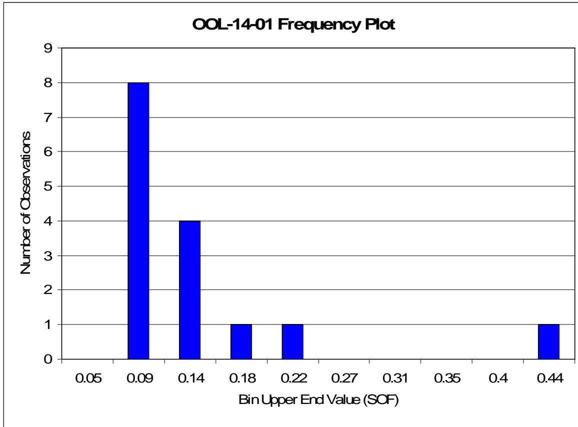
Figure 5 OOL-14-01 Sum of Fractions Frequency Plot
