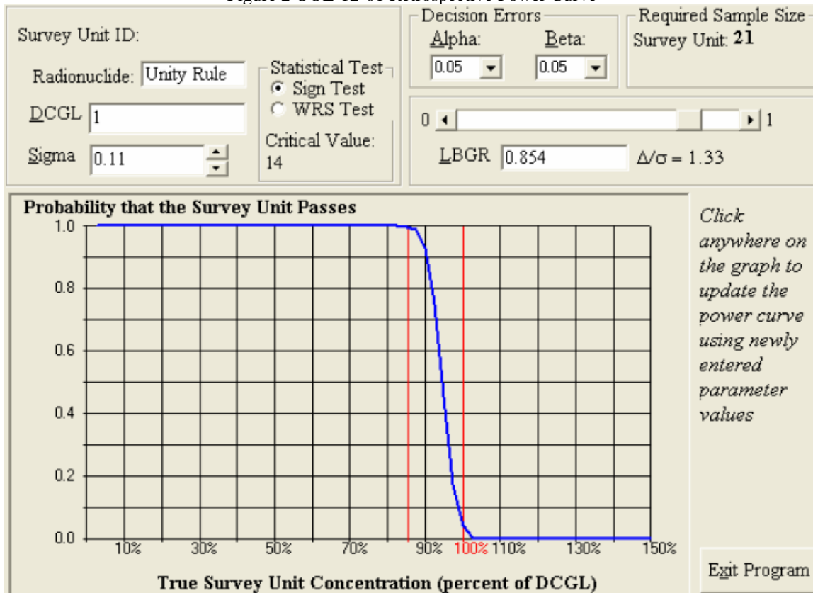
Figure 2 OOL-12-01 Retrospective Power Curve
