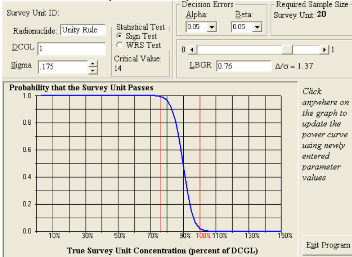
Figure 1 OOL-12-01 Prospective Power Curve
