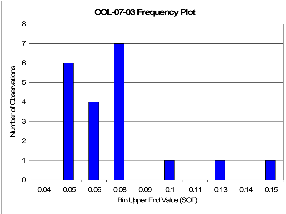
Figure 15 OOL-07-03 Sum of Fractions Frequency Plot
