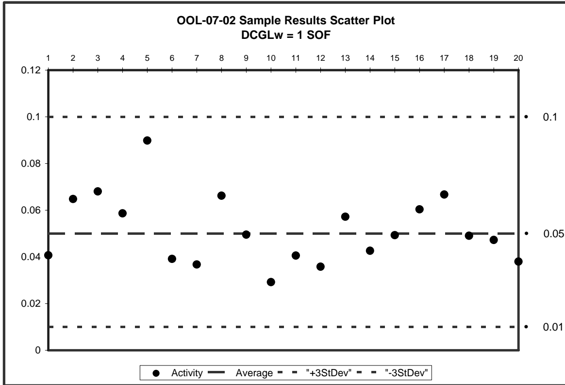
Figure 8 OOL-07-02 Sum of Fractions Scatter Plot
