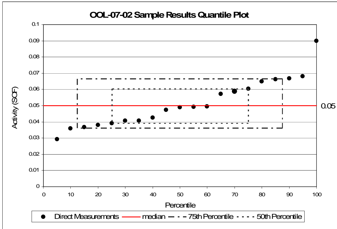
Figure 9 OOL-07-02 Sum of Fractions Quantile Plot
