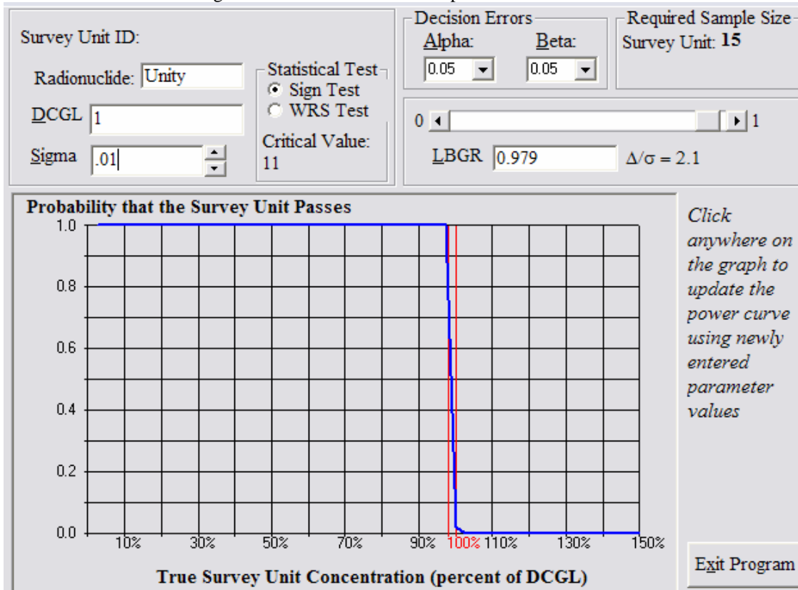
Figure 7 OOL-07-02 SOF Retrospective Power Curve
