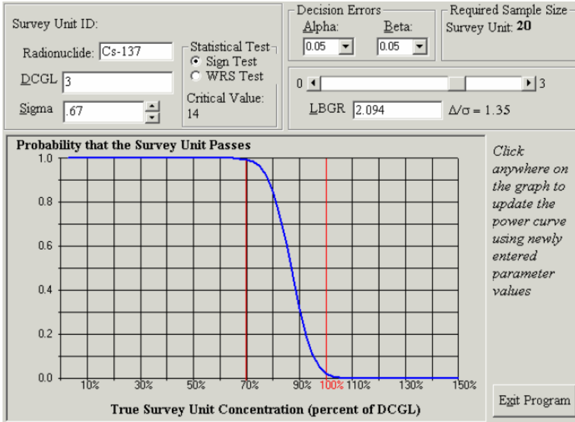
Figure 12 OOL-07-03 SOF Retrospective Power Curve
