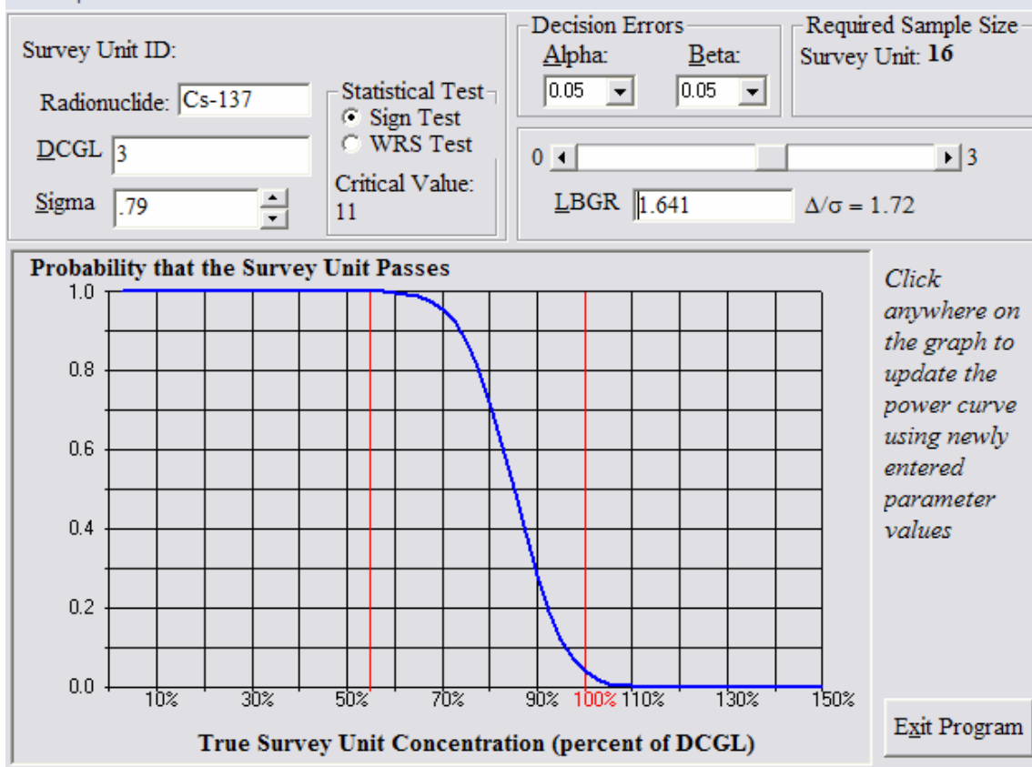
Figure 1 OOL-07-01 Cs-137 Prospective Power Curve
