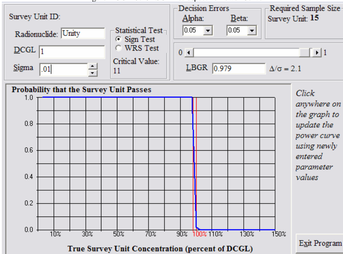
Figure 2 OOL-07-01 SOF Retrospective Power Curve
