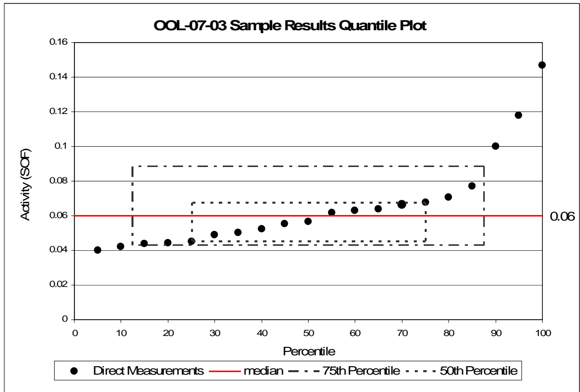
Figure 14 OOL-07-03 Sum of Fractions Quantile Plot
