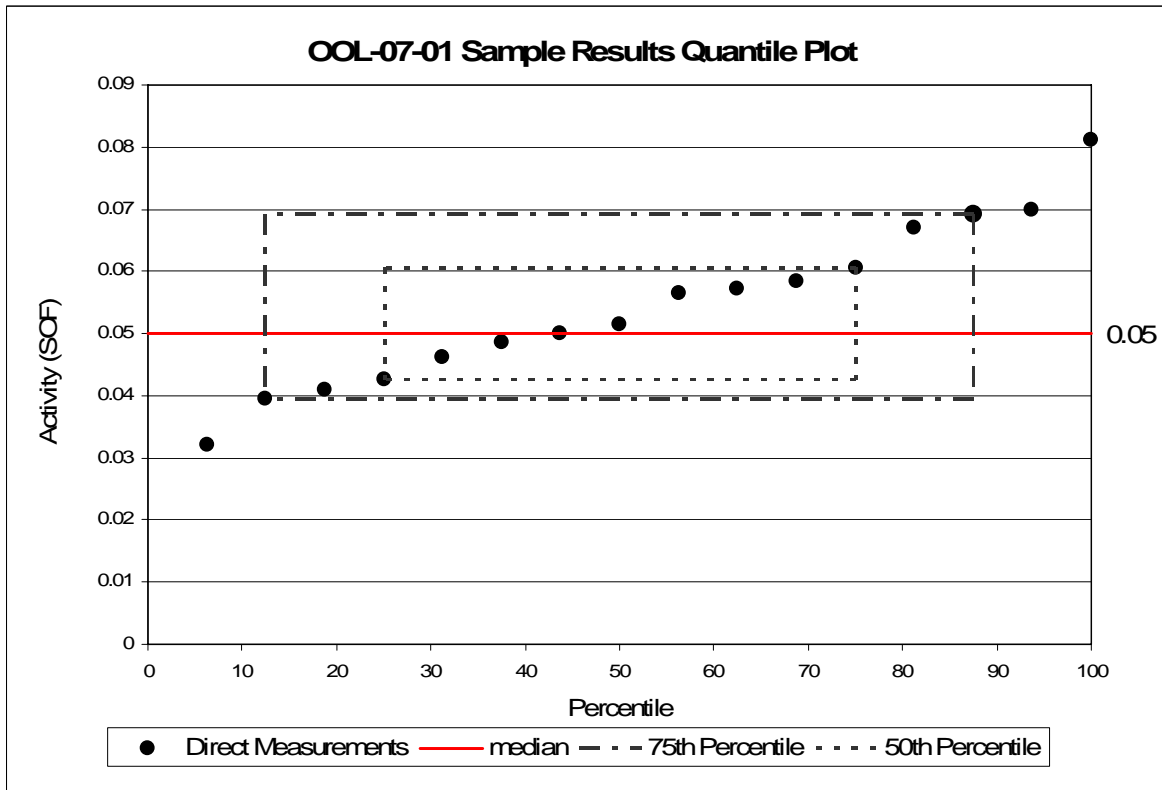
Figure 4 OOL-07-01 Sum of Fractions Quantile Plot
