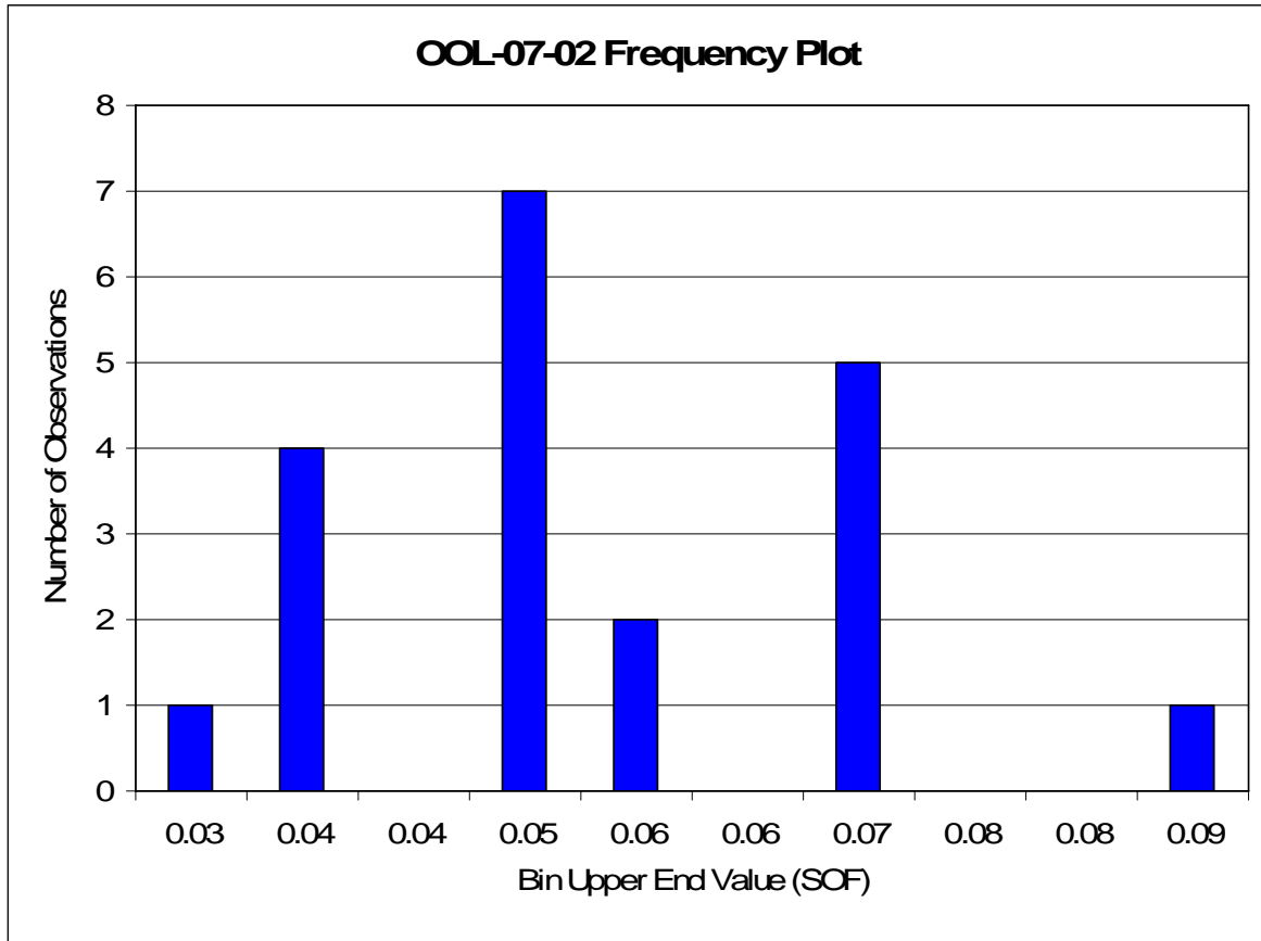
Figure 10 OOL-07-02 Sum of Fractions Frequency Plot
