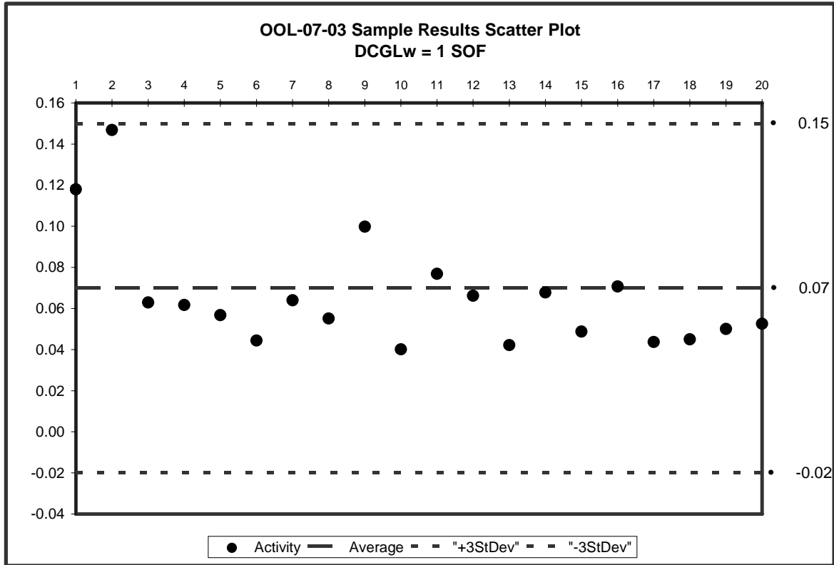
Figure 13 OOL-07-03 Sum of Fractions Scatter Plot
