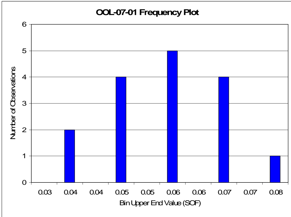
Figure 5 OOL-07-01 Sum of Fractions Frequency Plot
