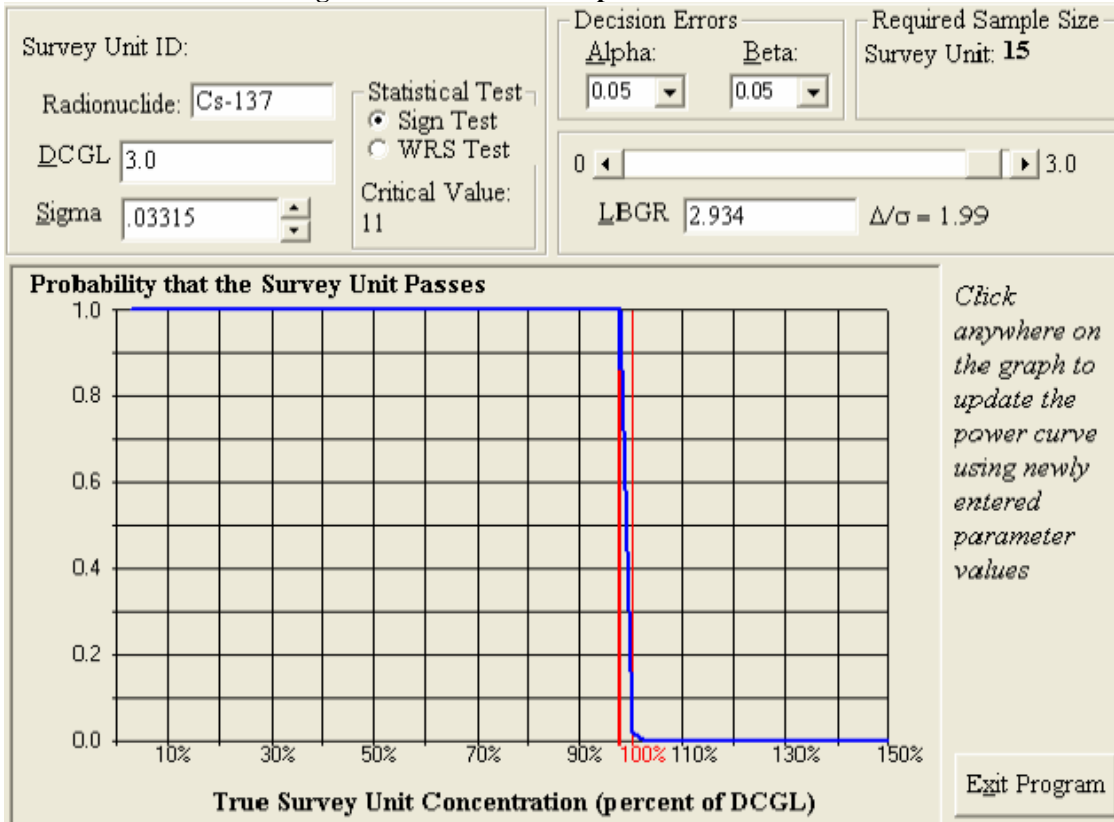
Figure 21 OOL-09-05 Retrospective Power Curve
