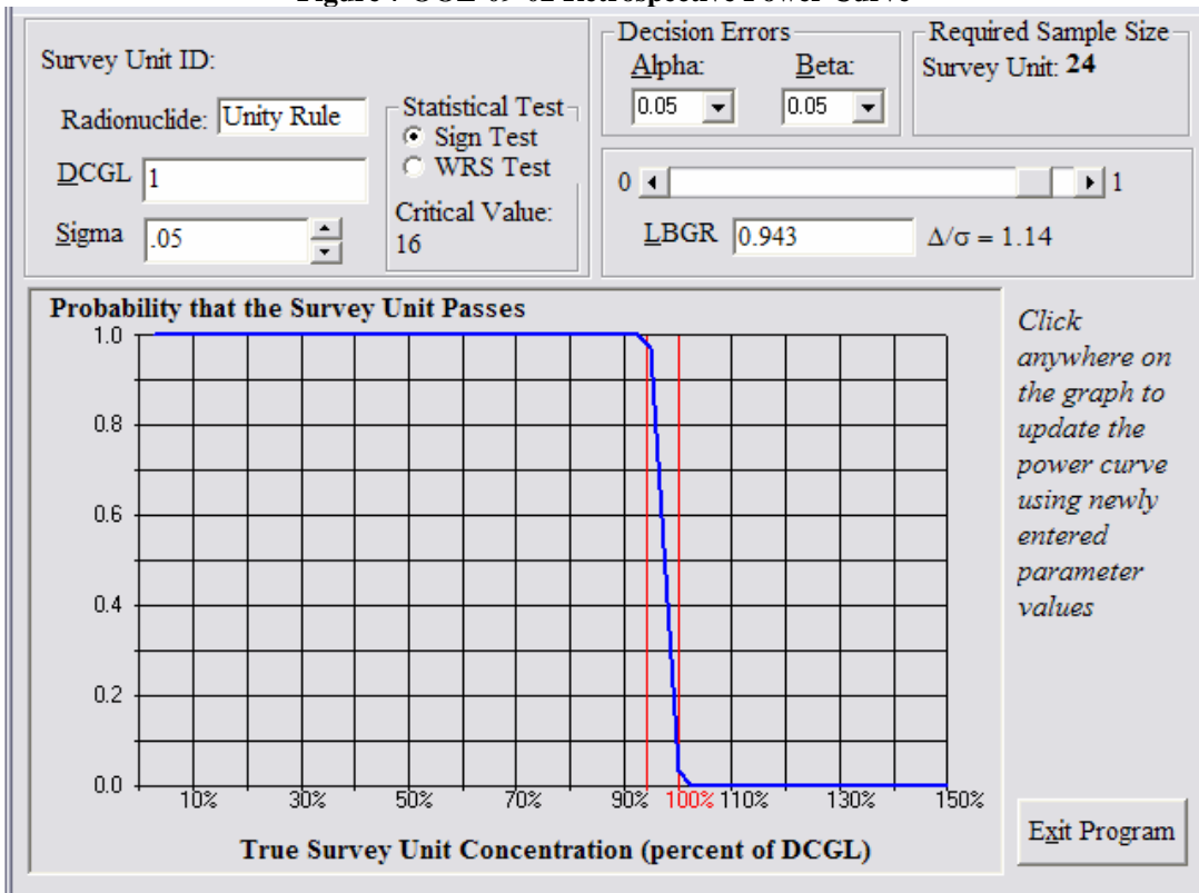
Figure 7 OOL-09-02 Retrospective Power Curve
