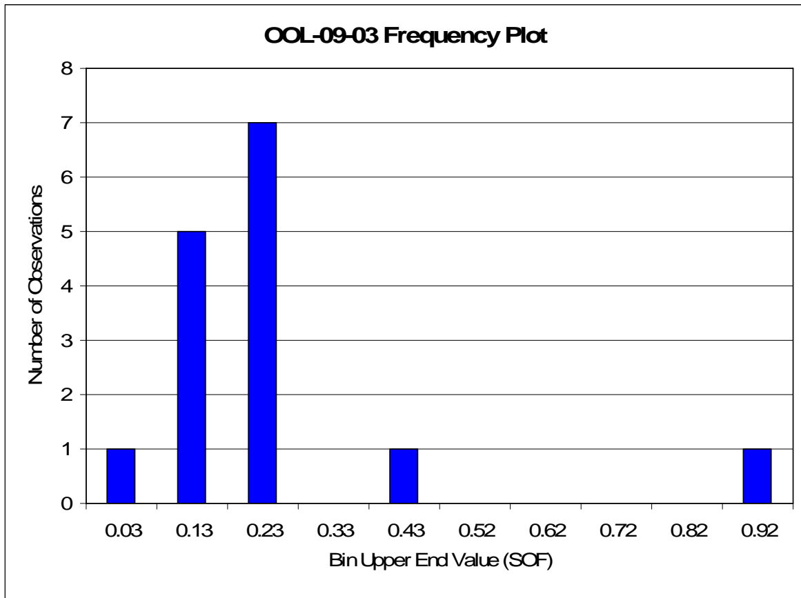
Figure 14 OOL-09-03 Sum of Fractions Frequency Plot
