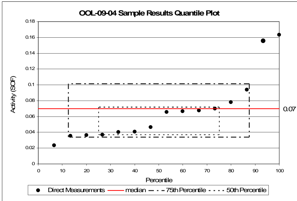
Figure 18 OOL-09-04 Sum of Fractions Quantile Plot
