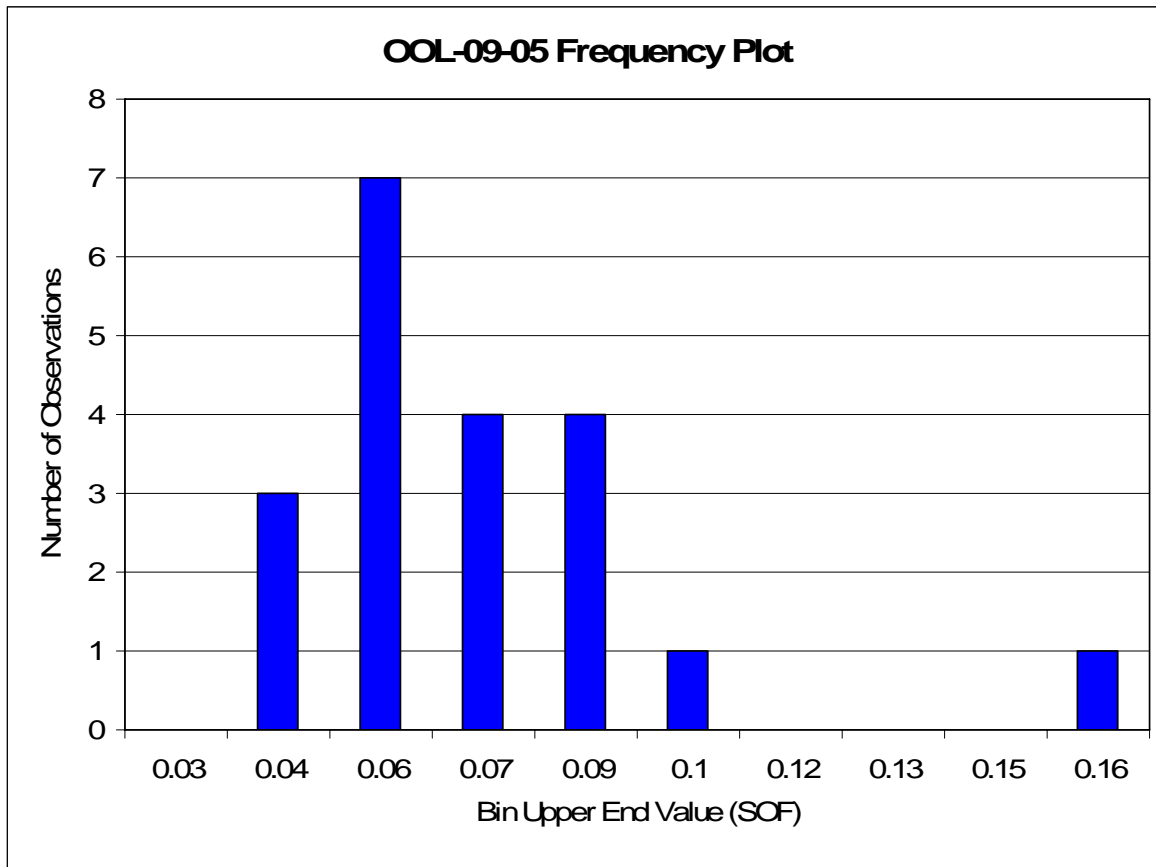
Figure 24 OOL-09-05 Sum of Fractions Frequency Plot
