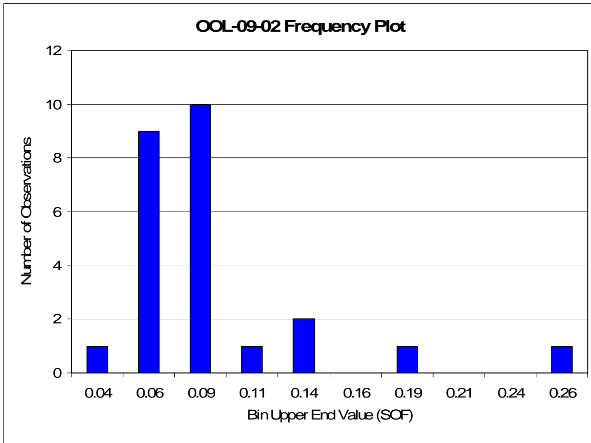
Figure 10 OOL-09-02 Sum of Fractions Frequency Plot
