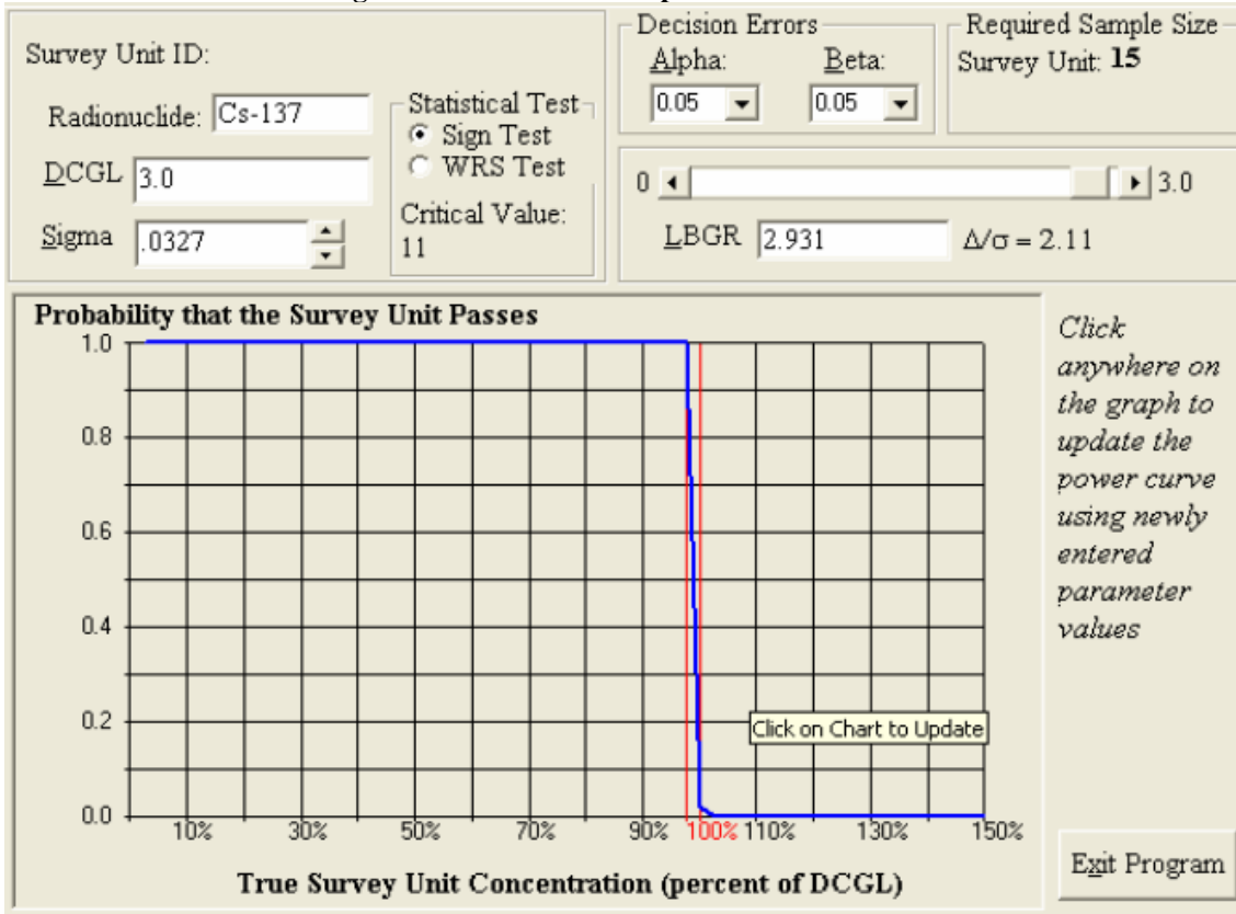
OOL-09-03 Retrospective Power Curve
