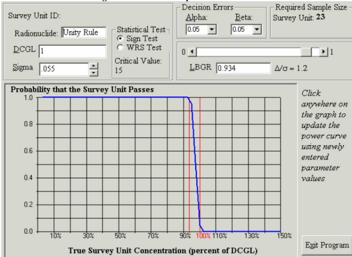
Figure 7 OOL-09-02 Retrospective Power Curve
