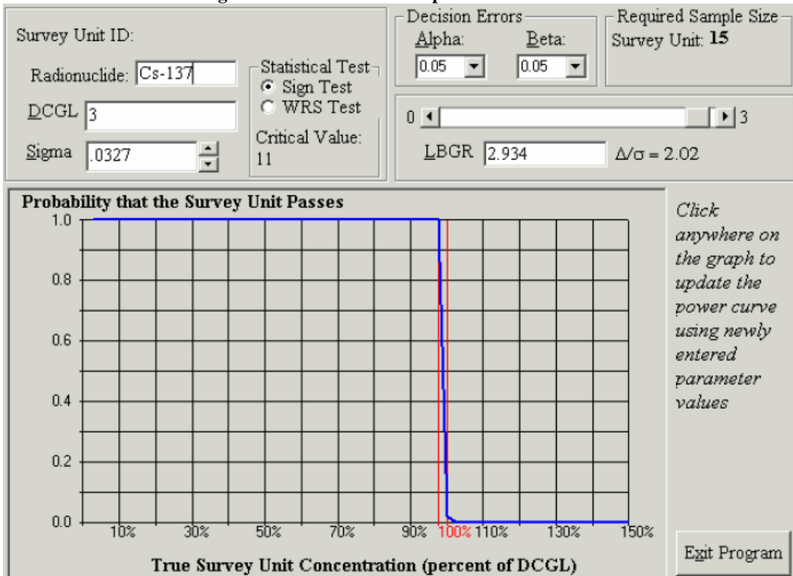
Figure 16 OOL-09-04 Retrospective Power Curve
