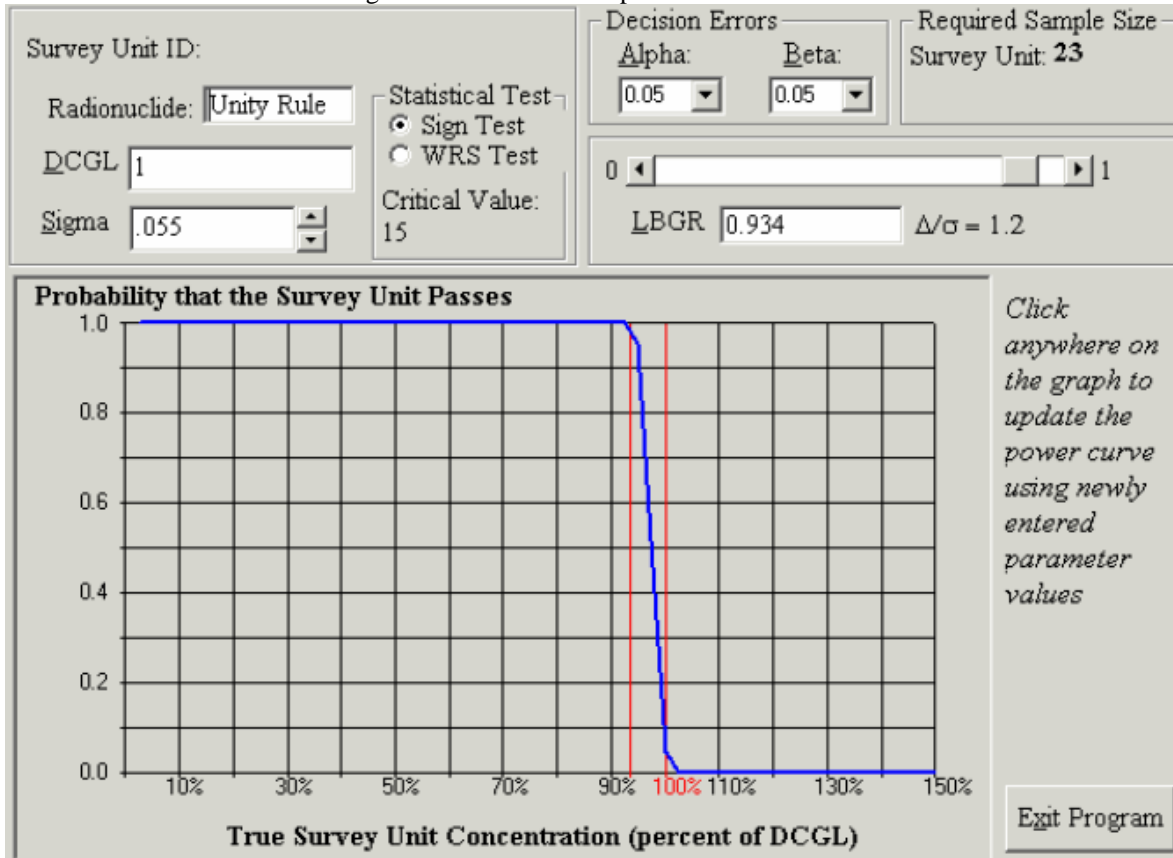
Figure 1 OOL-09-01 Prospective Power Curve
