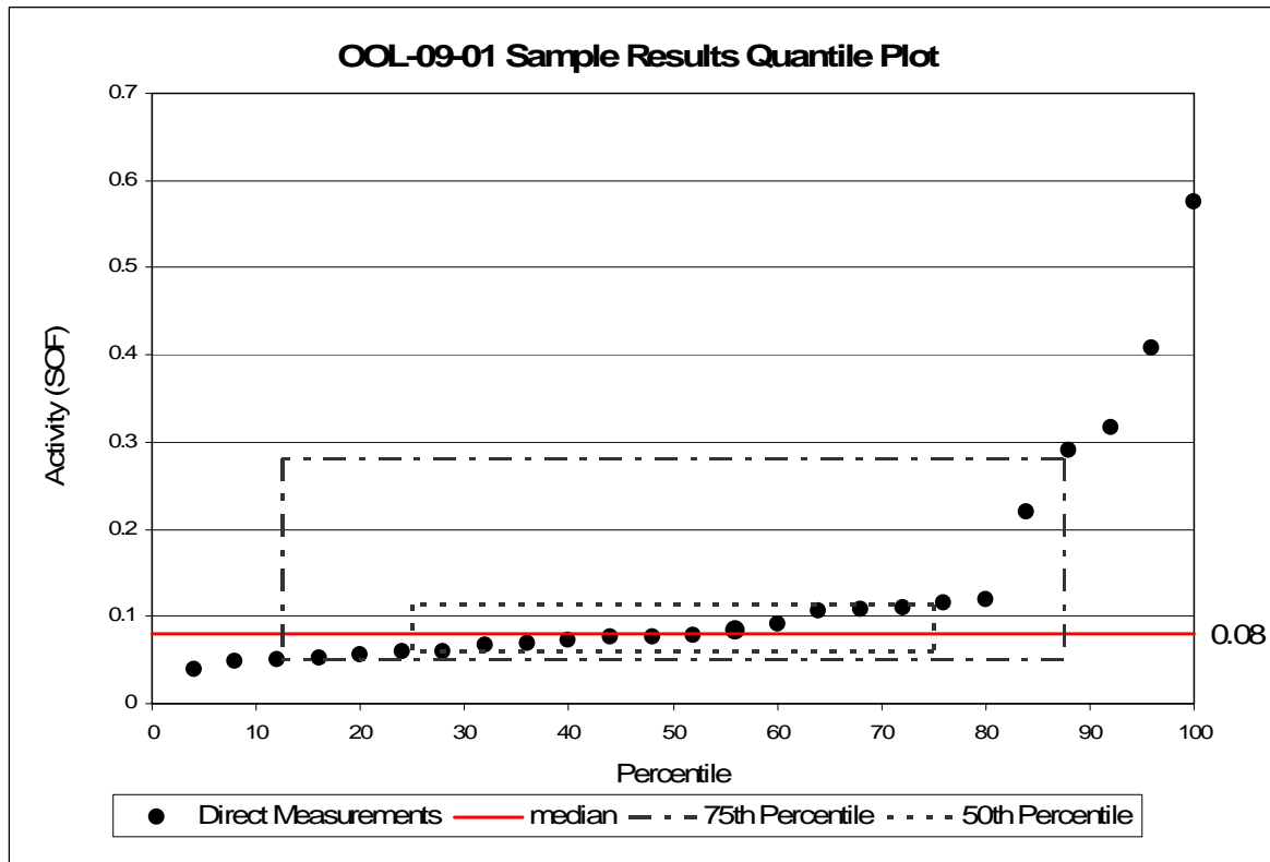
Figure 4 OOL-09-01 Sum of Fractions Quantile Plot
