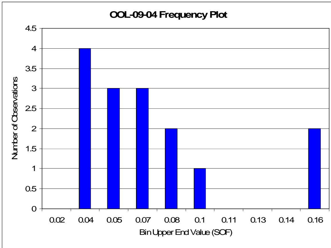
Figure 19 OOL-09-04 Sum of Fractions Frequency Plot
