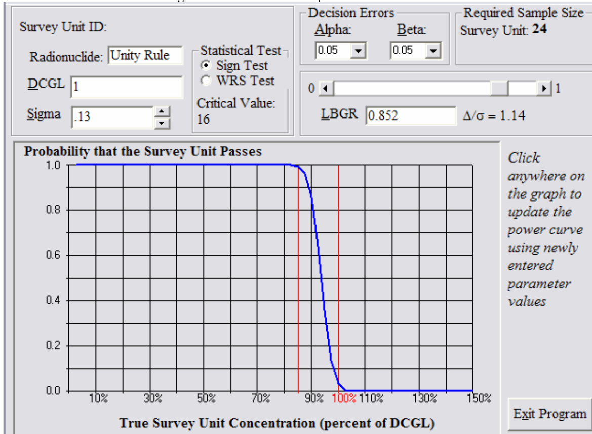
Figure 2 OOL-09-01 Retrospective Power Curve
