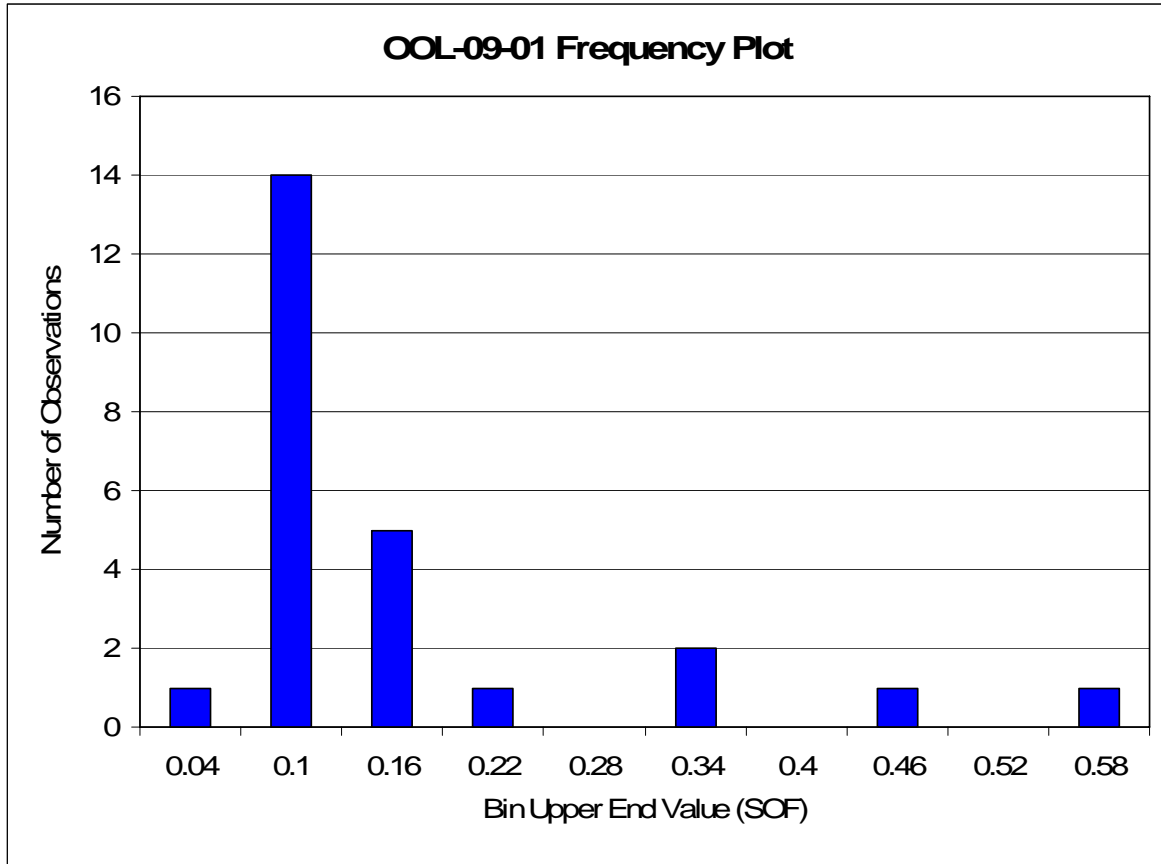
Figure 5 OOL-09-01 Sum of Fractions Frequency Plot
