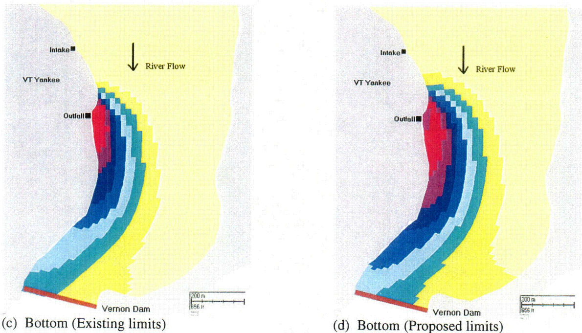
Figure 5-31. Predicted changes in Vermont Yankee's thermal plume surface or bottom area in lower Vernon Pool of the Connecticut River exposed to the average case (50% occurrence) of flow and ambient temperature under existing and proposed new summer thermal discharge limits for the spottail shiner avoidance temperature of 95°F.
