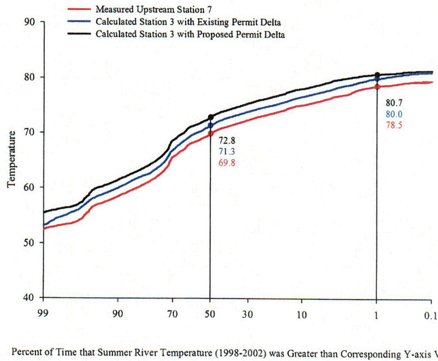
Figure 3-10. Comparison of Projected Temperature Response in the Connecticut River for Background, Existing and Proposed Vermont Yankee Discharge Conditions.
