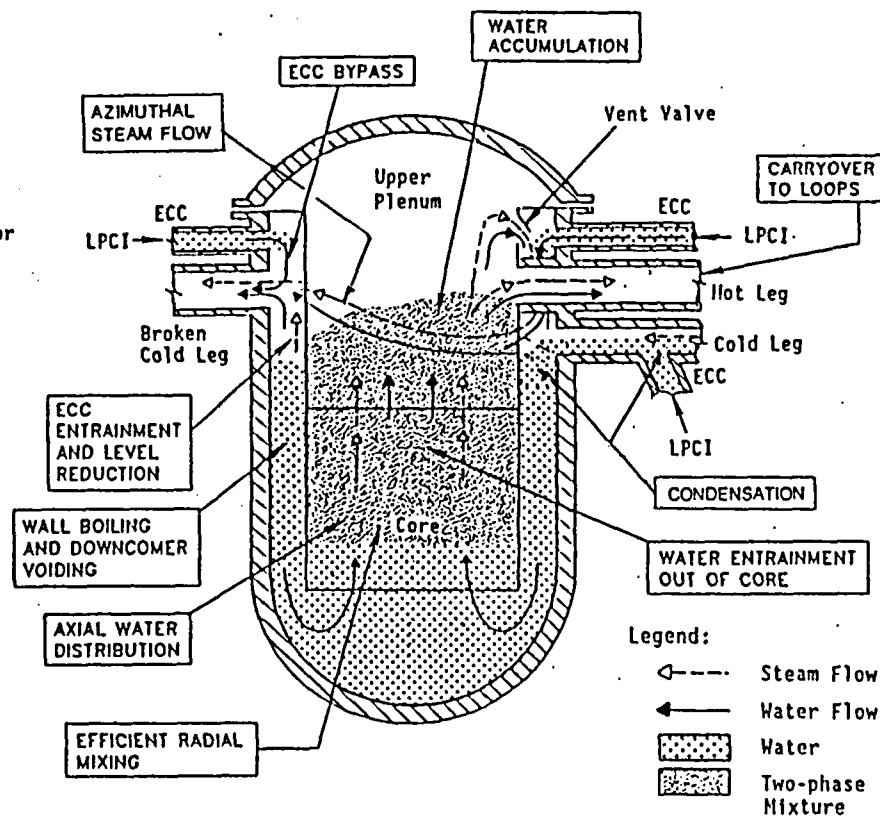
SUMMARY OF LBLOCA BEHAVIOR IN THE MK PWR REFLOOD
