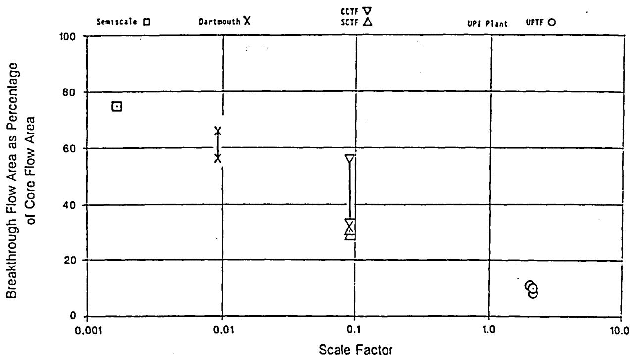
BREAKTHROUGH FLOW AREA VERSUS SCALE FACTOR (REFERENCE U-454)
