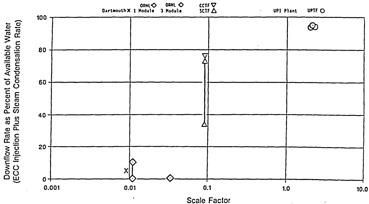
DOWNFLOW VERSUS SCALE FACTOR (REFERENCE U-454)
