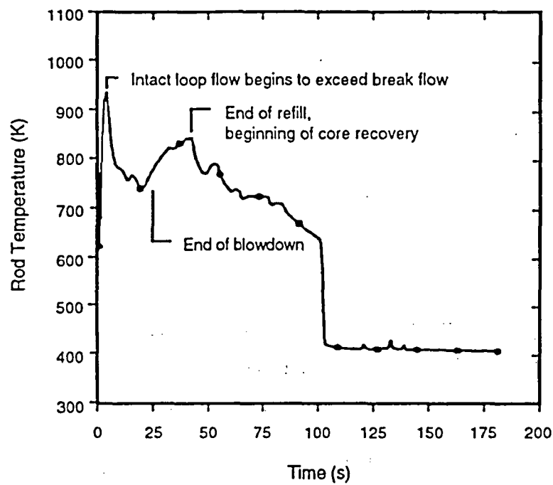
Maximum BE Rod Temperature
