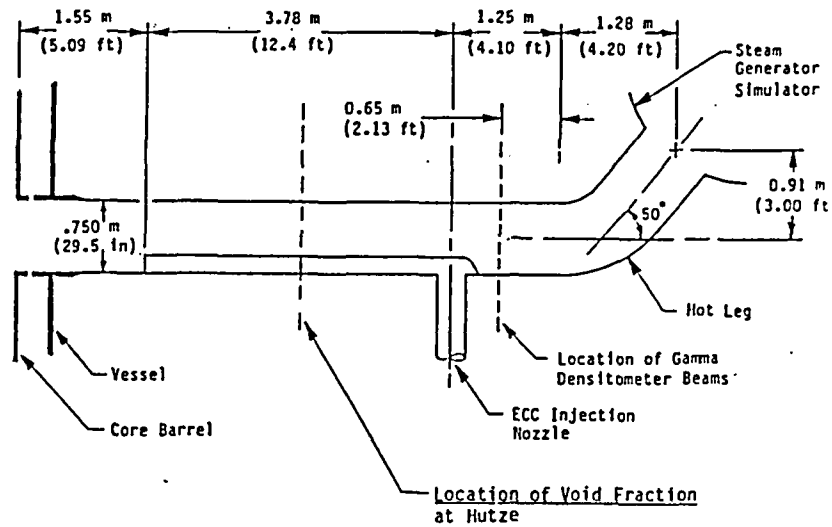
UPTF LOOP 4 HOT LEG
