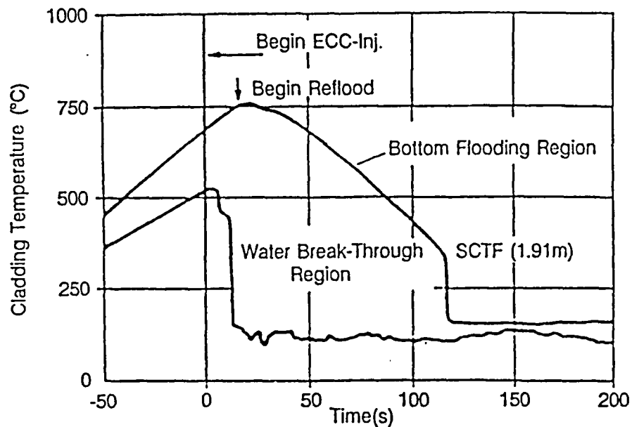
CLADDING TEMPERATURES WITH COMBINED ECC-INJECTION SCTF RUN 717
