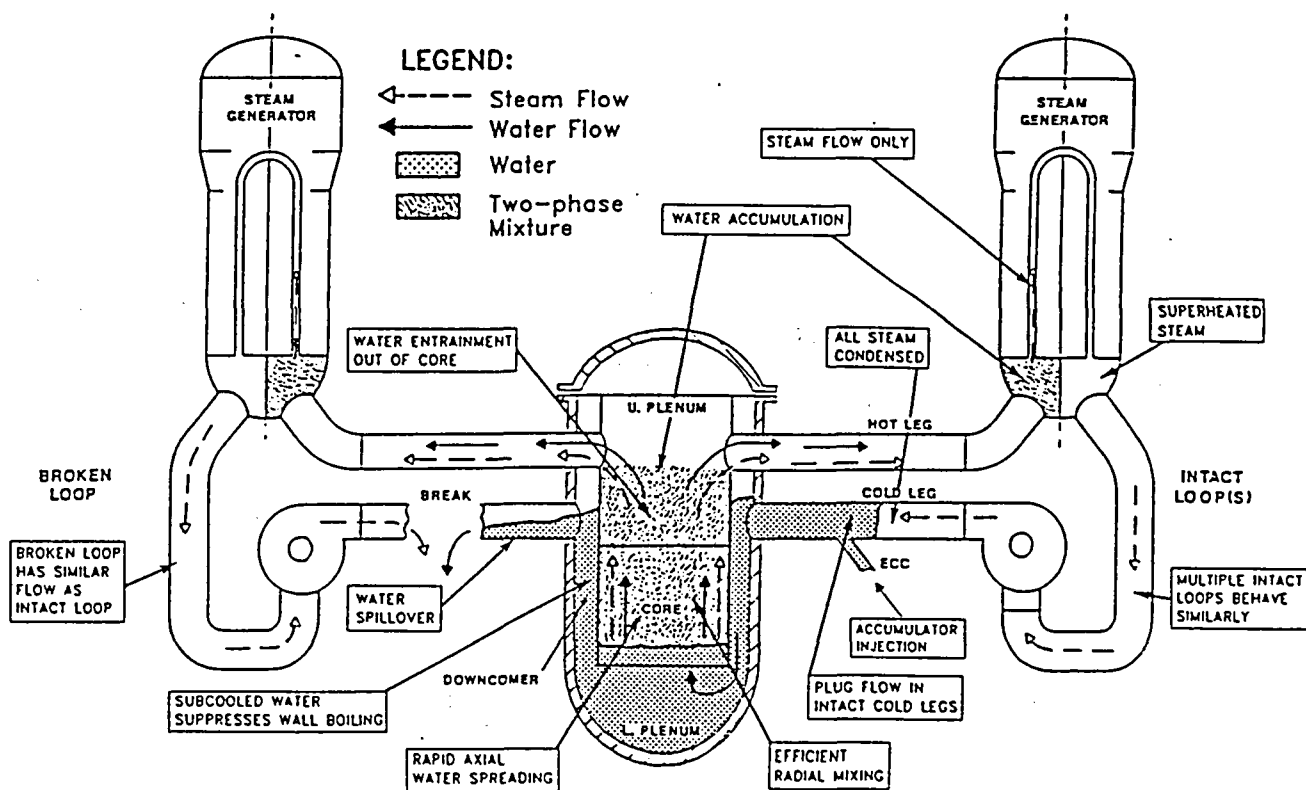
SUMMARY OF LBLOCA BEHAVIOR IN A COLD LEG INJECTION PWR EARLY REFLOW (ACCUMULATOR INJECTION)
