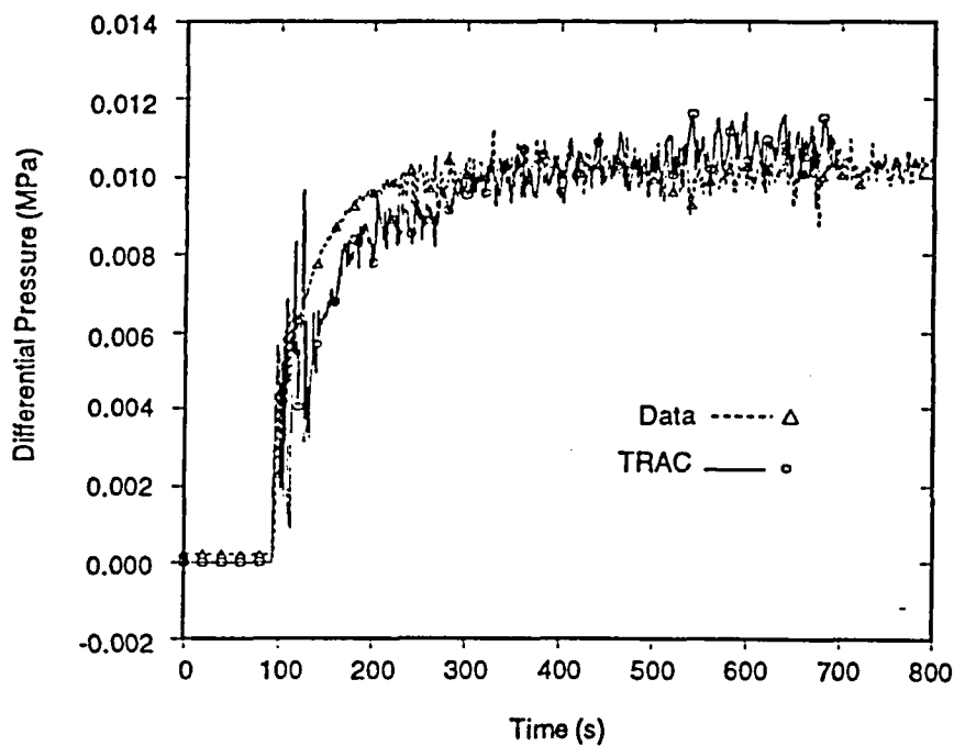
Core Lower Half \Delta P
