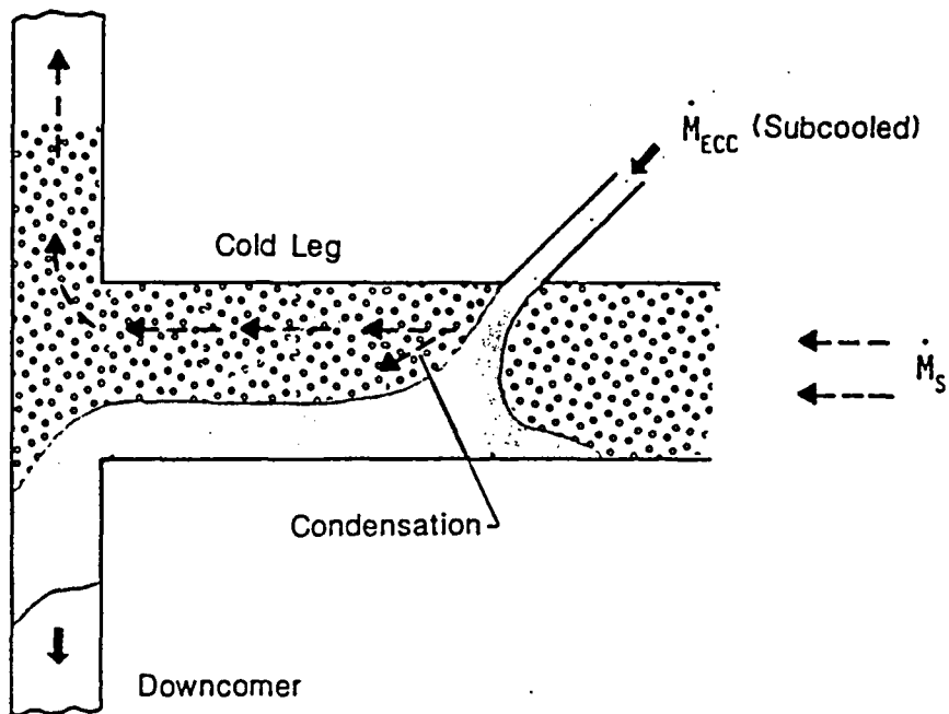
STRATIFIED FLOW
