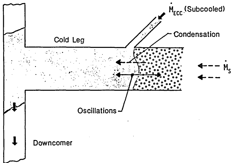
PLUG FLOW
