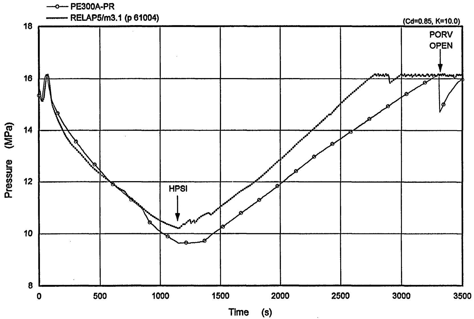
Figure 5.5 Pressurizer Pressure
