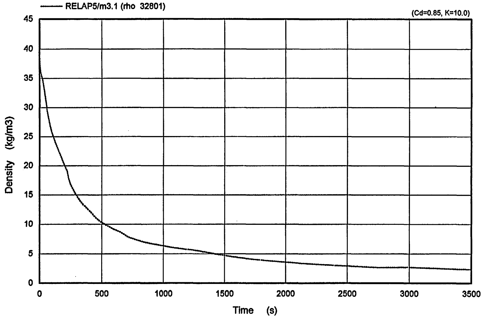
Figure 5.3 Break Density
