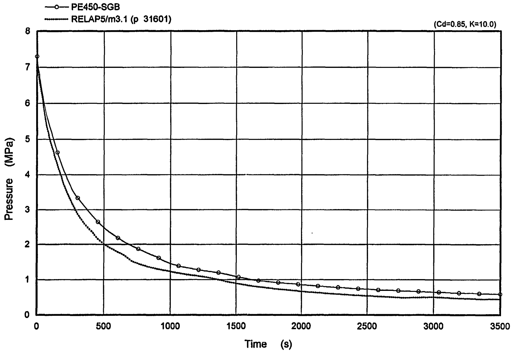
Figure 5.8 Secondary Pressure of Broken Loop
