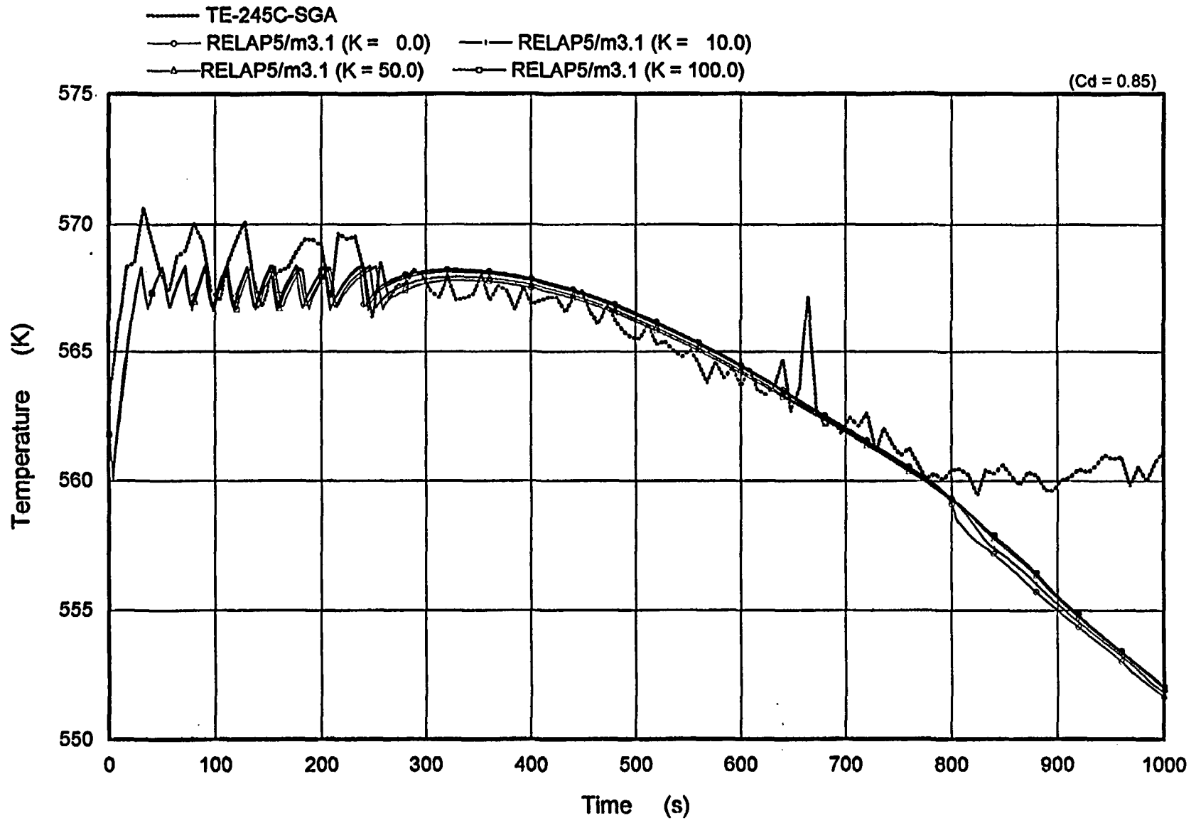
Figure 7.17 Comparison of Secondary Temperature of Intact Loop (K Value Sensitivity)
