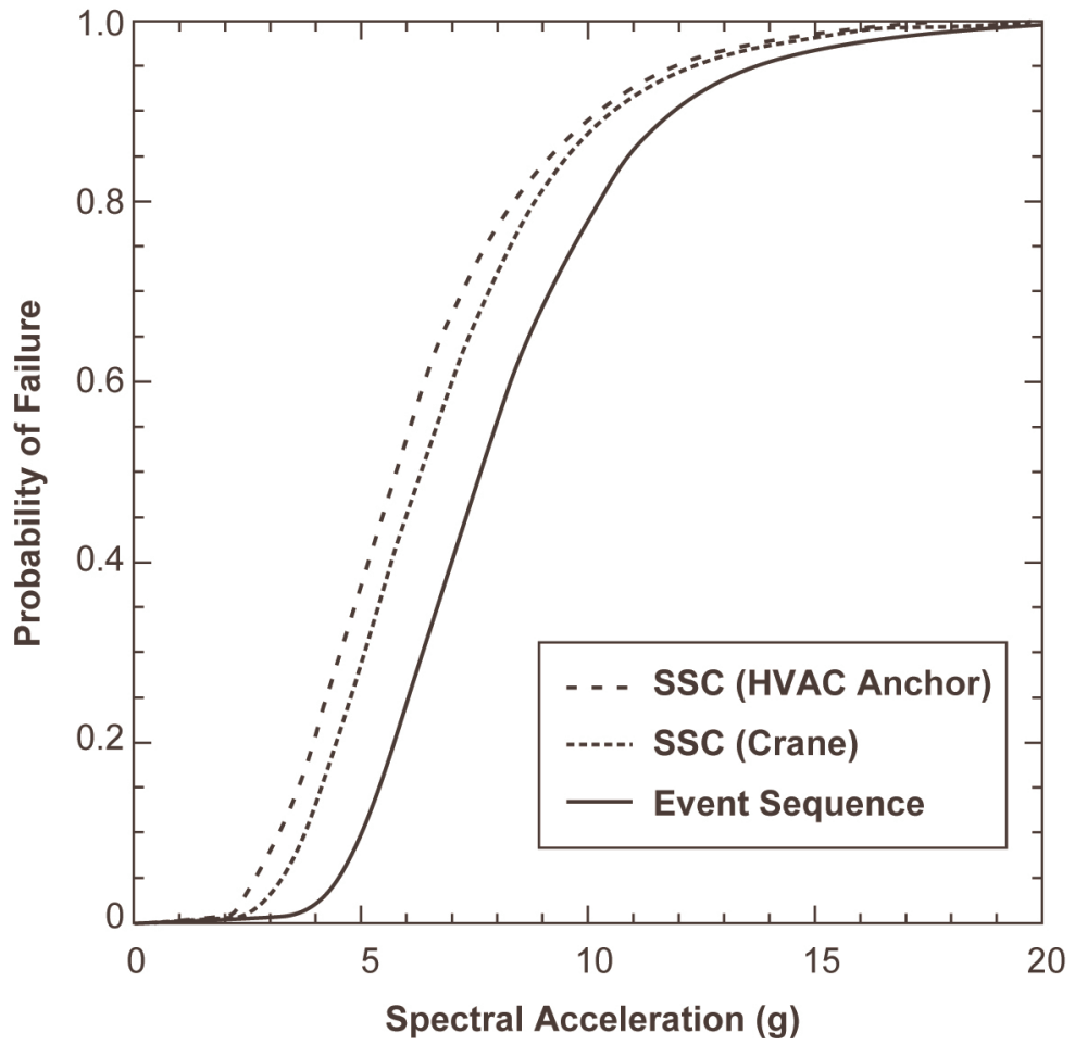
Figure B-2 Mean Fragility Curves for Event Sequence 3.
