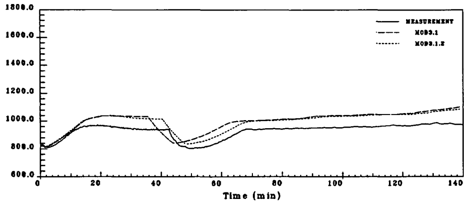
Figure 3.20: Test 9.1.b, Secondary side mass inventory
