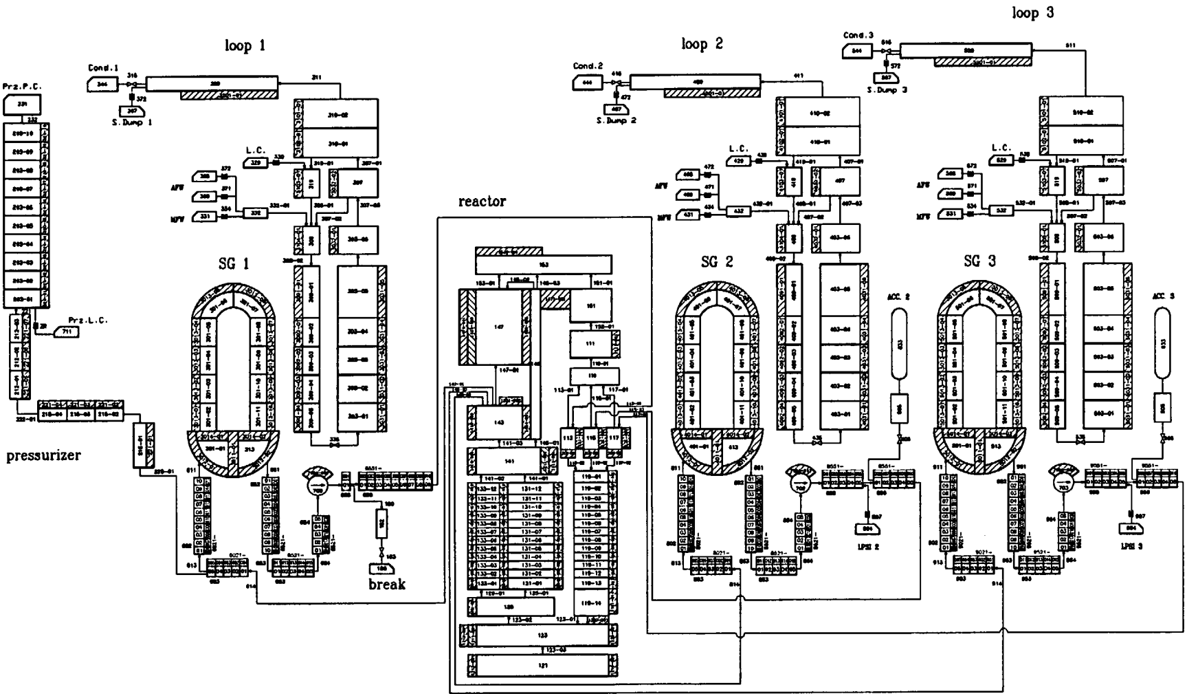
Figure 2.3: Enlarged (detailed) RELAP5 input model of BETHSY facility
