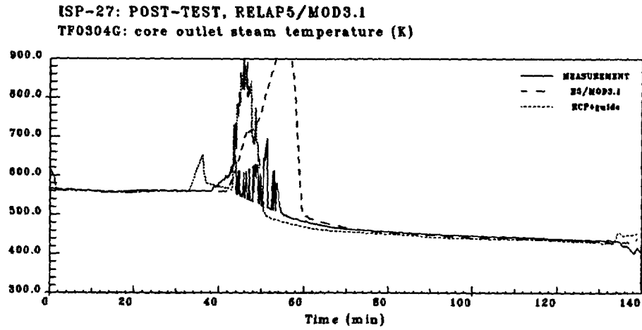
Figure 3.5: Test 9.1.b, Core outlet steam temperature
