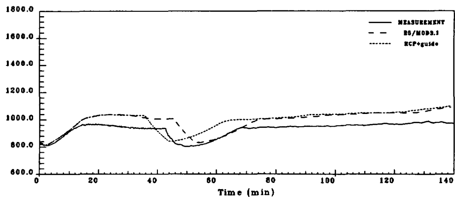
Figure 3.11: Test 9.1.b, Secondary side mass inventory
