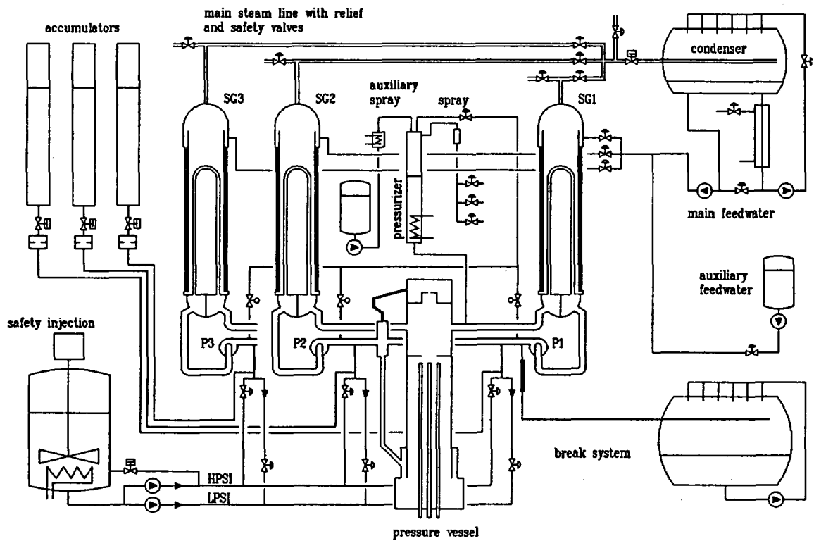
Figure 2.1: BETHSY facility
