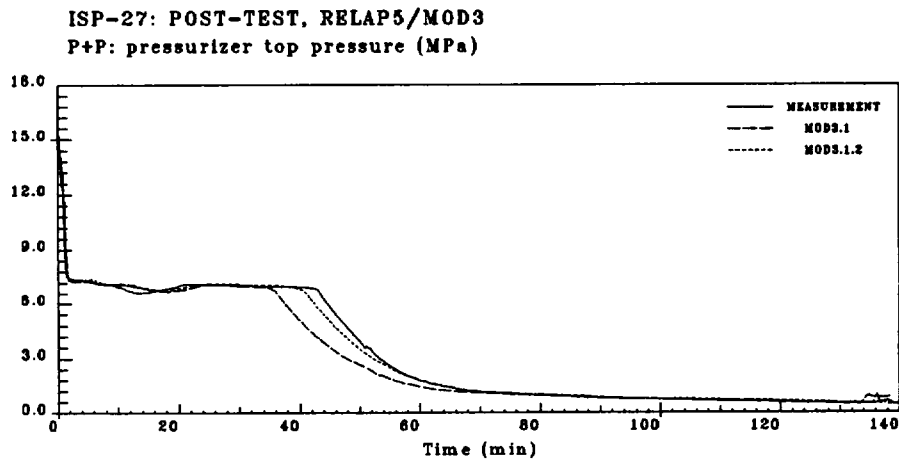
Figure 3.13: Test 9.1.b, Pressurizer pressure
