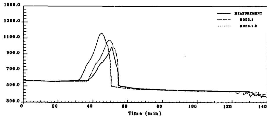
Figure 3.17: Test 9.1.b, Maximum cladding temperature
