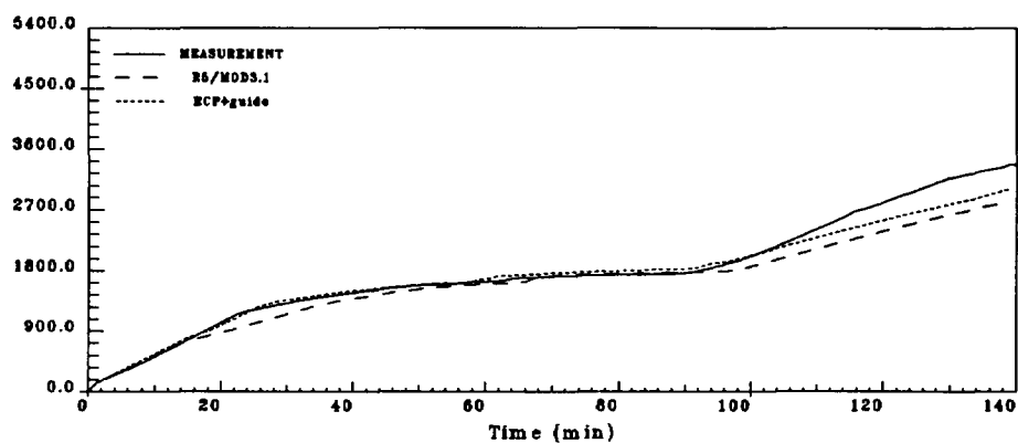
Figure 3.12: Test 9.1.b, Break discharged mass
