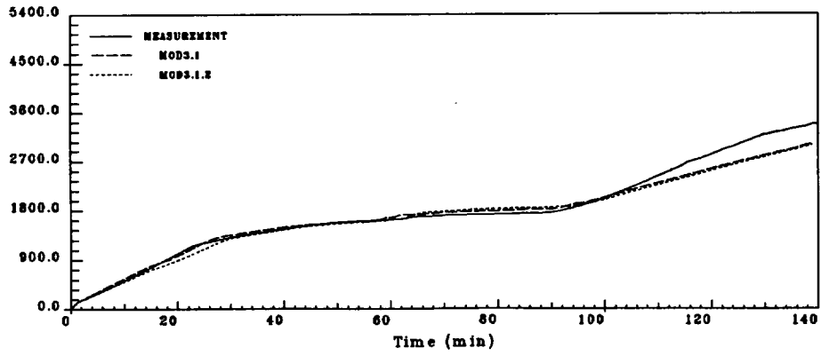
Figure 3.21: Test 9.1.b, Break discharged mass
