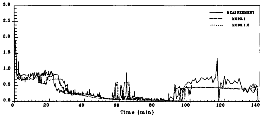
Figure 3.19: Test 9.1.b, Break mass flow rate
