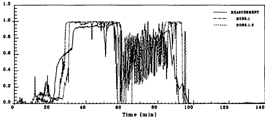
Figure 3.18: Test 9.1.b, No.1 CL spool piece void fraction
