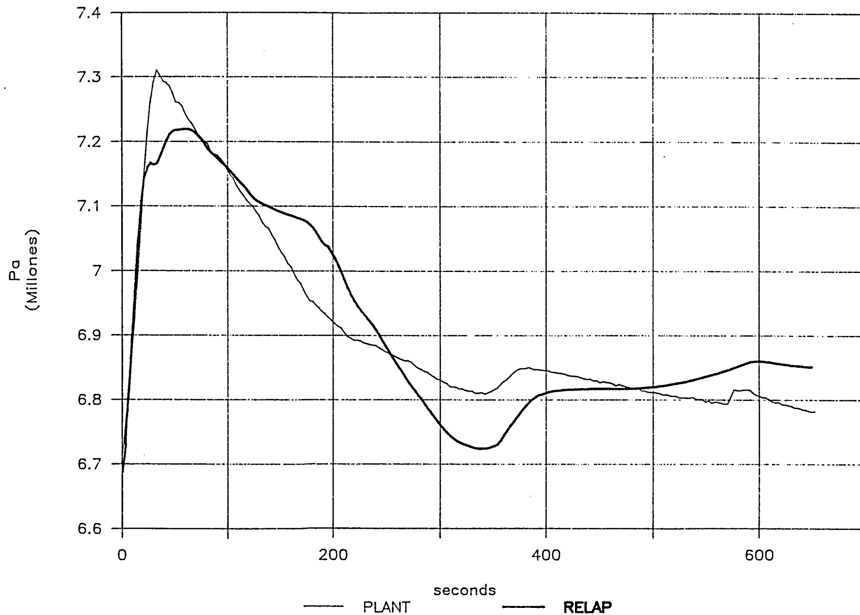
FIG.17 STEAM GENERATOR PRESSURE
