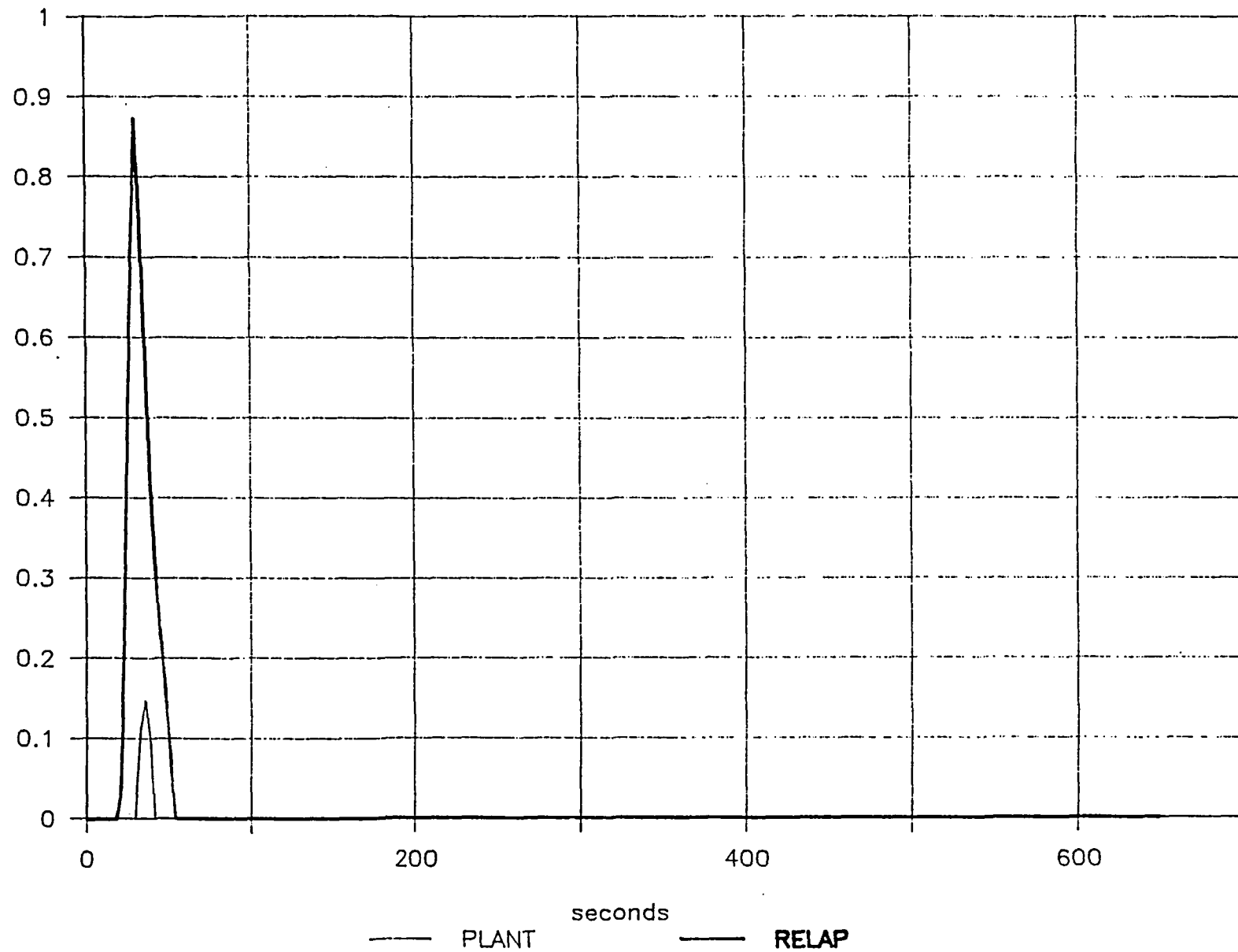
FIG.21 STEAM DUMP GR.3 VALVE POSITION
