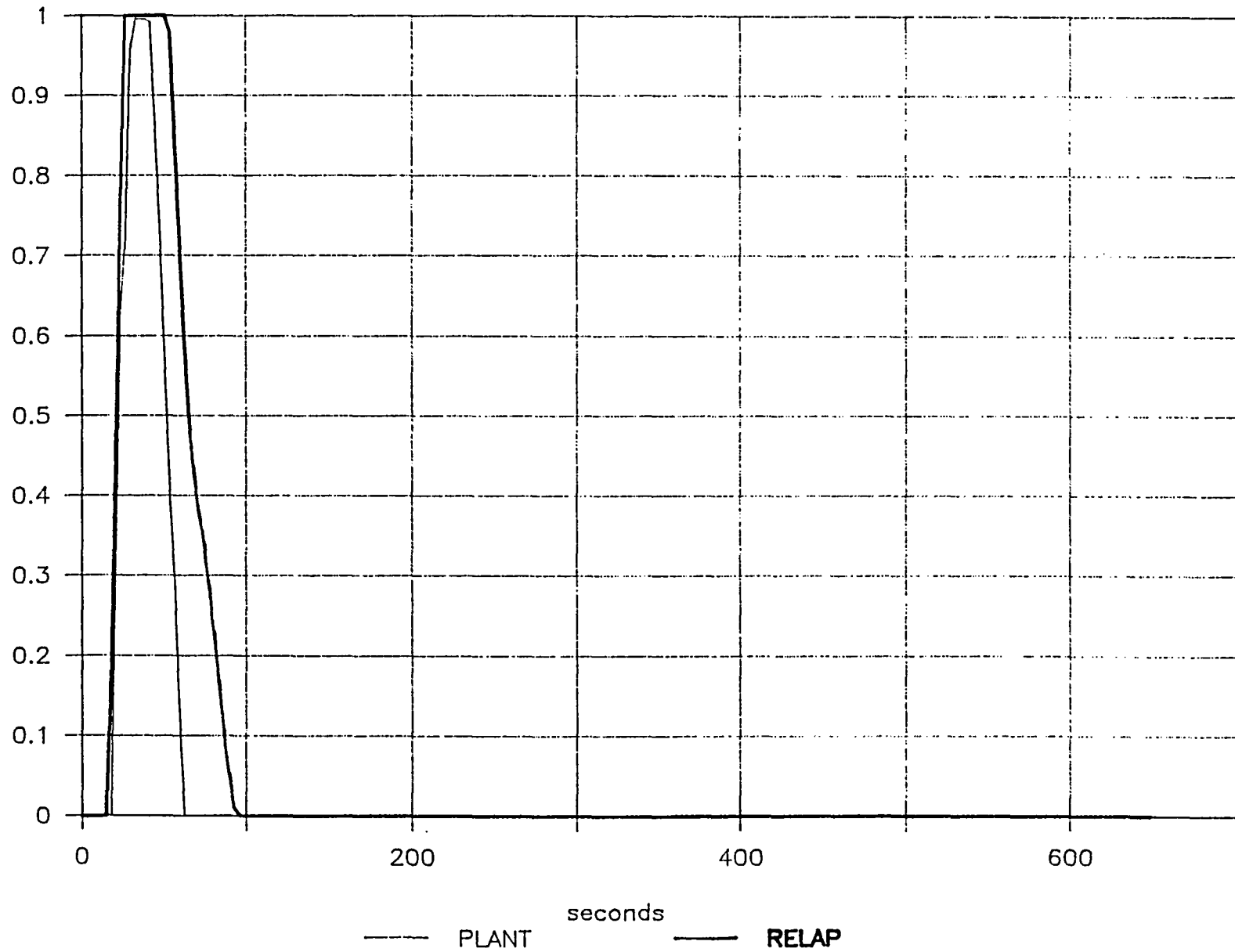
FIG.20 STEAM DUMP GR.2 VALVE POSITION
