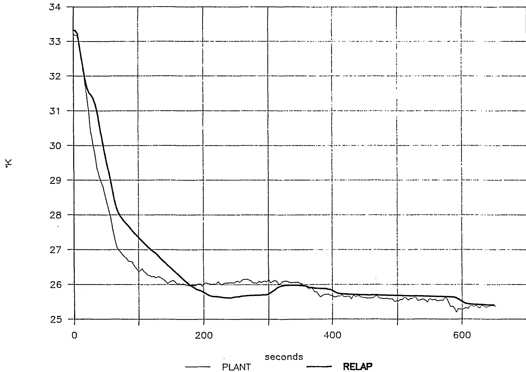
FIG.12 VESSEL DELTA TEMPERATURE
