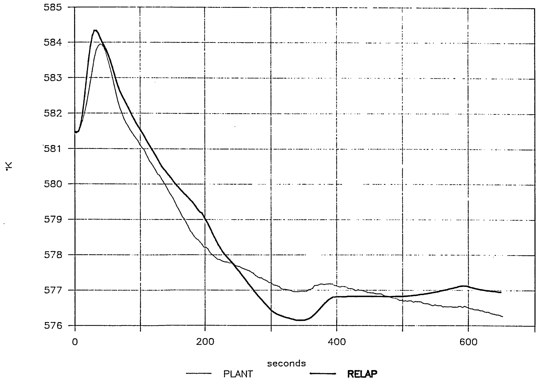
FIG.11 PRIMARY AVERAGE TEMPERATURE
