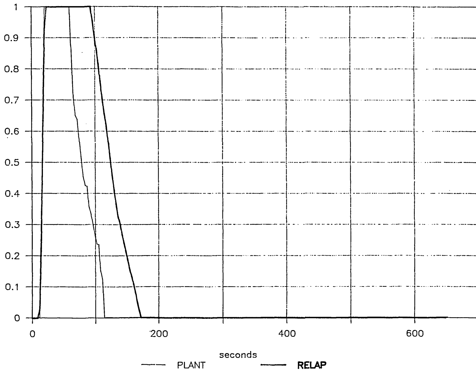
FIG.19 STEAM DUMP GR.1 VALVE POSITION
