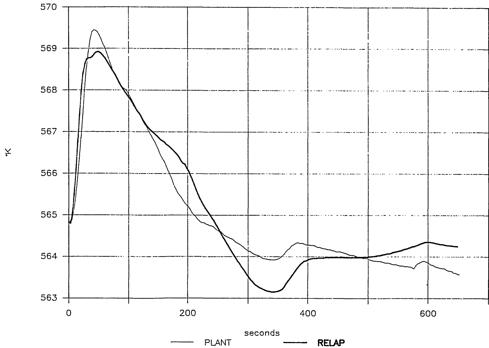
FIG.9 TEMPERATURE AT THE COLD LEG
