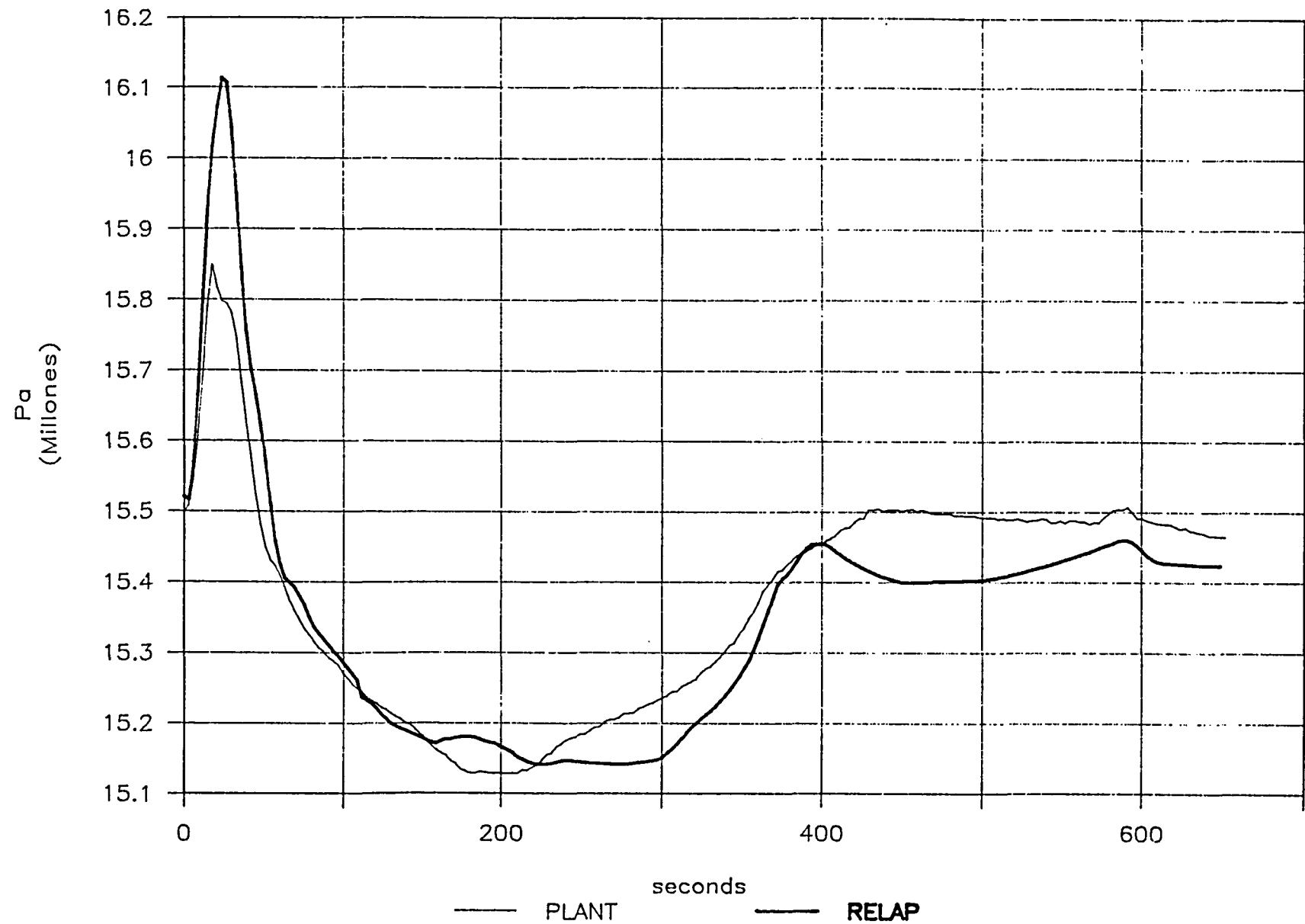
FIG.13 PRESSURIZER PRESSURE
