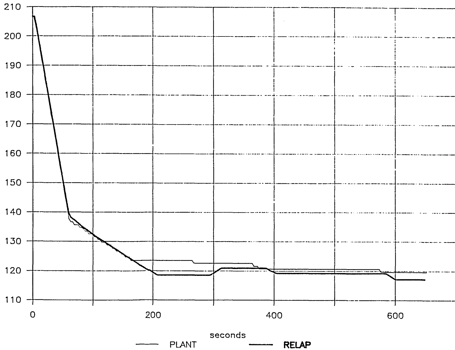
FIG.7 ROD POSITION (BANK D)
