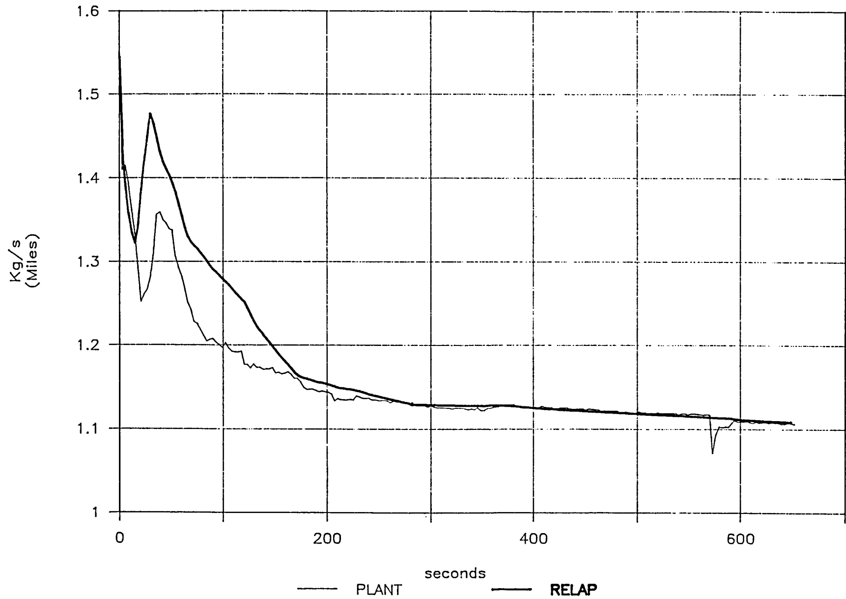
FIG.16 STEAM MASS FLOW RATE
