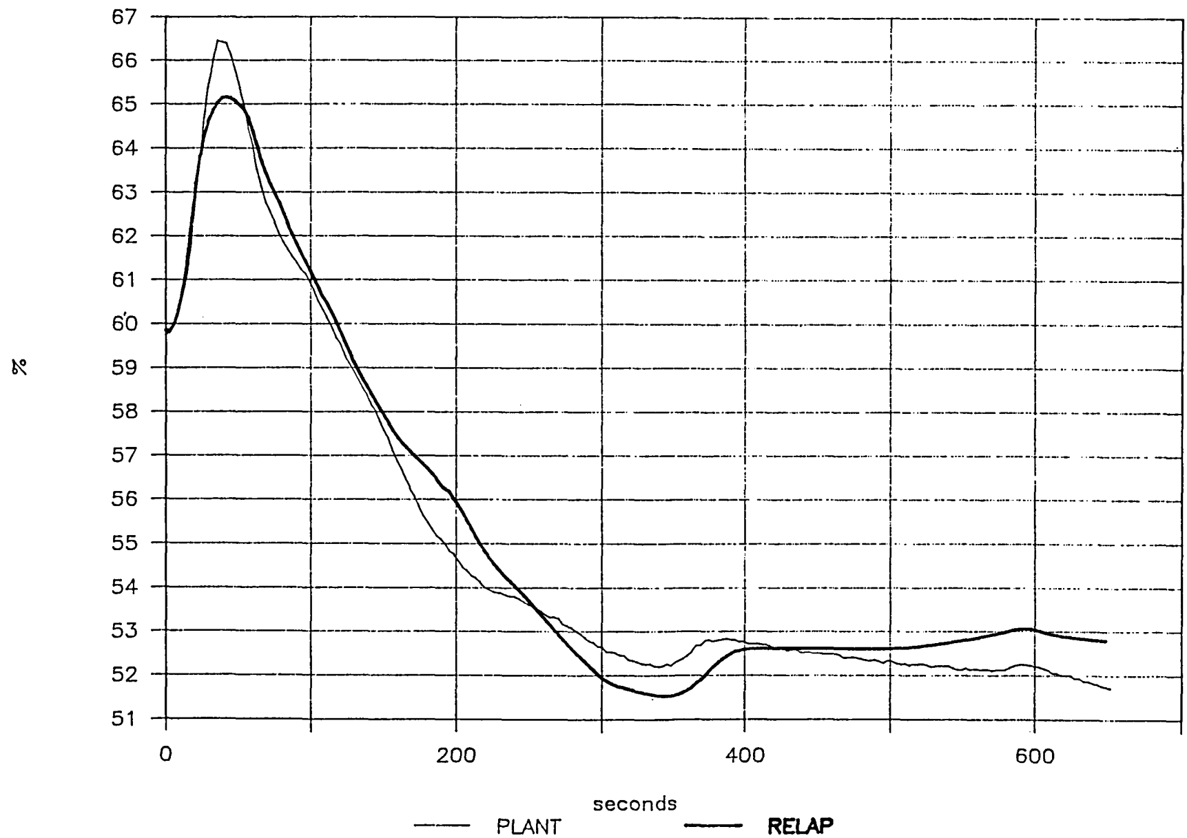
FIG.14 PRESSURIZER LEVEL
