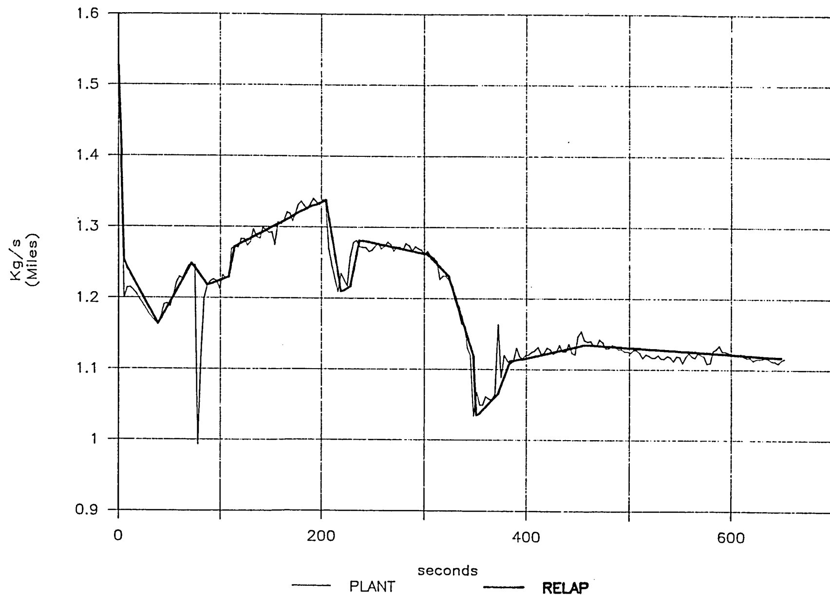
FIG.15 FEEDWATER MASS FLOW RATE
