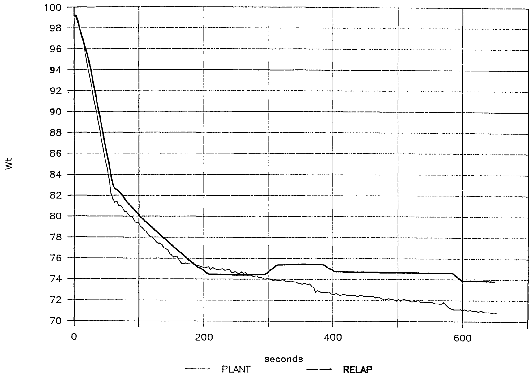
FIG.8 NUCLEAR POWER
