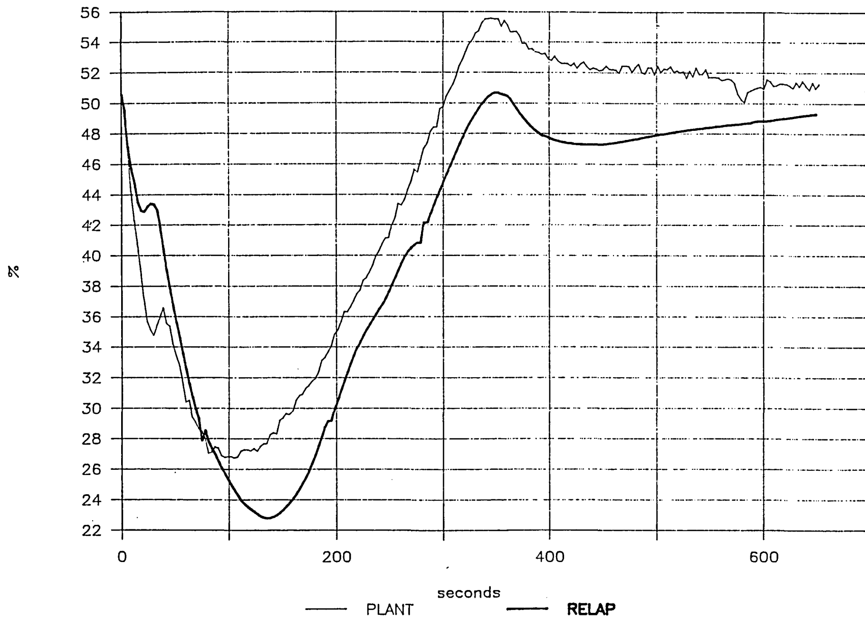
FIG.18 STEAM GENERATOR LEVEL
