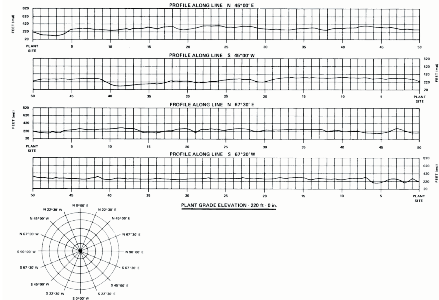
Figure 2.7-15 Terrain Elevation Profiles Within 50 Miles of the VEGP Site (Sheet 2 of 4)
