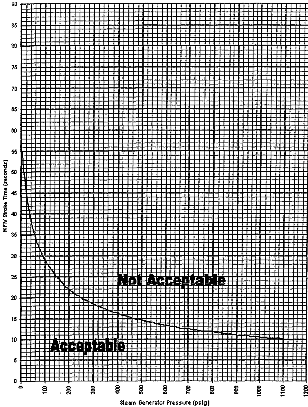
Figure 3.7.3-1 (page 1 of 1) MFIV Stroke Time Limit vs Steam Generator Pressure
