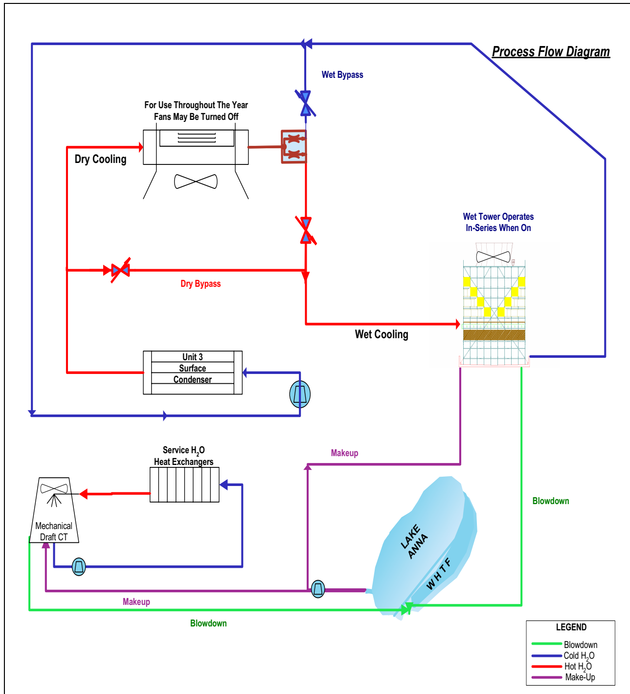
Figure 3.4-11 Conceptual Closed Loop Cooling Water Diagram
