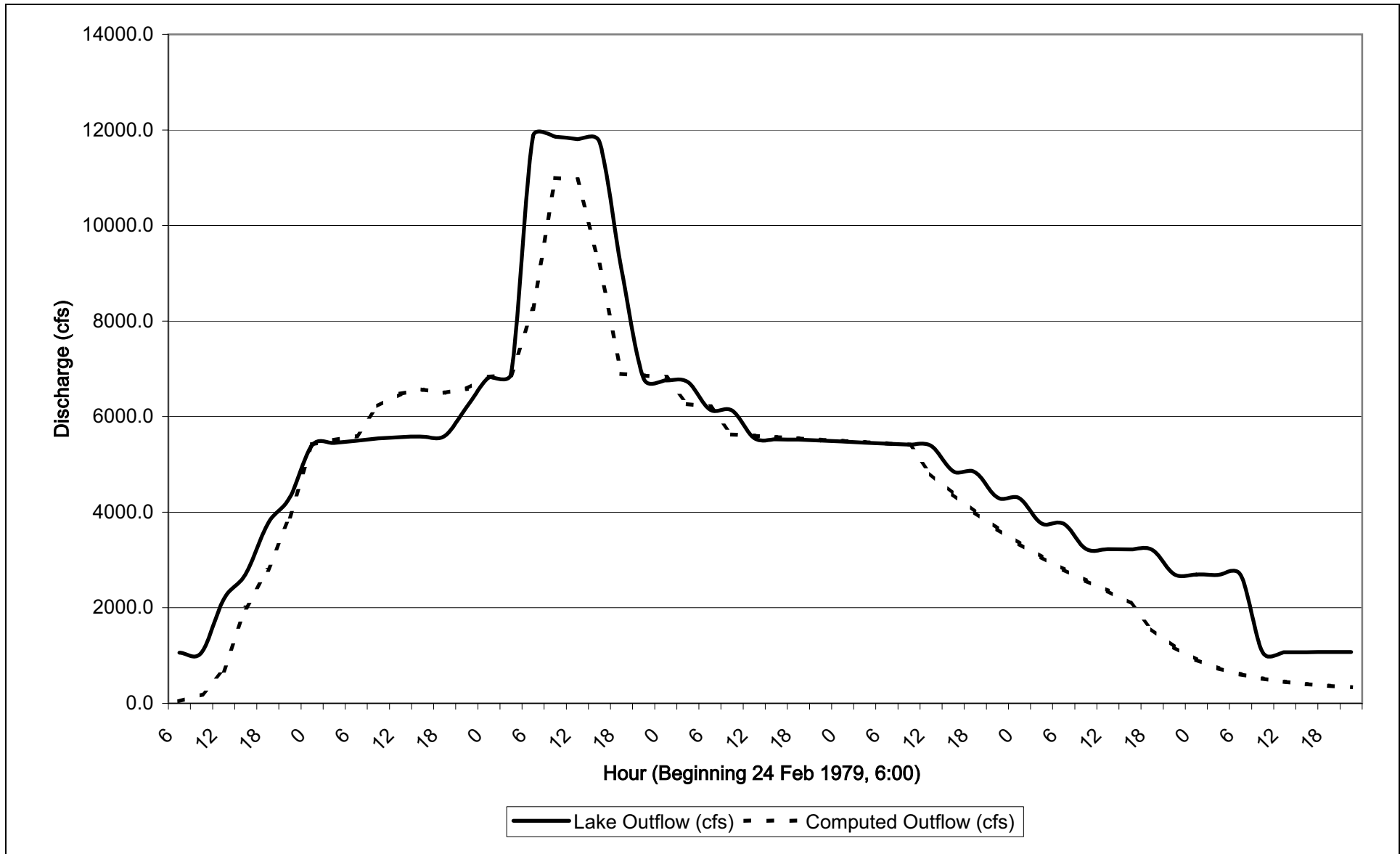
Figure 2.4-7 1979 Storm Outflow Hydrograph Comparison
