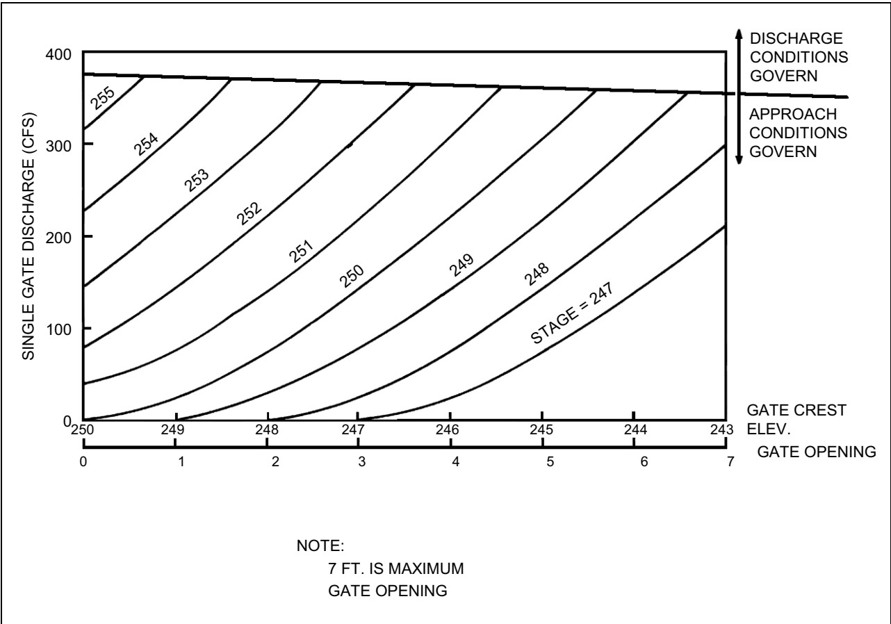
Figure 2.4-4 Skimmer Gate Discharge Capacity North Anna Dam
