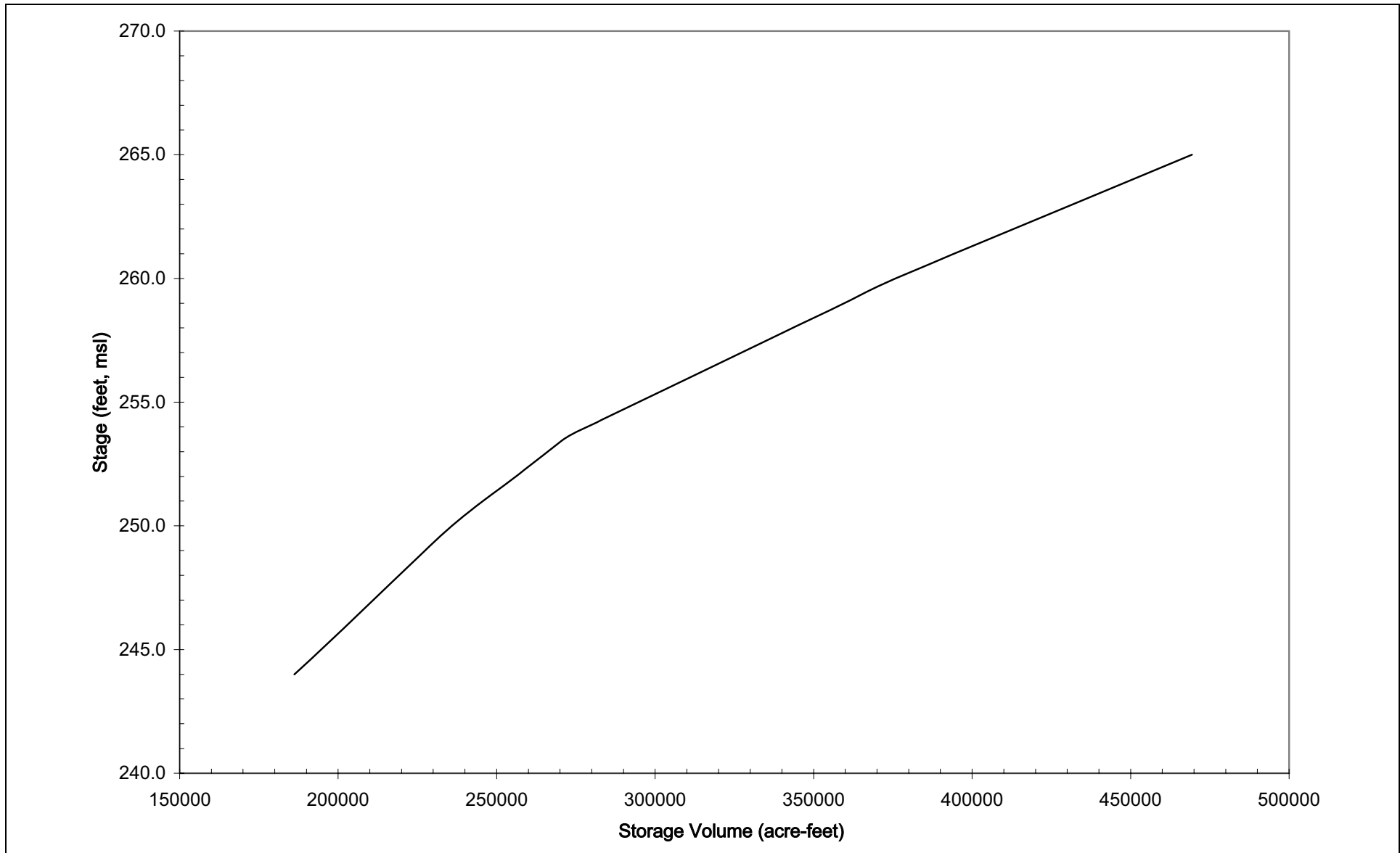
Figure 2.4-10 North Anna Reservoir & WHTF Combined Stage-Storage
