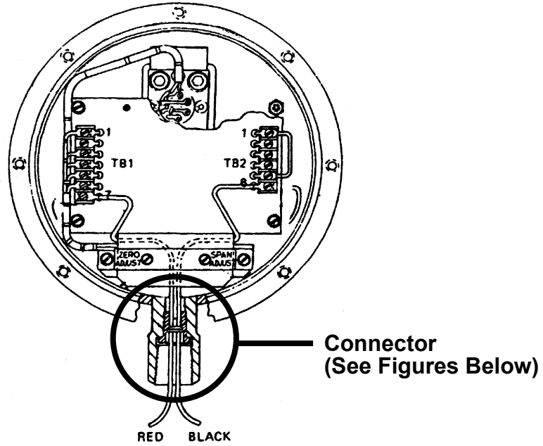
Model 764 Electronic Transmitter - Internal View (Model 763/763A Similar)
