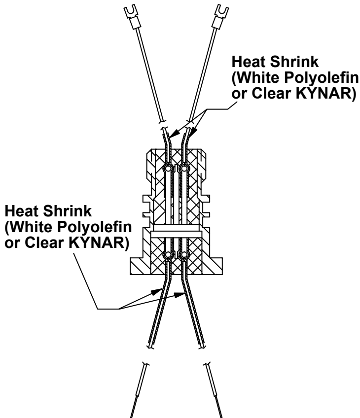
Model 764 Electronic Transmitter - Internal View (Model 763/763A Similar)
