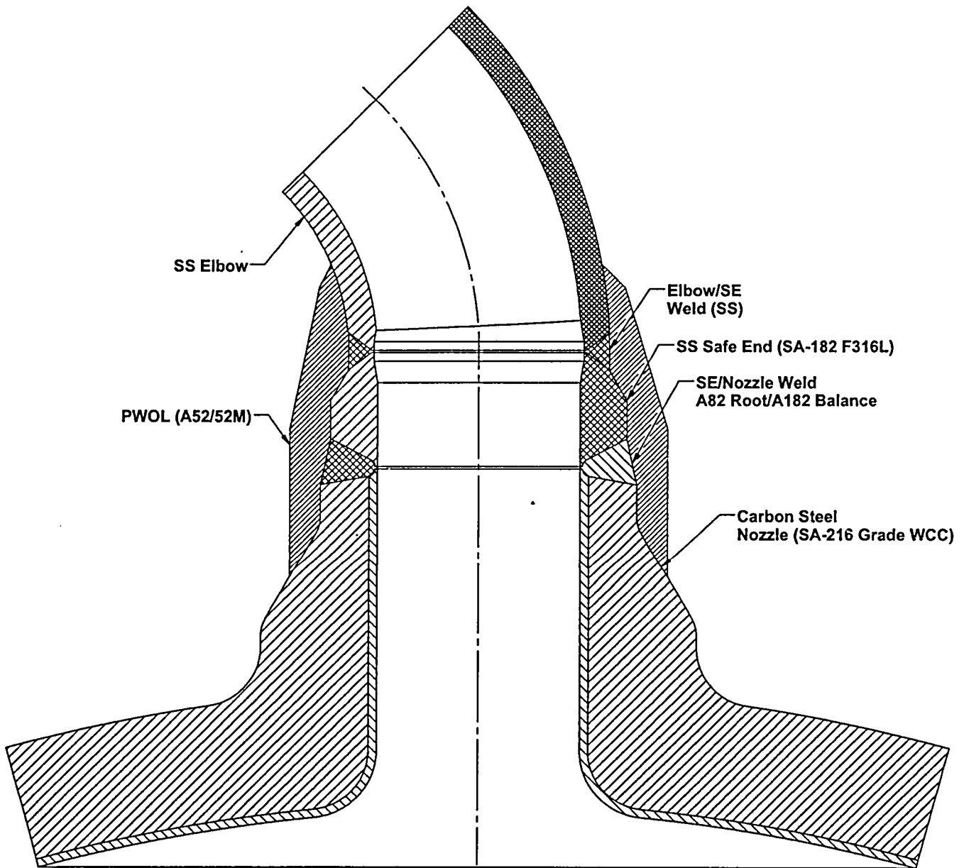
Figure 1 - Typical PWOL Configuration
