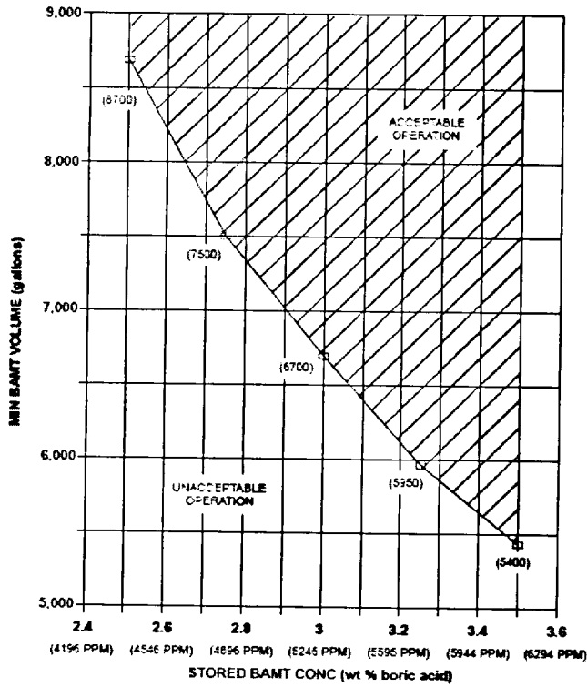
FIGURE 3.1-1 ST. LUCIE 1 MIN BANT VOLUME VS STORED BANT CONCENTRATION
