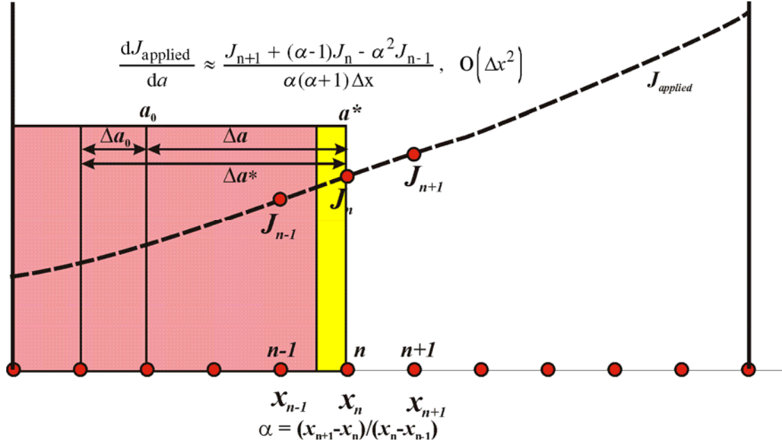
Fig. 19. IGA Propagation submodel mesh used to estimate dJ_{applied} / da using a second-order central finite-difference ratio.
