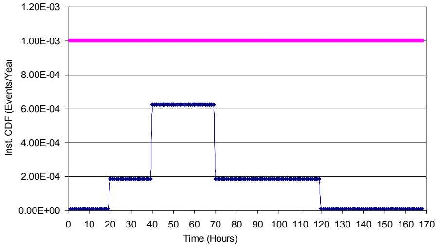
Figure 3-2 Configuration Risk Management – Instantaneous CDF Profile Example
