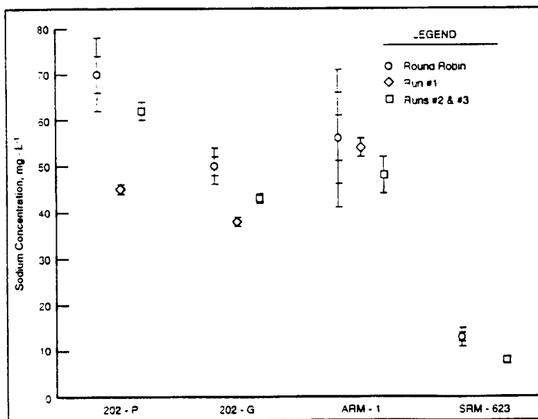
Figure 4. Release of Sodium as a Function of Glass Type
