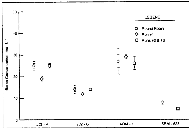
Figure 1. Release of Boron as a Function of Glass Type
