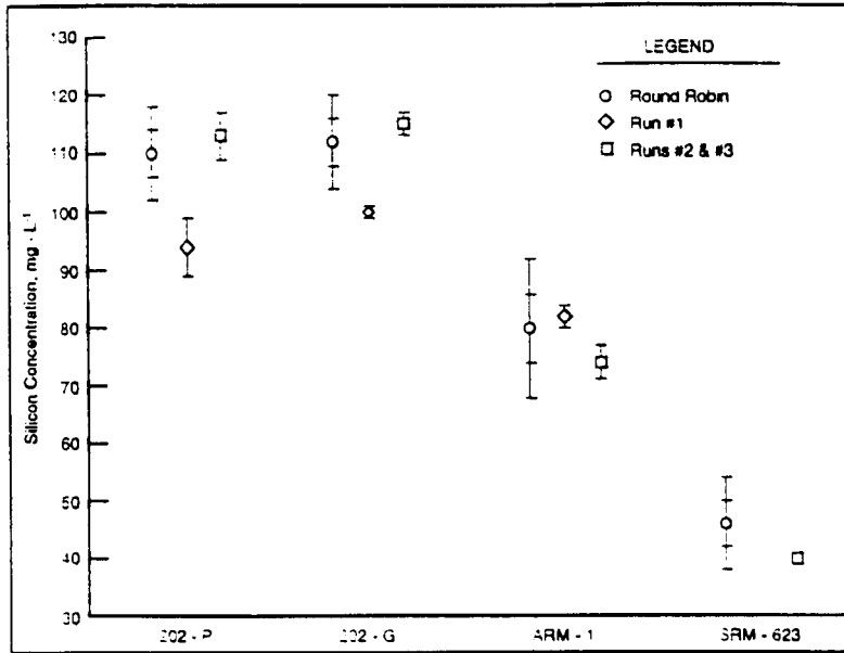
Figure 5. Release of Silicon as a Function of Glass Type
