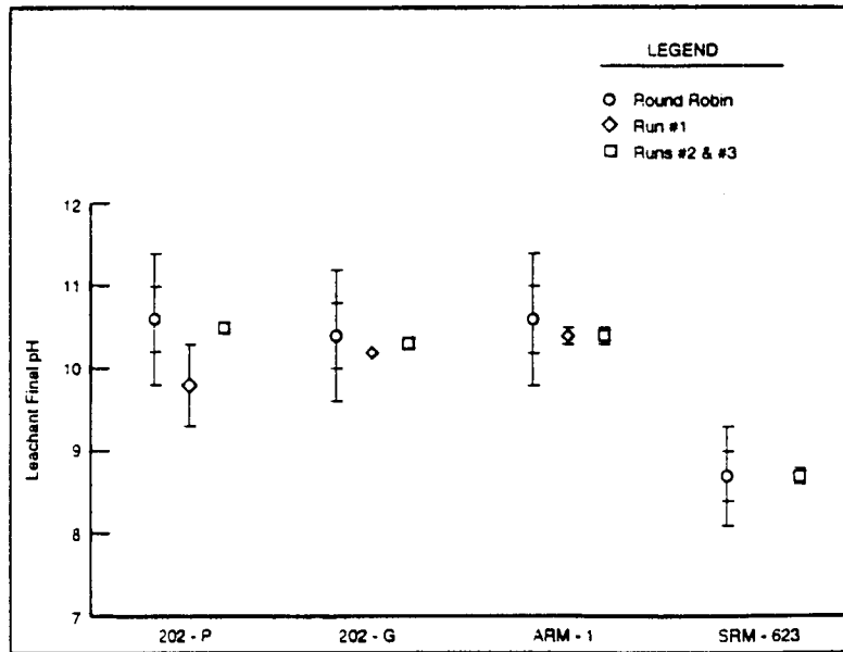
Figure 6. Leachant Final pH as a Function of Glass Type
