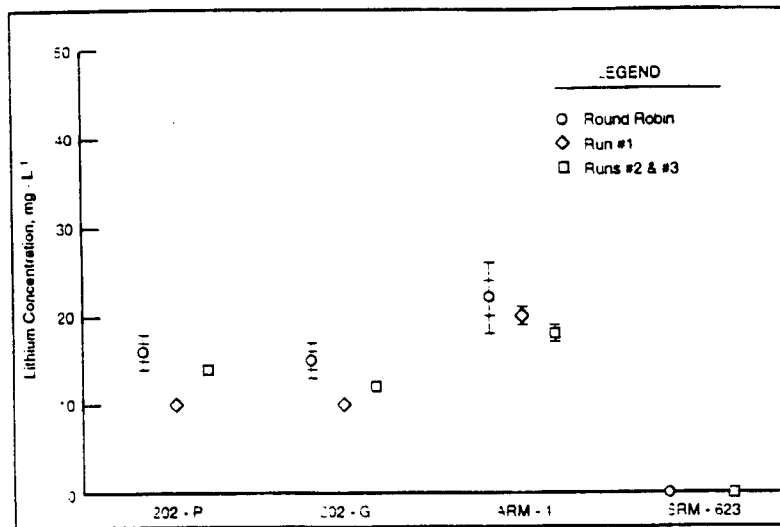
Figure 3. Release of Lithium as a Function of Glass Type
