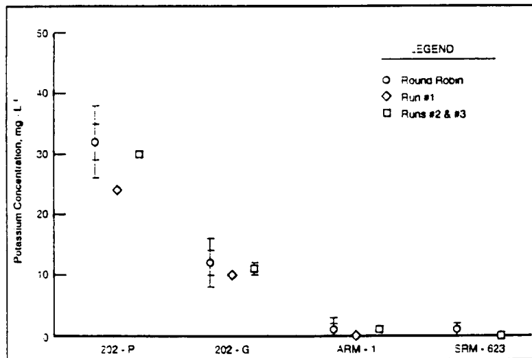
Figure 2. Release of Potassium as a Function of Glass Type
