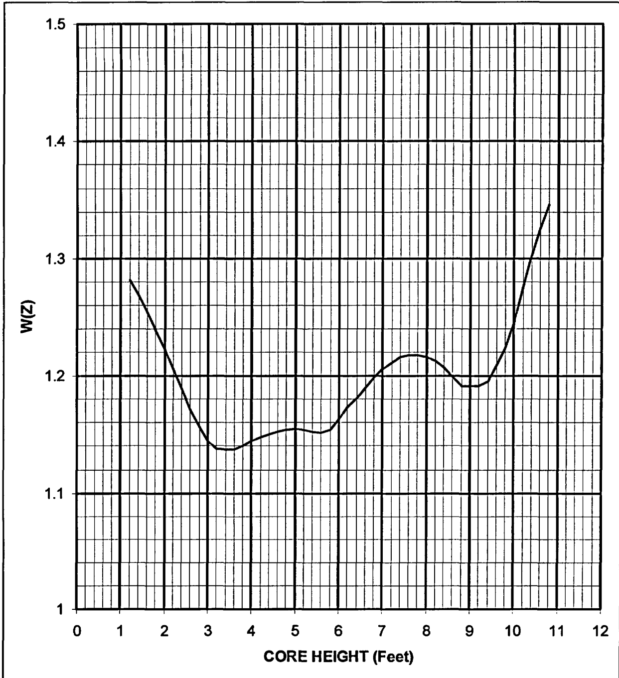
Figure 4.4: W(Z) Versus Core Height 19,000 MWD/MTU
