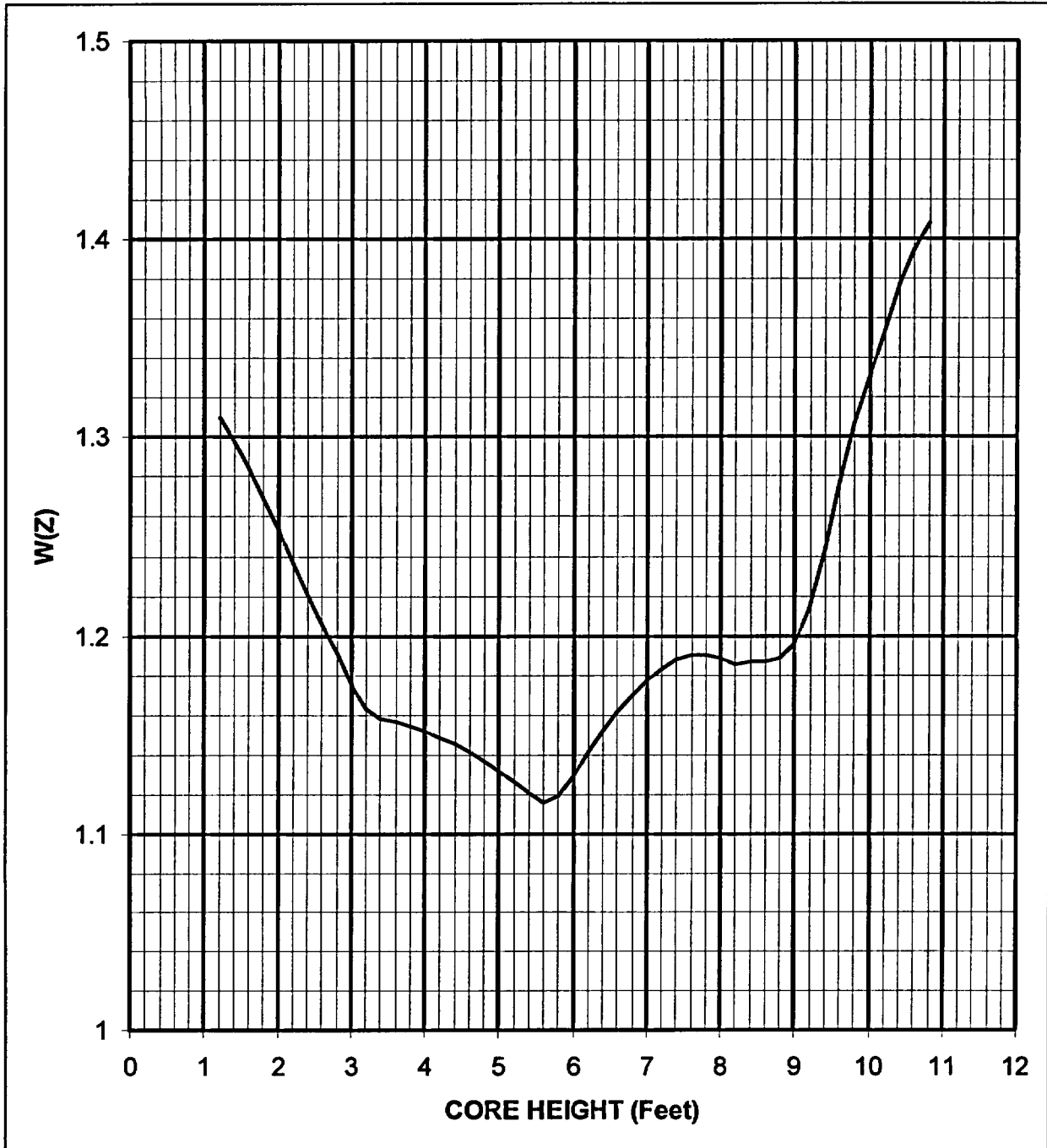
Figure 4.1: W(Z) Versus Core Height 150 MWD/MTU
