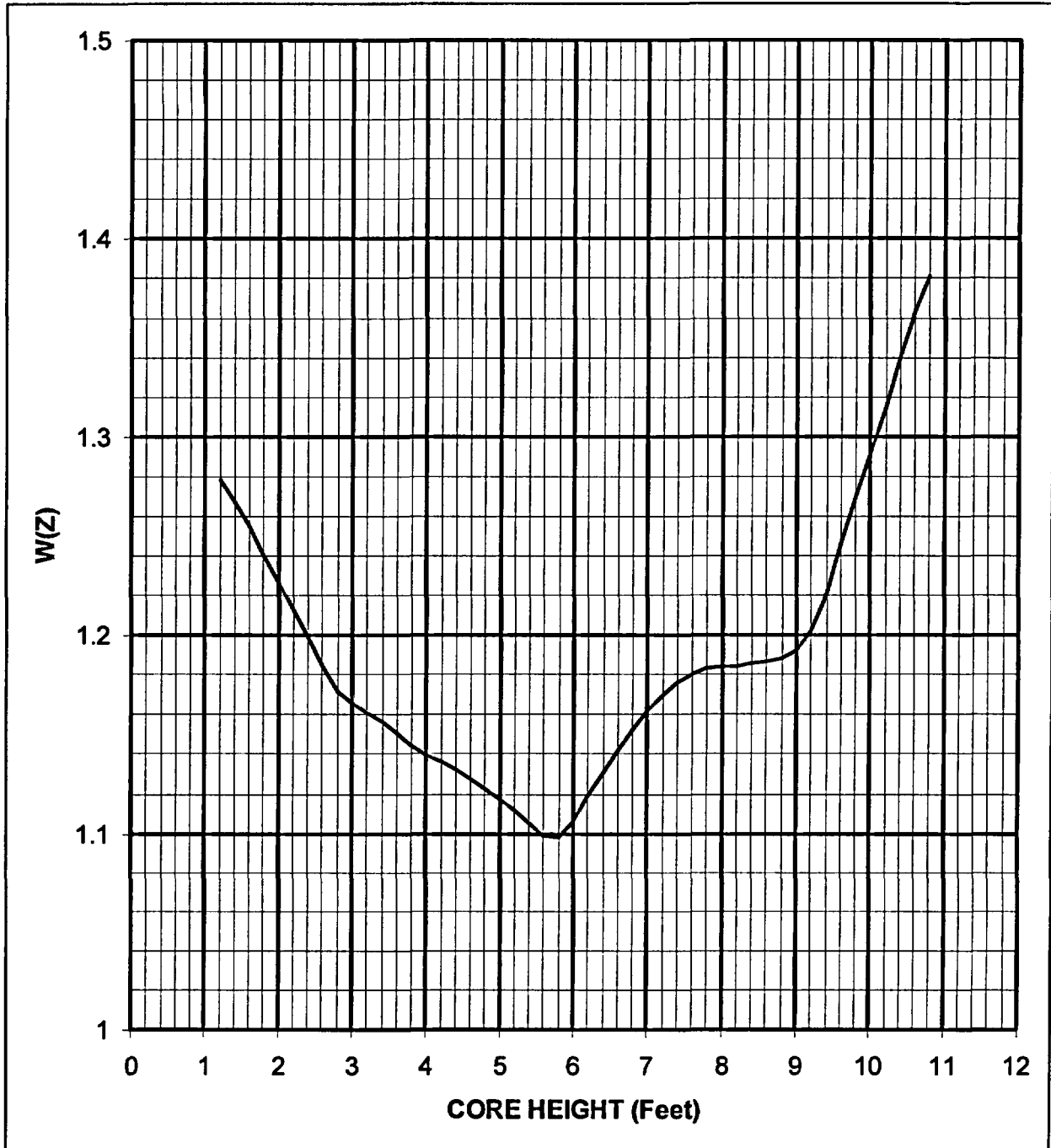
Figure 4.3: W(Z) Versus Core Height 10,000 MWD/MTU
