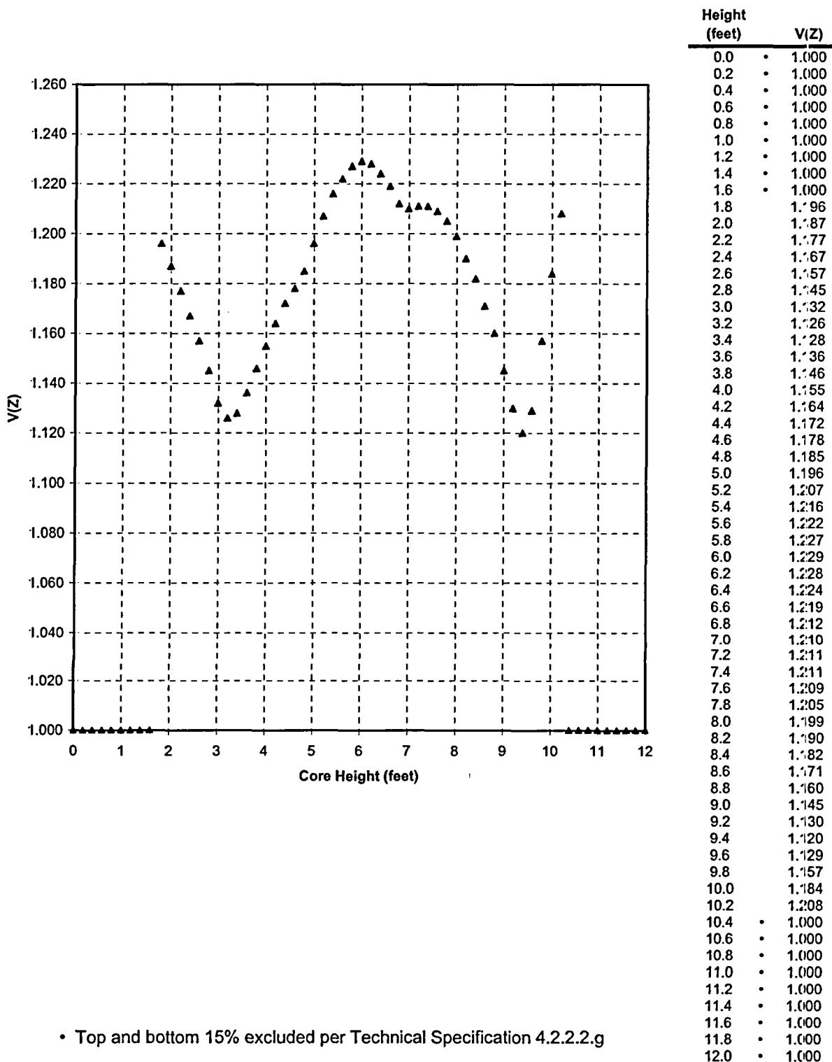
Figure 7 Cycle 14 V(Z) Versus Core Height 17500 MWD/MTU ≤ burnup < 18000 MWD/MTU
