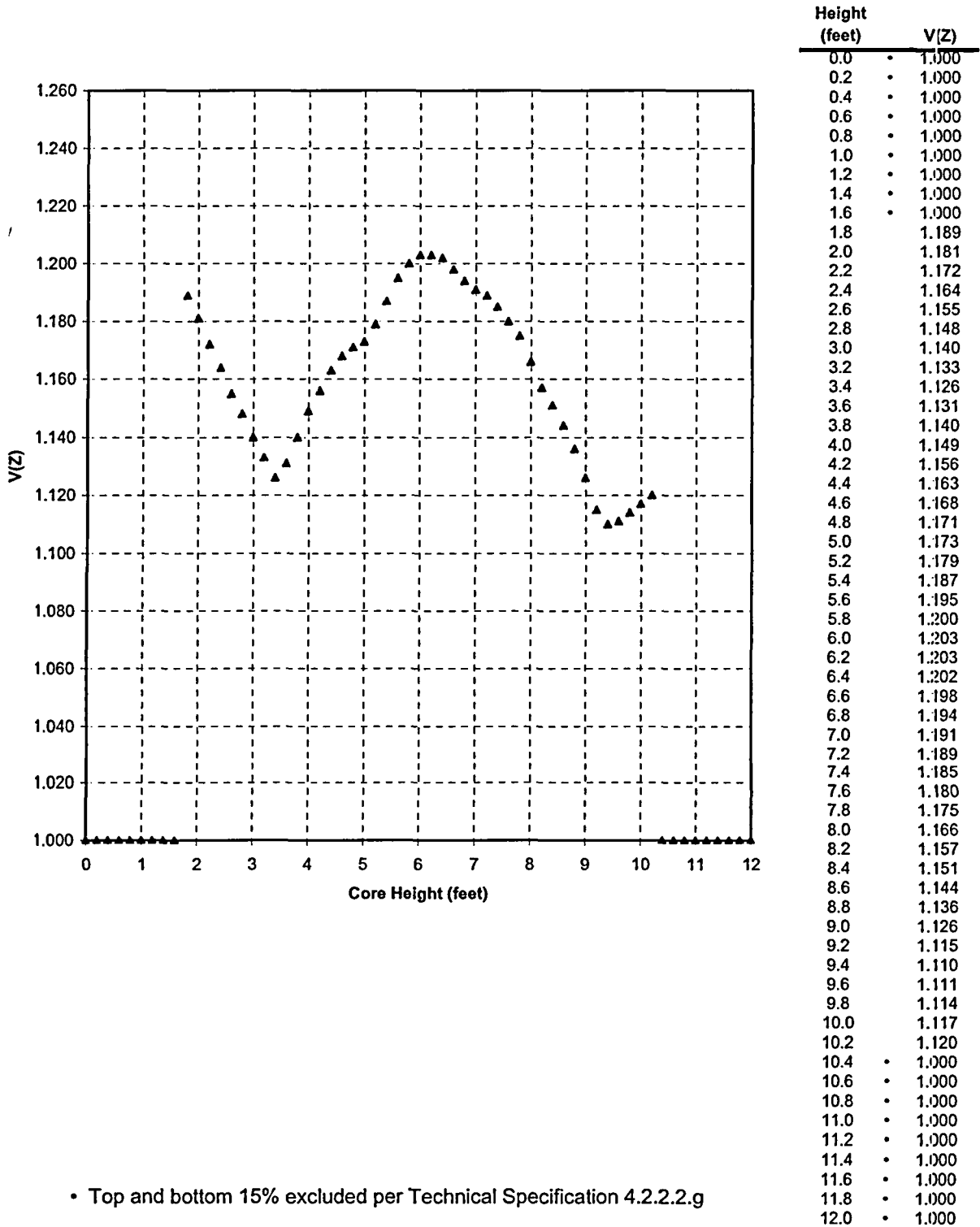
Figure 5 Cycle 14 V(Z) Versus Core Height 0 MWD/MTU ≤ burnup < 15000 MWD/MTU
