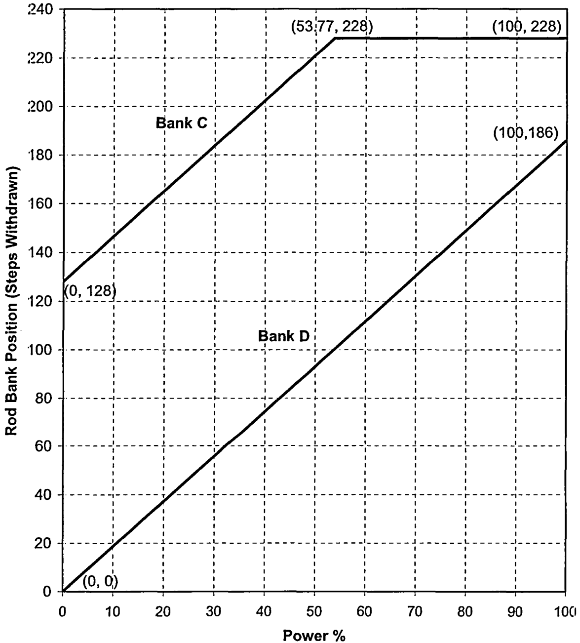
Figure 2 Rod Group Insertion Limits Versus Thermal Power (Three Loop Operation)
