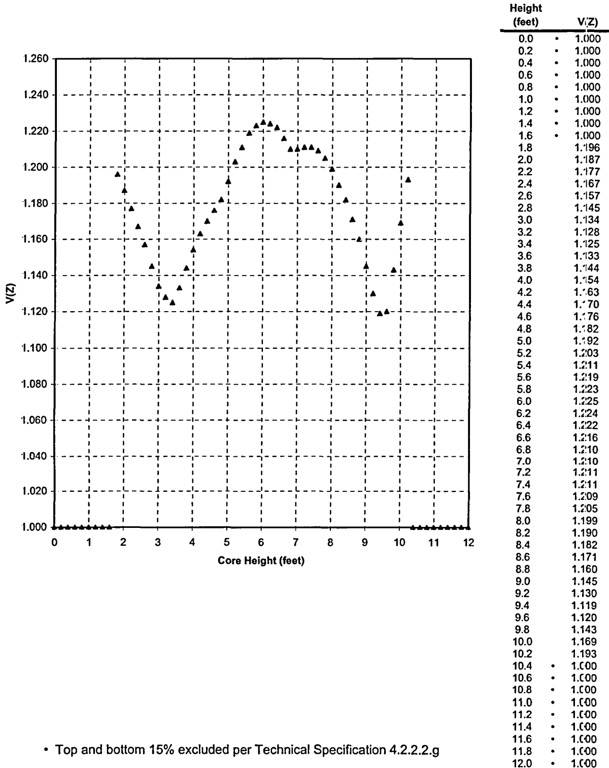
Figure 6 Cycle 14 V(Z) Versus Core Height 15000 MWD/MTU ≤ burnup < 17500 MWD/MTU
