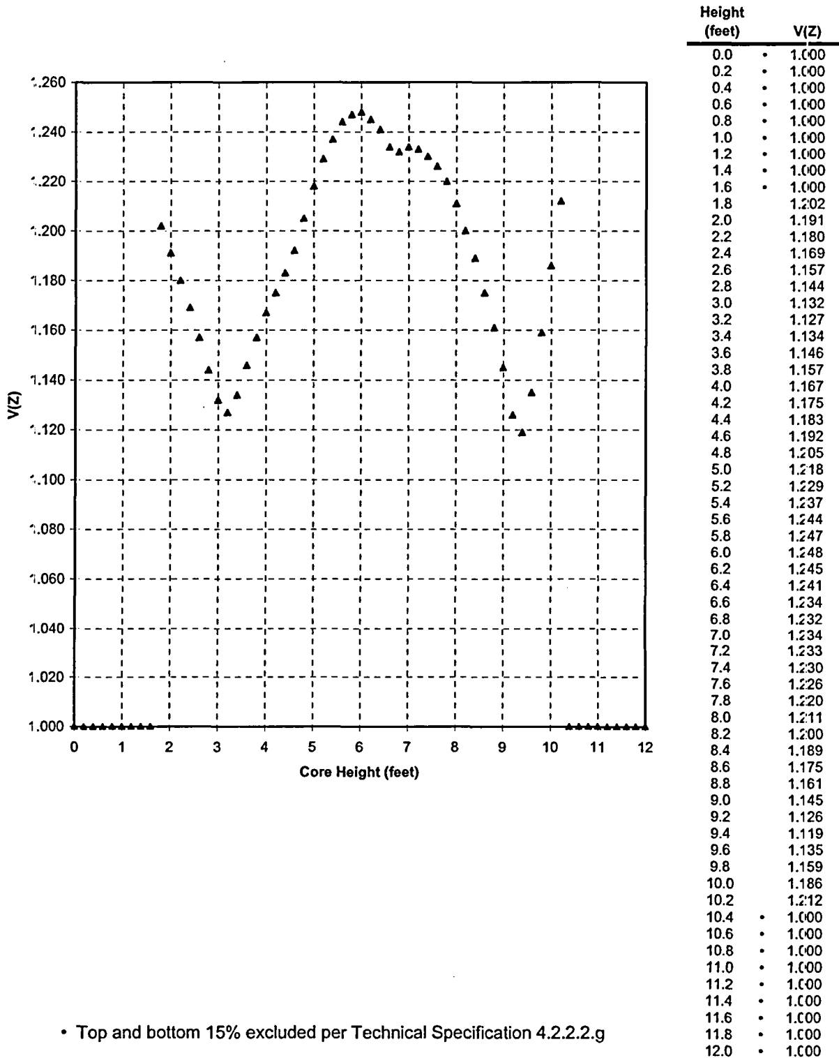
Figure 8 Cycle 14 V(Z) Versus Core Height 18000 MWD/MTU ≤ burnup ≤ 20491 MWD/MTU
