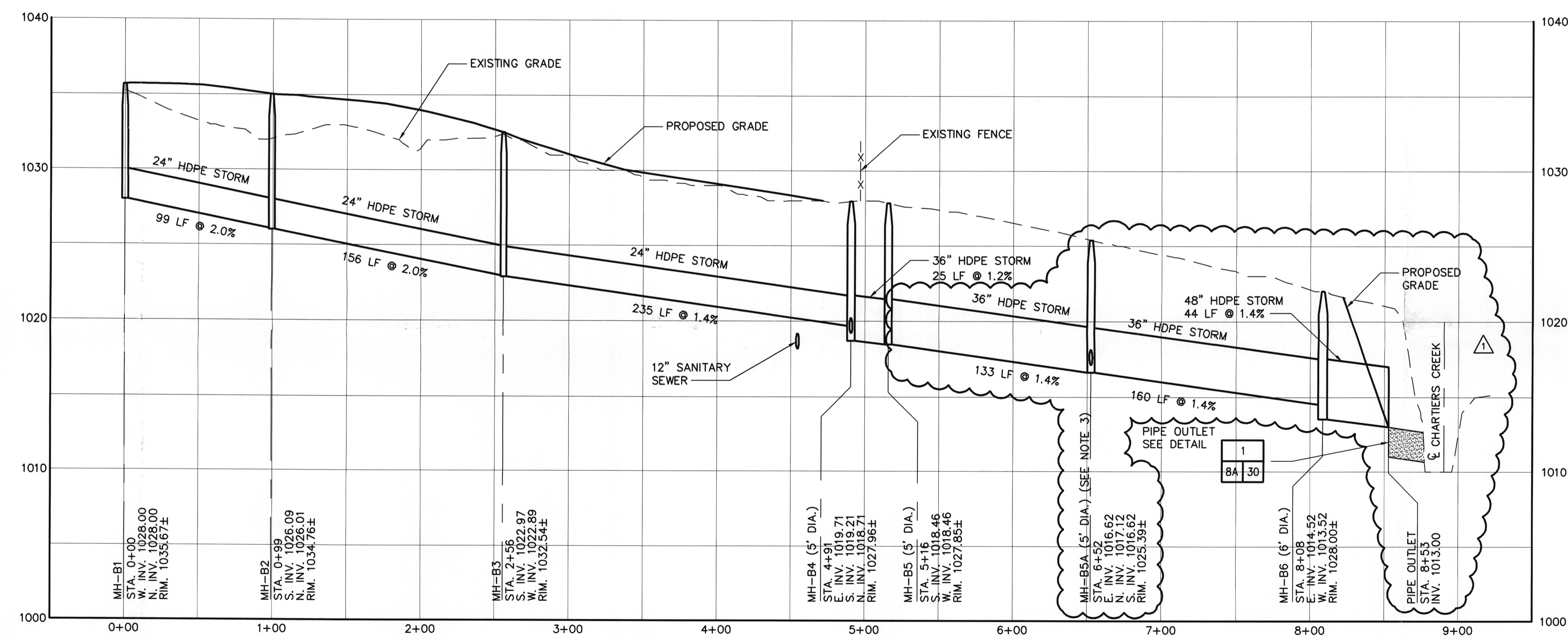
GRAVITY STORM PROFILE - "LINE B"
