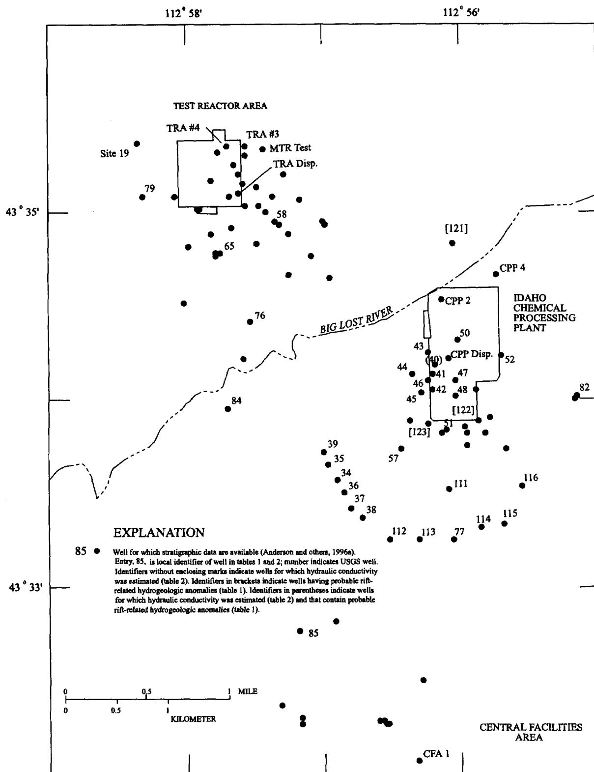
Figure 3. Locations of wells at and near the Idaho Chemical Processing Plant, Test Reactor Area, and Central Facilities Area for which stratigraphic data and estimates of hydraulic conductivity are available.
