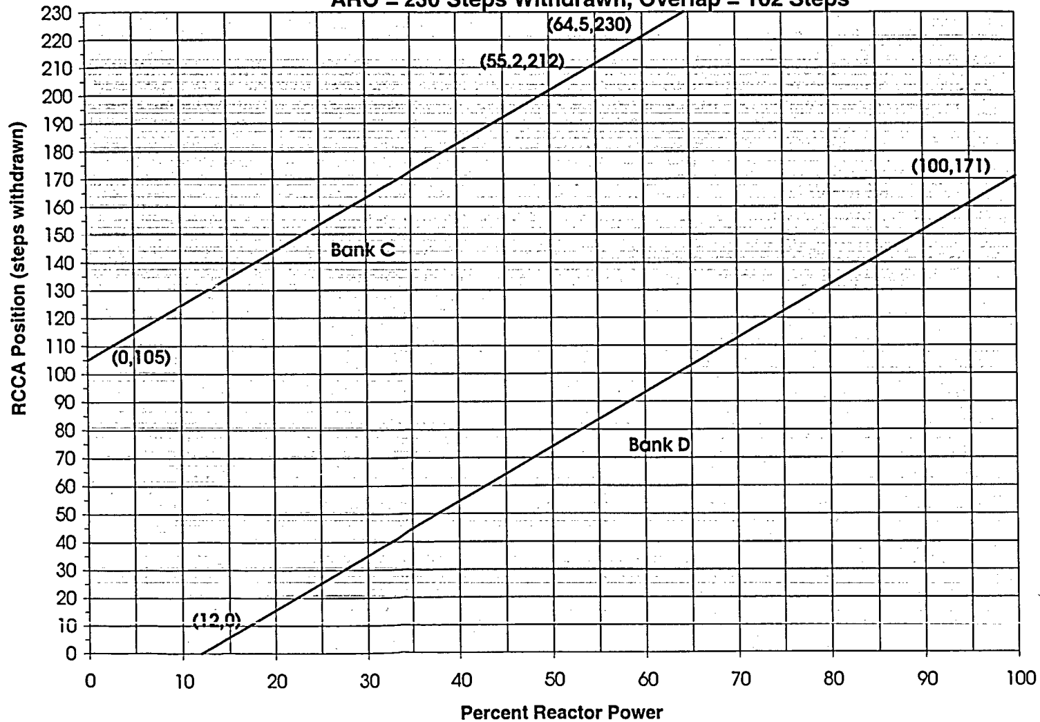
Figure 1 Turkey Point Unit 3 - Cycle 22 Rod Insertion Limits vs Thermal Power ARO = 230 Steps Withdrawn, Overlap = 102 Steps
