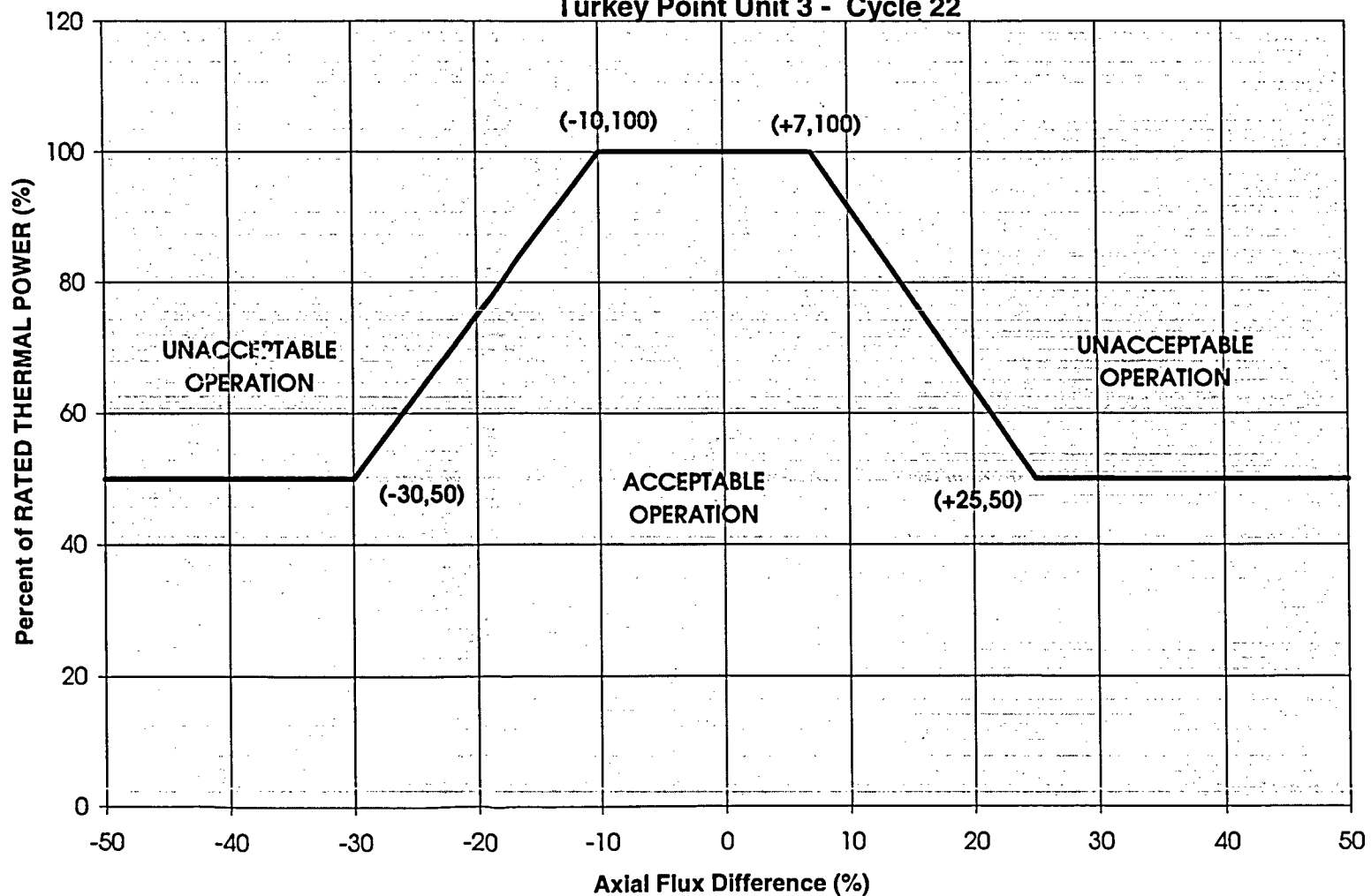
Figure 2 Axial Flux Difference as a Function of Rated Thermal Power Turkey Point Unit 3 - Cycle 22
