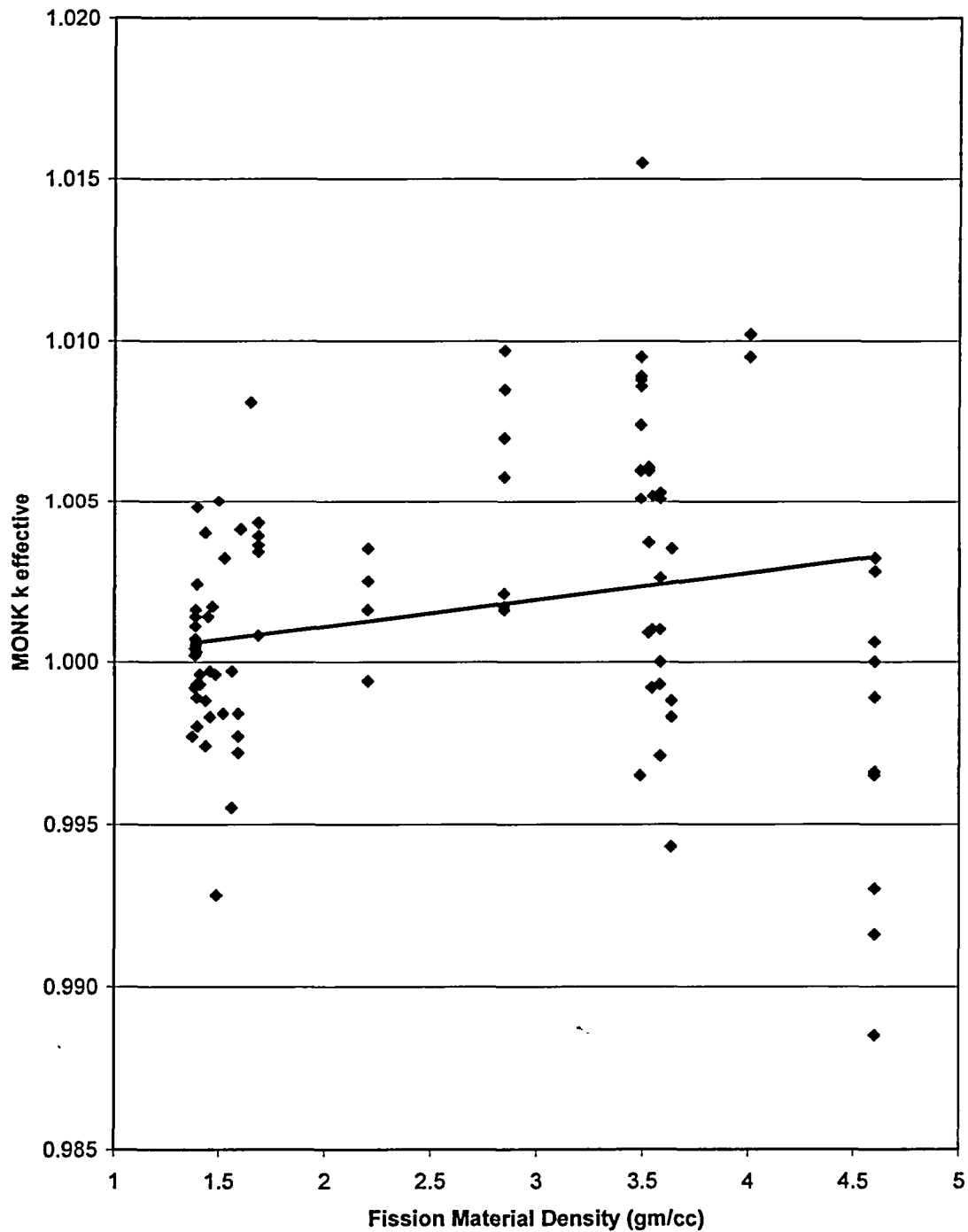
Figure 6-2 Plot of MONK k effective vs. Fission Material Density
