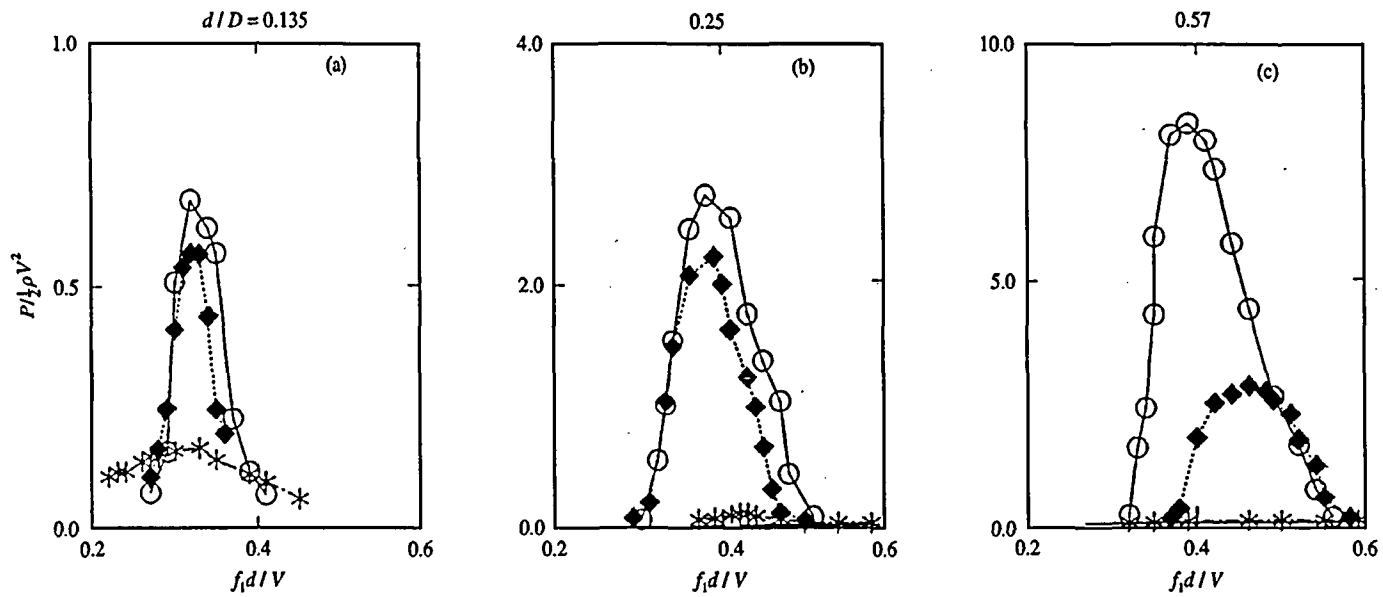
Figure 8. Comparison between the acoustic responses of single, tandem and coaxial side-branches for several values of diameter ratios: *, single; ♦, tandem; and O, coaxial branches. (a) d/D = 0.135 ; (b) d/D = 0.25 ; (c) d/D = 0.57 .
