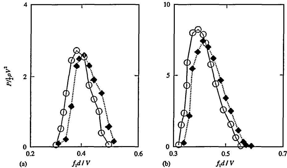
Figure 13. Effect of the upstream elbow on the resonance of two coaxial branches: O, without elbow; ◆, with elbow at \mathcal{L}/D = 3.8 ; (a) d/D = 0.25 ; (b) d/D = 0.57 .
