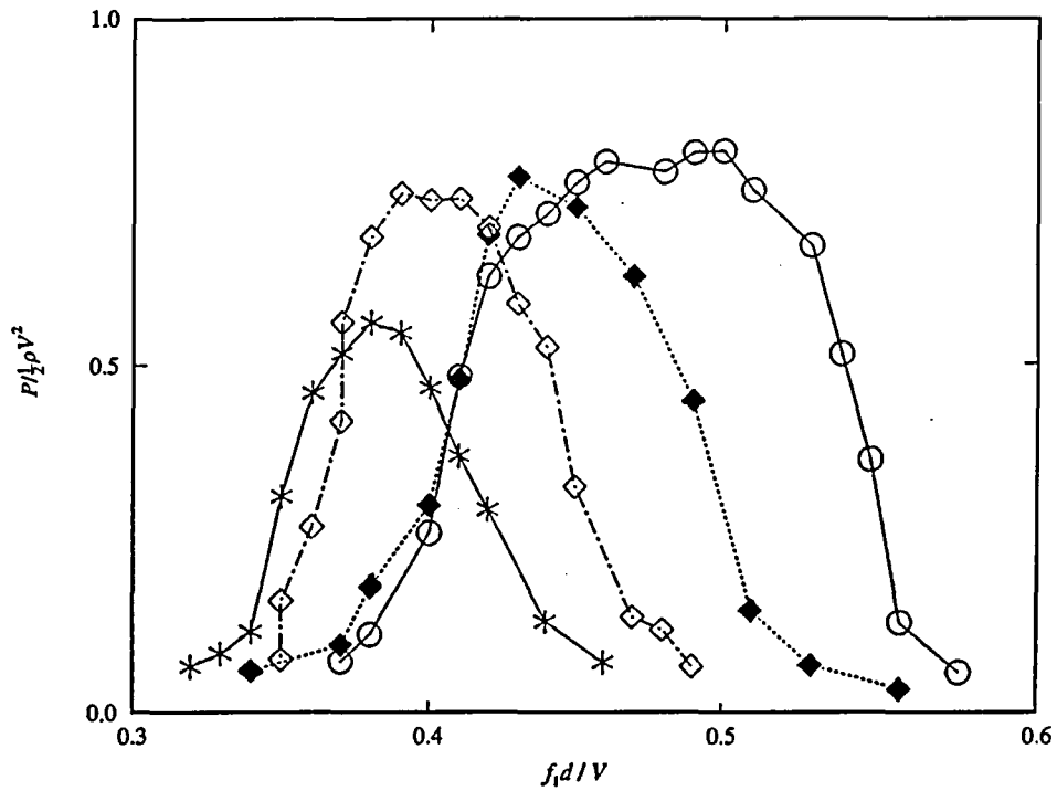
Figure 11. Pulsation amplitude versus Strouhal number for a single branch located at the outer side of, but at different distances ( \mathcal{L} ), from an upstream elbow; d/D = 0.25 , f_1 = 326 Hz, P_s = 3 bar. O, \mathcal{L}/D = 1.8 ; \blacklozenge , \mathcal{L}/D = 6.2 ; \diamond , \mathcal{L}/D = 10 ; *, \mathcal{L}/D = \infty .
