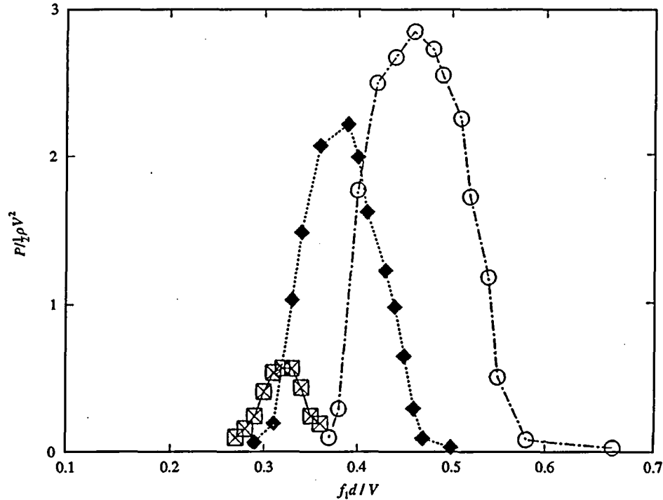
Figure 9. Effect of the diameter ratio of tandem branches on the critical Strouhal number of the onset of resonance. \square , d/D = 0.135 ; \blacklozenge , 0.25 ; \circ , 0.75 .
