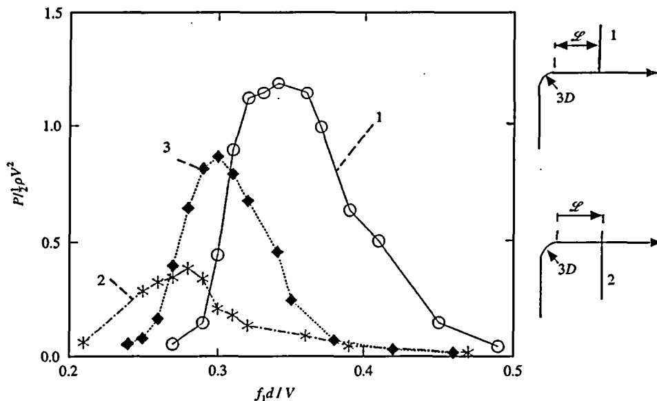
Figure 10. Effect of the upstream elbow on the acoustic response of a single branch; O, branch at the outer side of the elbow; *, at the inner side; ♦, no elbow. d/D = 0.135 , f_1 = 490 Hz, \mathcal{L}/D = 1.85 , P_s = 3 bar.
