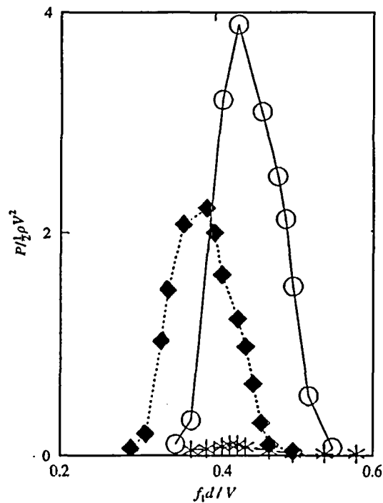
Figure 12. Effect of the upstream elbow on the resonance of two tandem branches installed at its outer side; d/D = 0.25 ; *, single branch without elbow; \blacklozenge , tandem branches without elbow; O, tandem branches with elbow at \mathcal{L}/D = 3.75 .
