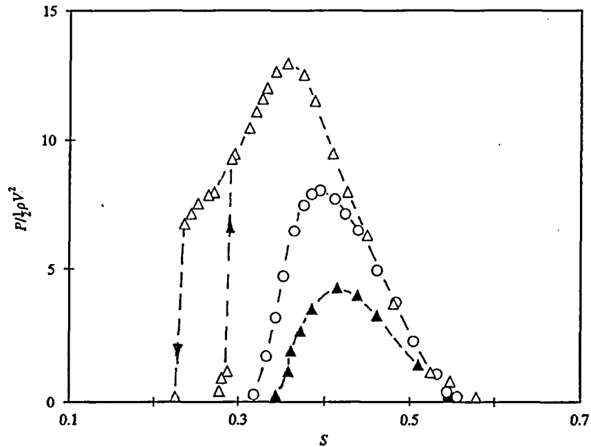
Figure 7. Acoustic response of the coaxial branches showing the effect of the branch length (i.e., the effect of acoustic attenuation). \Delta , L = 61 cm, f_1 = 132.5 Hz, P_s = 3.5 bar; \circ , L = 110.5 cm, f_1 = 72.5 Hz, P_s = 4 bar; \blacktriangle , L = 158.5 cm, f_1 = 50 Hz, P_s = 4 bar.
