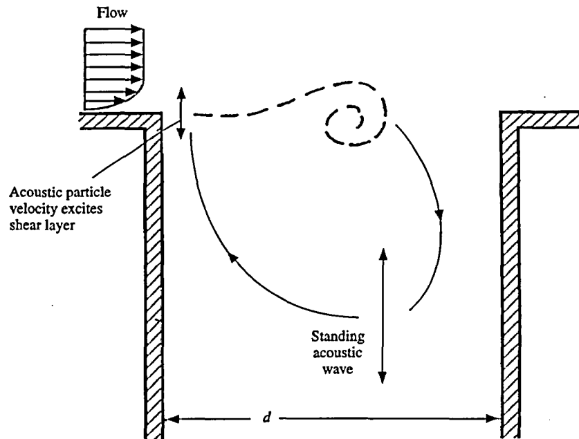
Figure 1. Feedback mechanism of flow-excited acoustic resonances of closed side-branches (the fluid-resonant mechanism).
