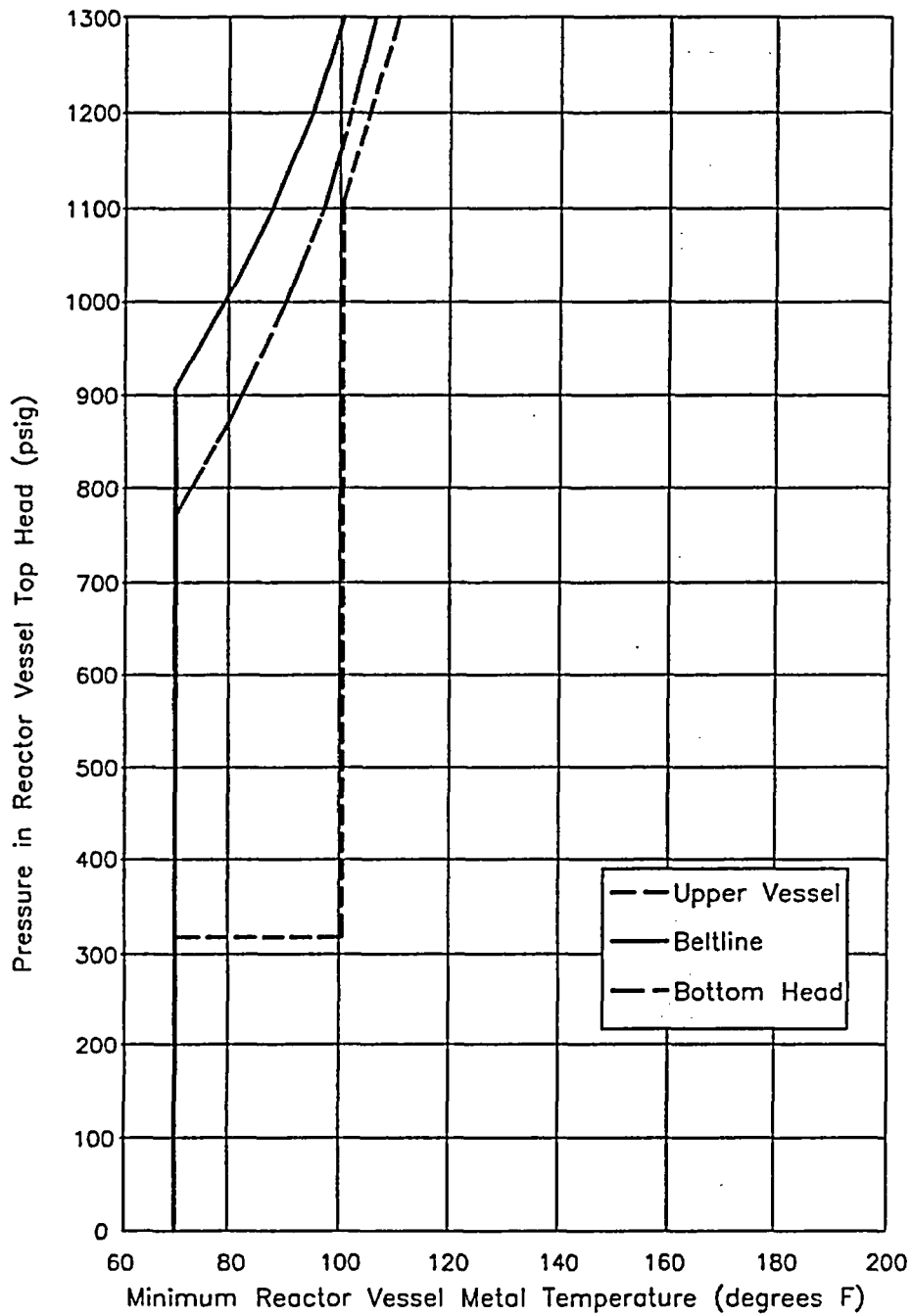
Figure 3.4.10-1 System Hydrotest Limit with Fuel in Vessel for 30.2 EPY (Curve A)
