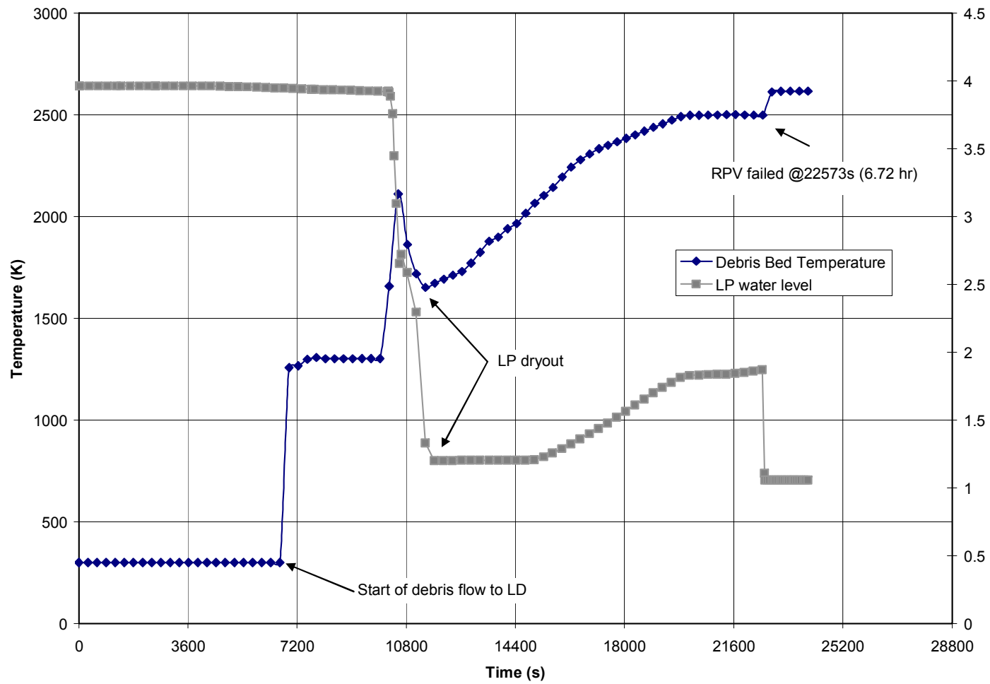
Graph illustrates initial cooling of corium displaced to LP followed by debris bed heatup as LP dries out
