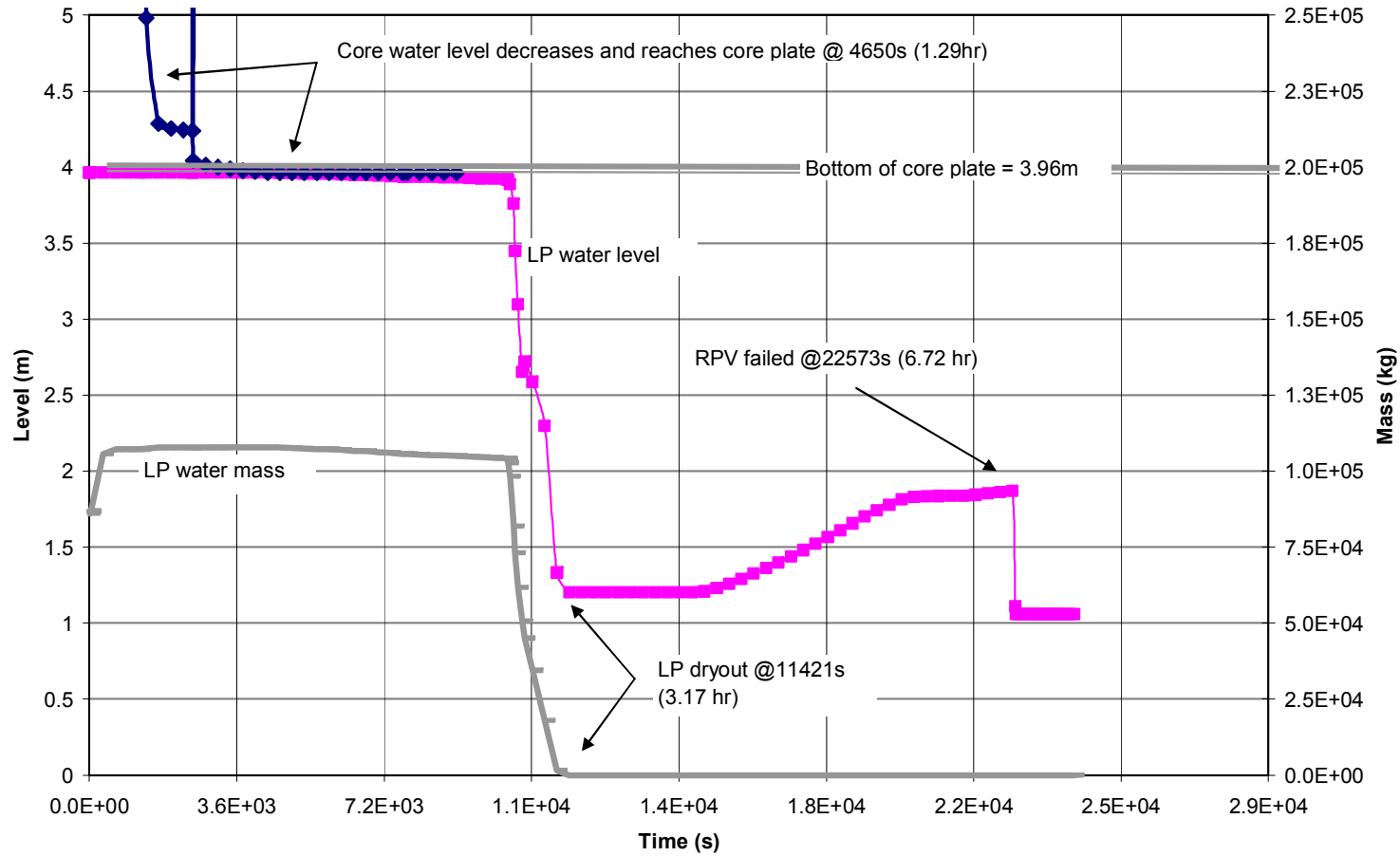
Graph illustrates time between water level reaching core support plate and lower plenum dryout is about 1.9 hrs
