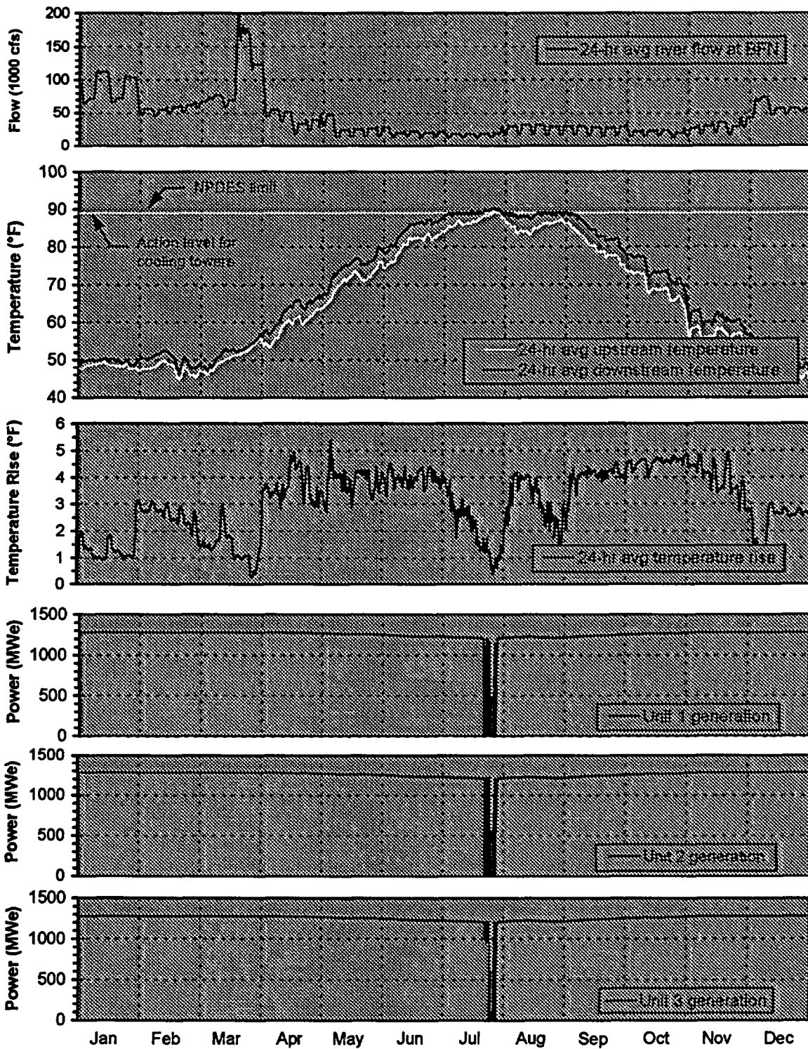
Figure 26. BFN Operation for 1993
