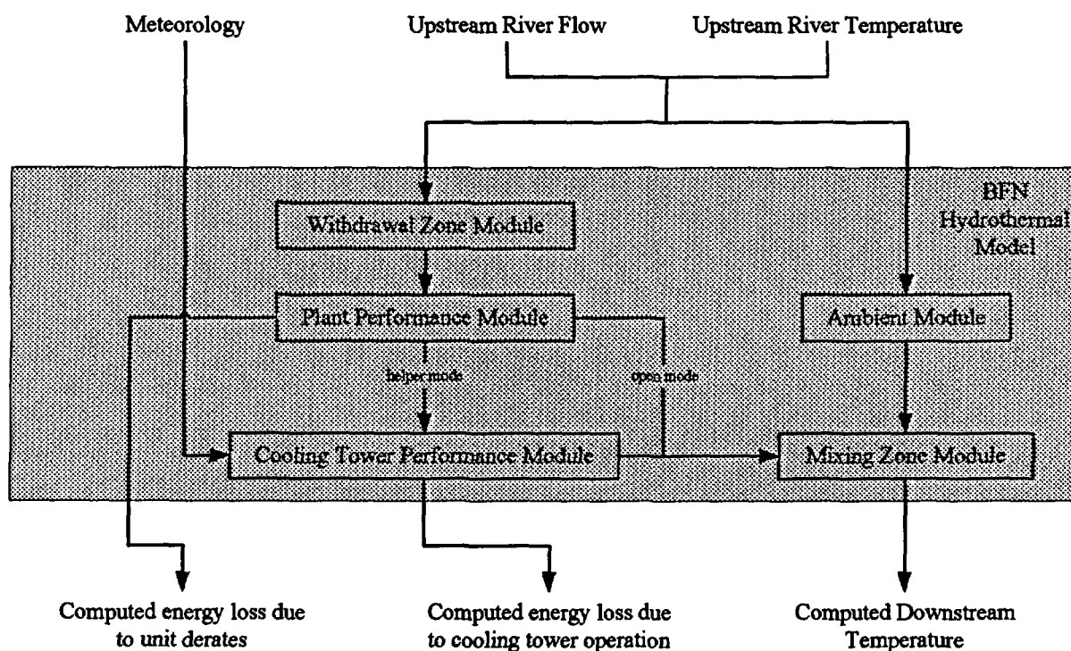
Figure 8. BFN Hydrothermal Model
