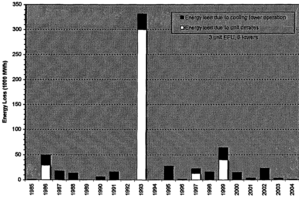
Figure 25. Baseline (Case 0) Results for BFN Simulations
