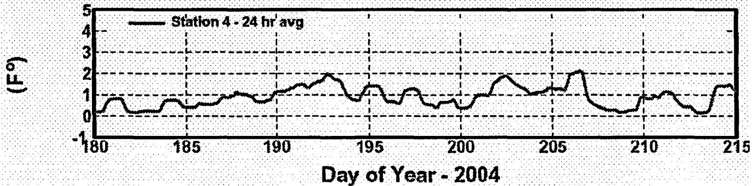
Figure 24. Computed vs. Measured Temperatures for Two-Unit Operation for Summer 2004
