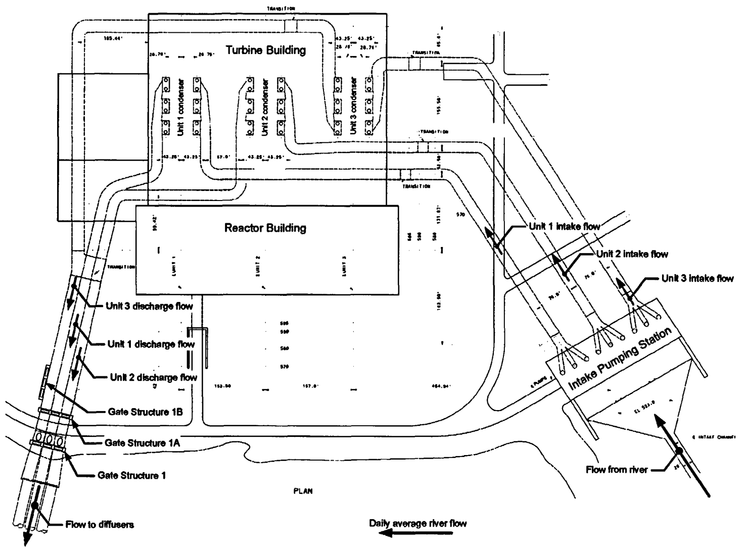
Figure 2. BFN CCW Intake and Discharge Conduits
