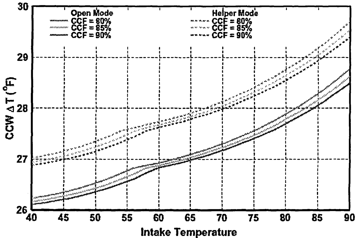
Figure 29. Effect of Condenser Cleanliness Factor on Condenser Temperature Rise
