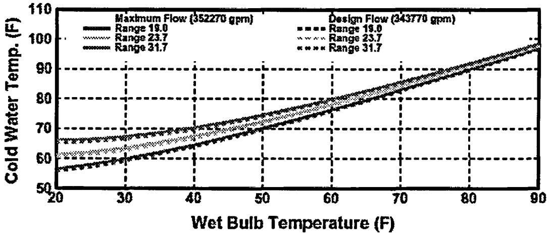
Figure 17. BFN Cooling Tower Performance Curves
