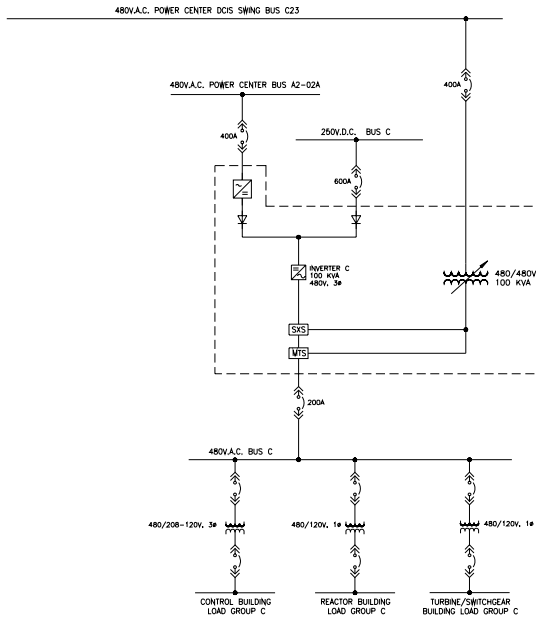
NON CLASS 1E UNINTERRUPTIBLE POWER SUPPLY
