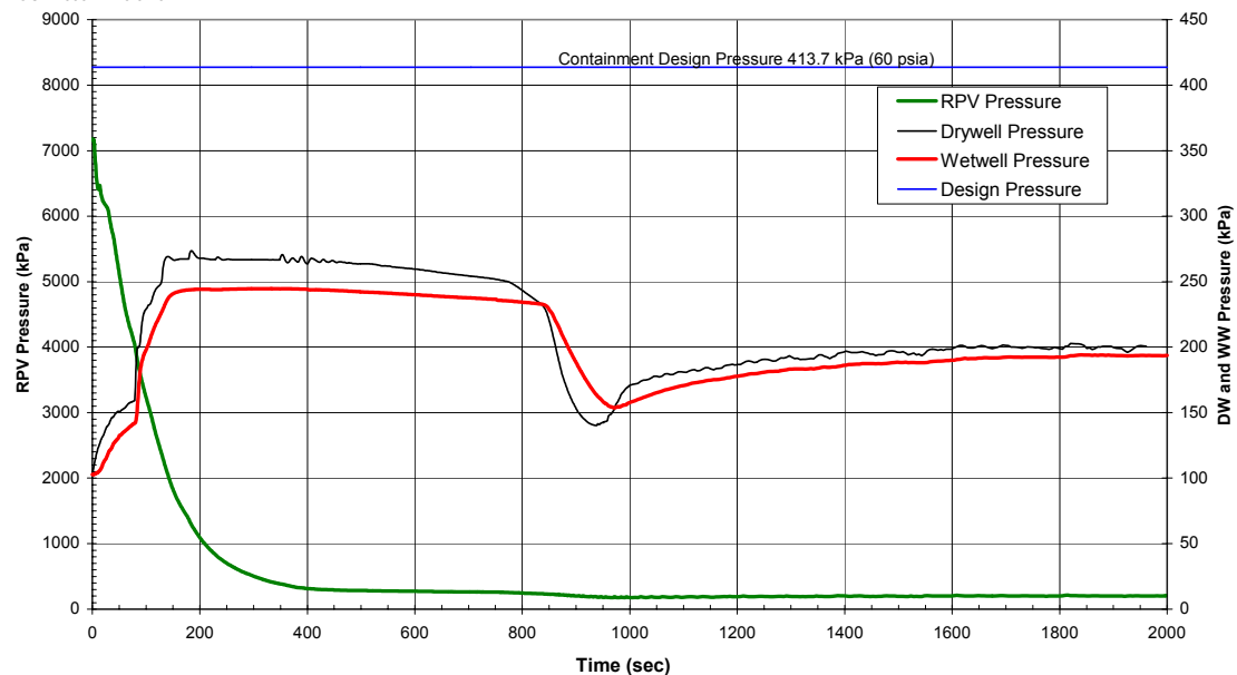
Figure 6.3-26. System Pressures, Bottom Drain Line Break, 1 GDSCS Valve Failure
