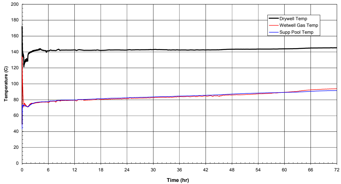
Figure 6.2-13. Feedwater Line Break (Bounding Case) — Containment Temperatures
