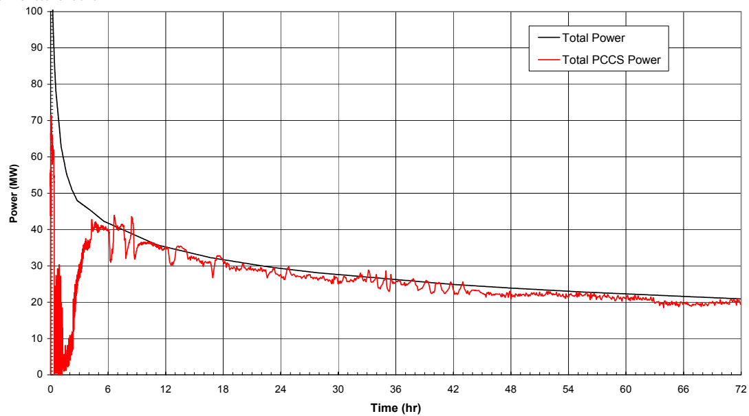
Figure 6.2-14. Feedwater Line Break (Bounding Case) — PCCS Heat Removal versus Decay Heat
