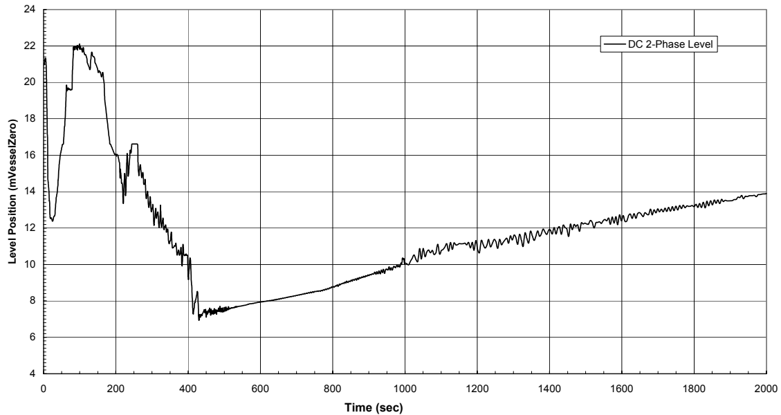
Figure 6.3-33. Downcomer Water Level, GDCS Injection Line Break, 1 GDCS Valve Failure
