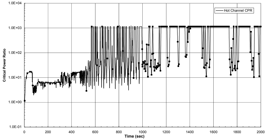
Figure 6.3-7. MCPR, Feedwater Line Break, 1 GDSCS Valve Failure
