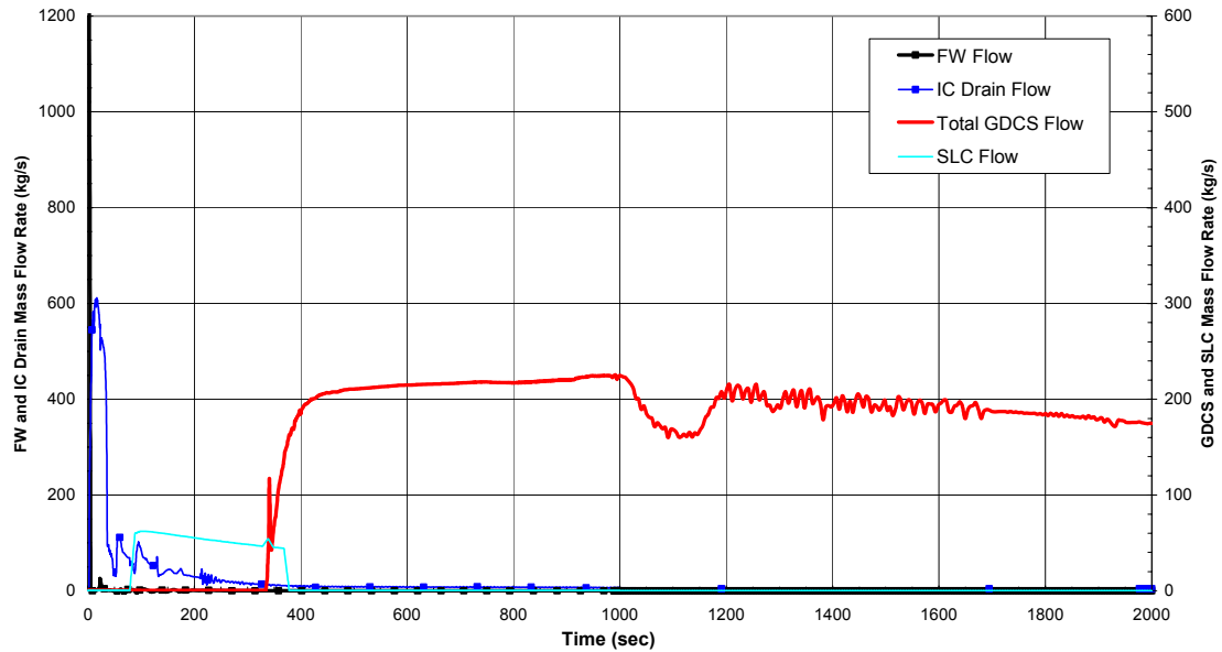
Figure 6.3-37. Flows Into Vessel, GDCS Injection Line Break, 1 GDCS Valve Failure
