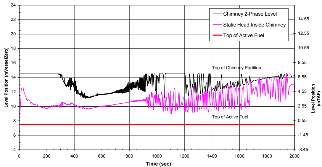
Figure 6.3-32. Chimney Water Level, GDCS Injection Line Break, 1 GDCS Valve Failure
