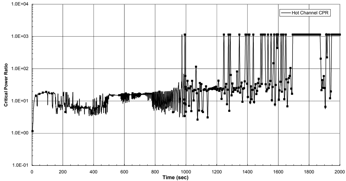
Figure 6.3-31. MCPR, GDCS Injection Line Break, 1 GDCS Valve Failure
