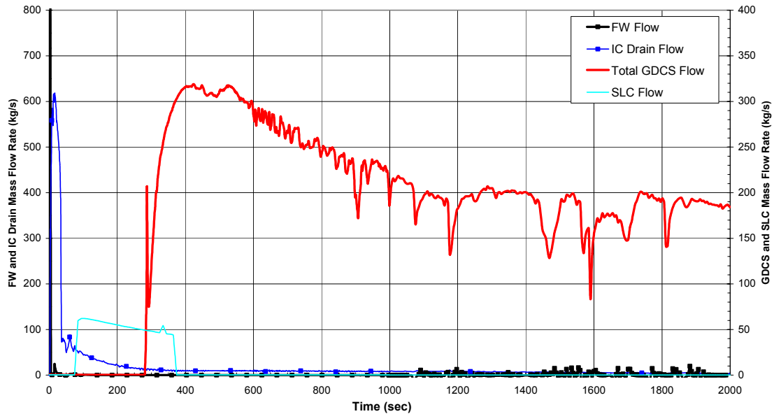
Figure 6.3-13. Flows Into Vessel, Feedwater Line Break, 1 GDCS Valve Failure
