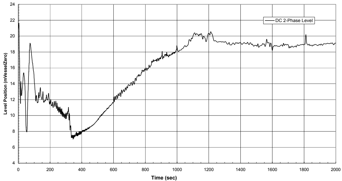
Figure 6.3-9. Downcomer Water Level, Feedwater Line Break, 1 GDSCS Valve Failure
