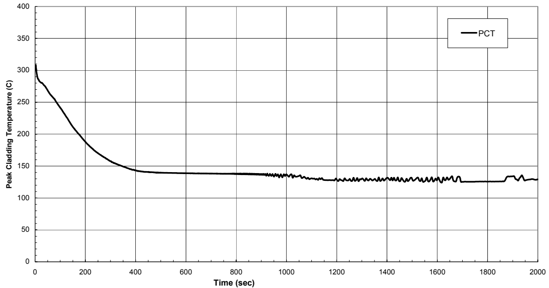
Figure 6.3-38. PCT, GDCS Injection Line Break, 1 GDCS Valve Failure
