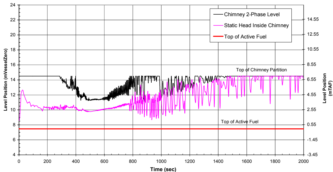
Figure 6.3-24. Chimney Water Level, Bottom Drain Line Break, 1 GDSCS Valve Failure
