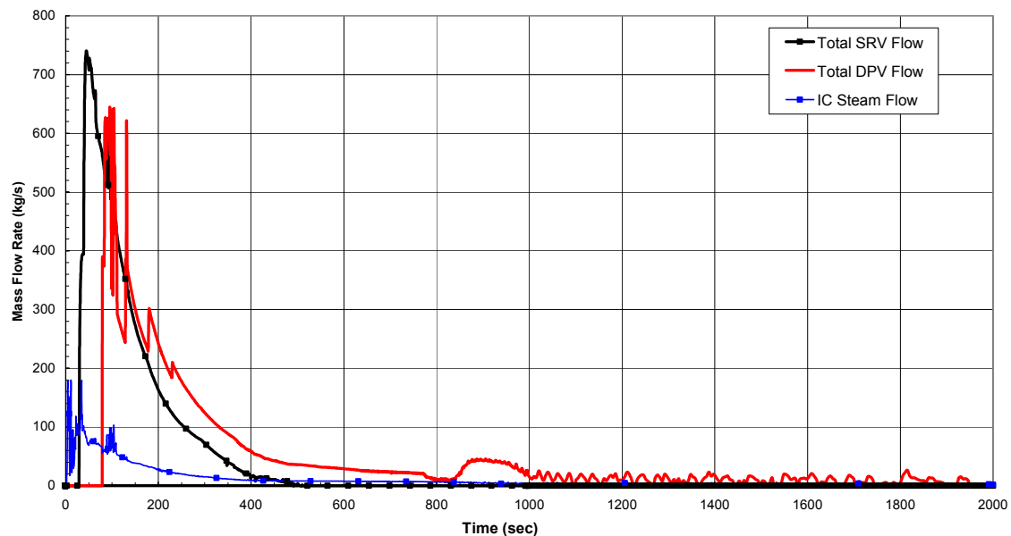
Figure 6.3-28. ADS Flow, Bottom Drain Line Break, 1 GDACS Valve Failure
