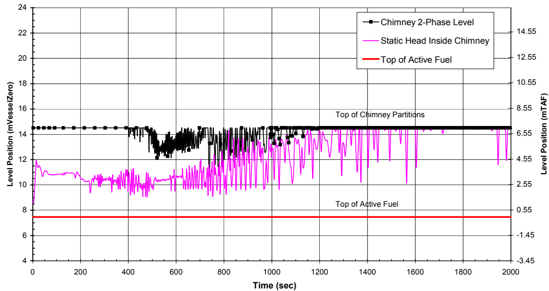
Figure 6.3-16. Chimney Water Level, Inside Steam Line Break, 1 GDCS Valve Failure
