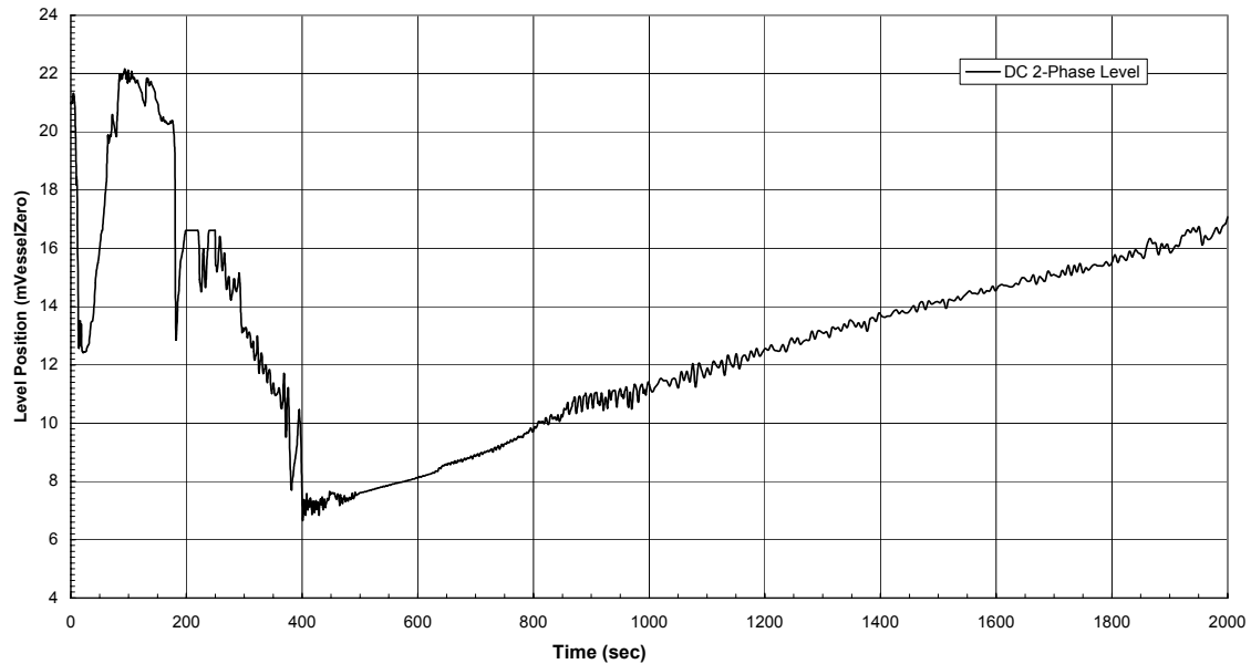
Figure 6.3-25. Downcomer Water Level, Bottom Drain Line Break, 1 GDSCS Valve Failure
