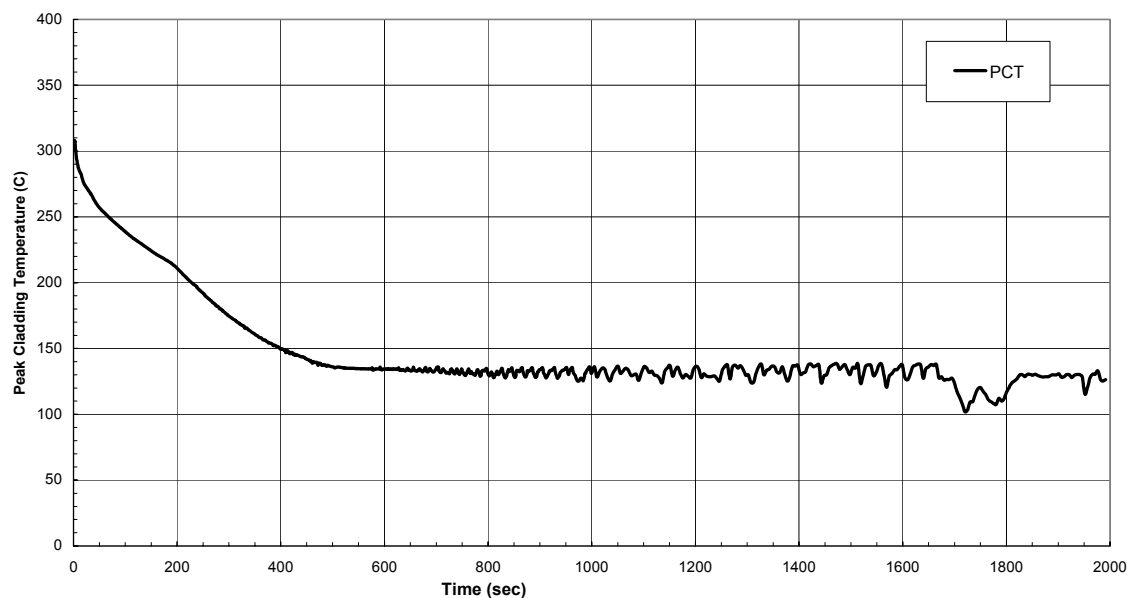
Figure 6.3-22. PCT, Inside Steam Line Break, 1 GDCS Valve Failure
