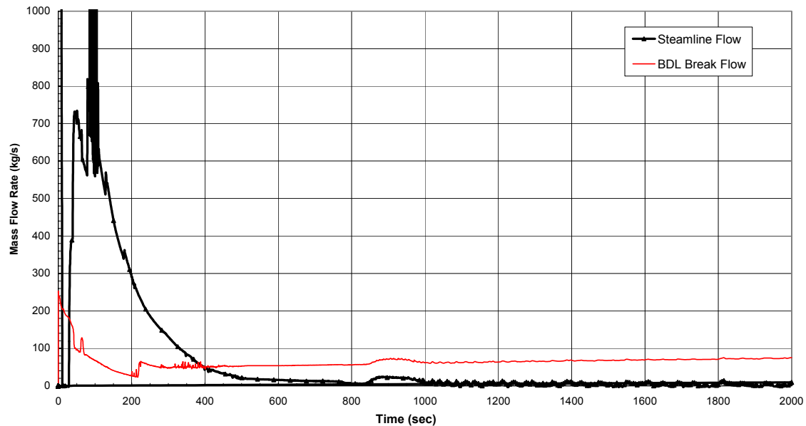
Figure 6.3-27. Steam Line and Break Flow, Bottom Drain Line Break, 1 GDACS Valve Failure
