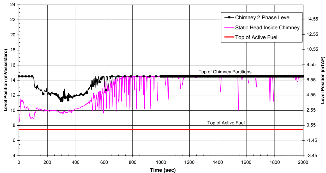
Figure 6.3-8. Chimney Water Level, Feedwater Line Break, 1 GDSCS Valve Failure
