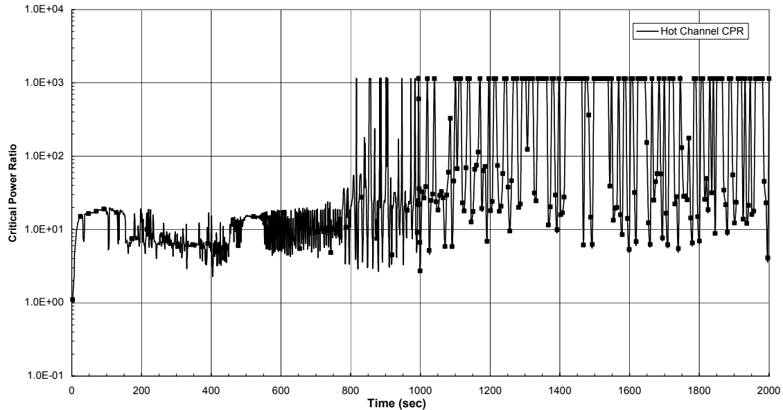
Figure 6.3-23. MCPR, Bottom Drain Line Break, 1 GDSCS Valve Failure
