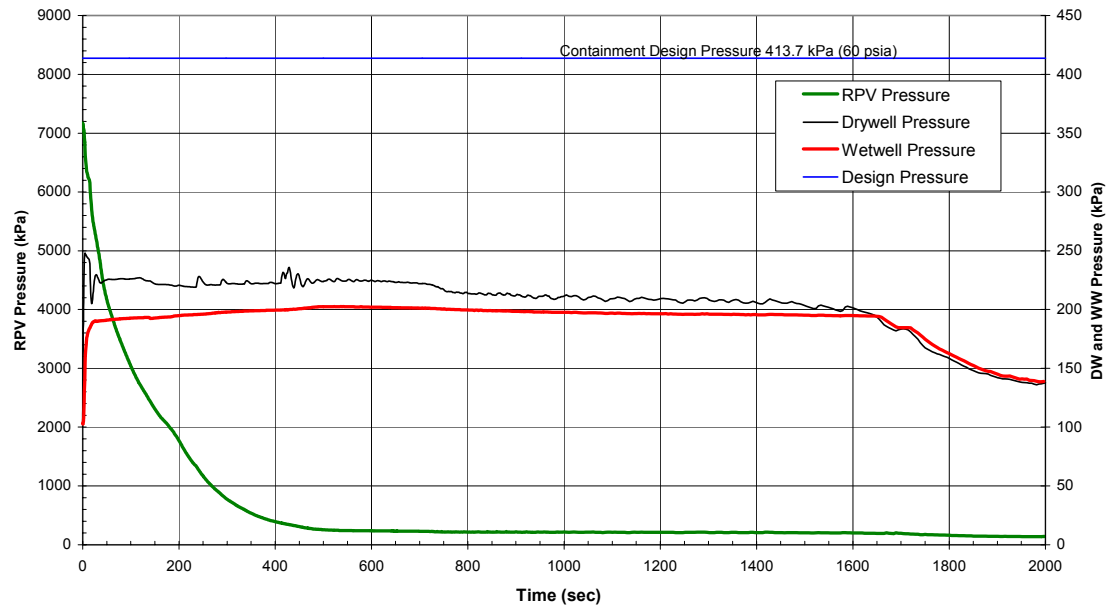
Figure 6.3-18. System Pressures, Inside Steam Line Break, 1 GDSC Valve Failure
