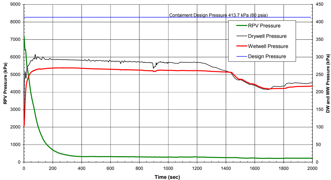
Figure 6.3-10. System Pressures, Feedwater Line Break, 1 GDSCS Valve Failure
