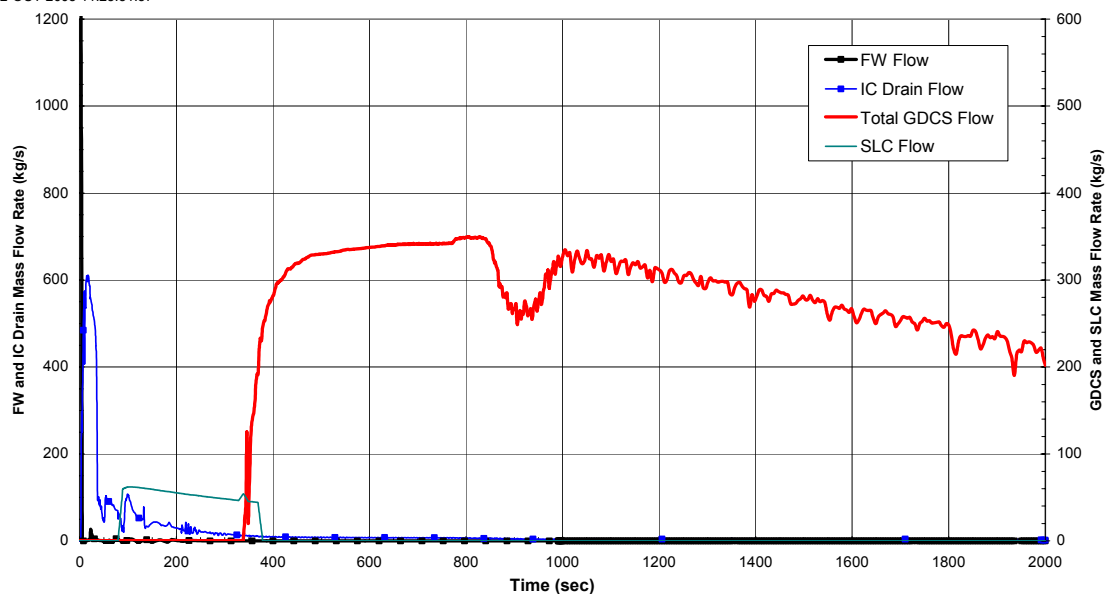
Figure 6.3-29. Flows Into Vessel, Bottom Drain Line Break, 1 GDCS Valve Failure
