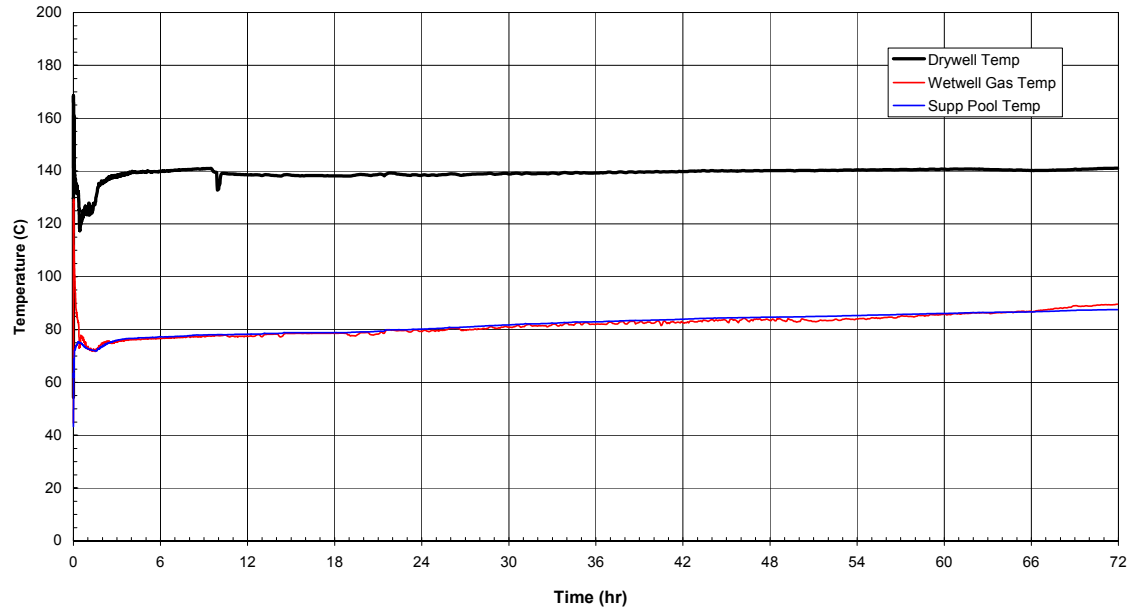
Figure 6.2-10. Feedwater Line Break (Nominal Case) — Containment Temperatures
