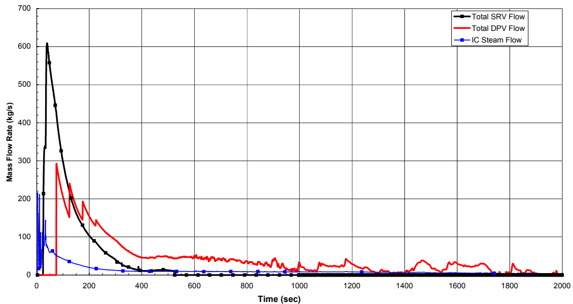
Figure 6.3-12. ADS Flow, Feedwater Line Break, 1 GDCS Valve Failure
