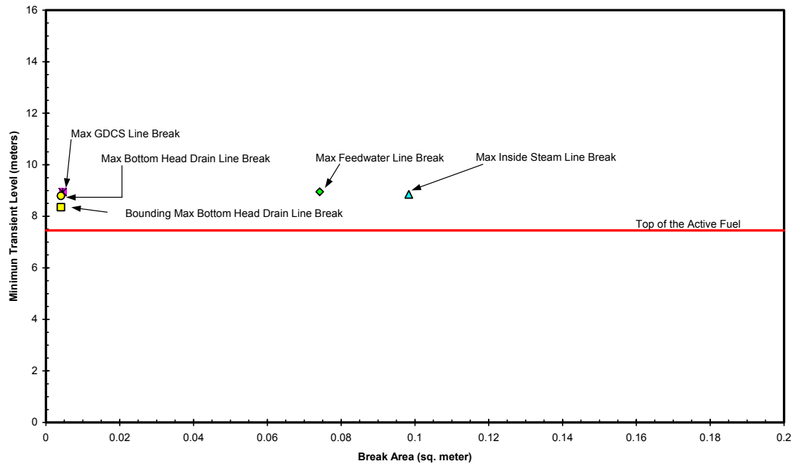
Figure 6.3-6. Minimum Chimney Water Level vs. Break Area
