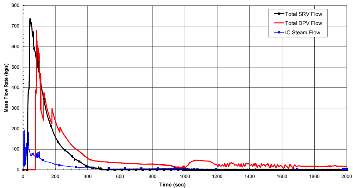
Figure 6.3-36. ADS Flow, GDCS Injection Line Break, 1 GDCS Valve Failure
