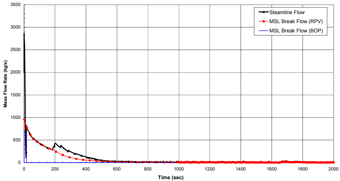
Figure 6.3-19. Steam Line and Break Flow, Inside Steam Line Break, 1 GDCS Valve Failure
