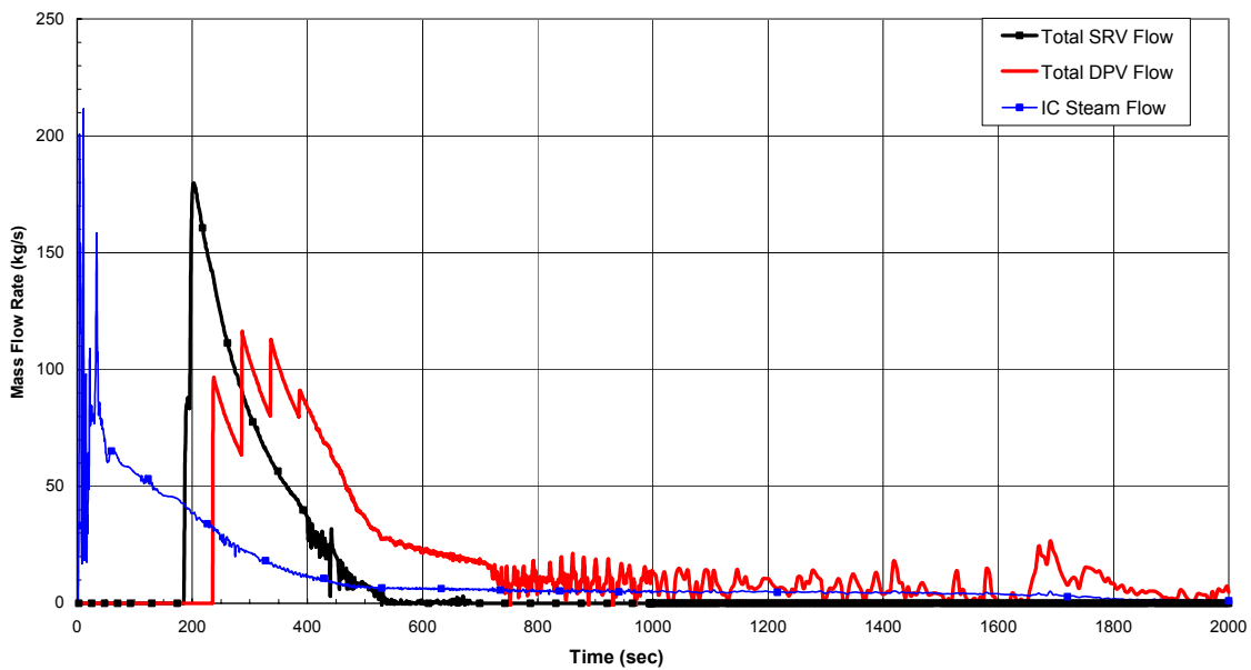
Figure 6.3-20. ADS Flow, Inside Steam Line Break, 1 GDCS Valve Failure
