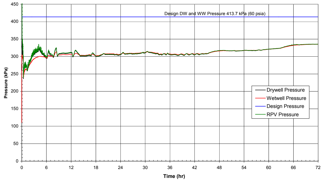
Figure 6.2-12. Feedwater Line Break (Bounding Case) — Containment Pressures
