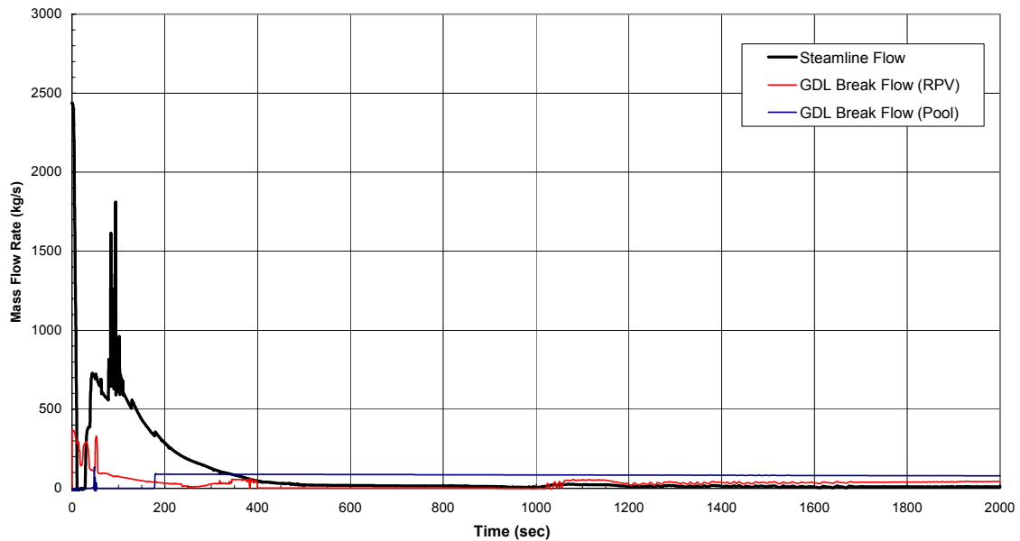
Figure 6.3-35. Steam Line and Break Flow, GDCS Injection Line Break, 1 GDCS Valve Failure
