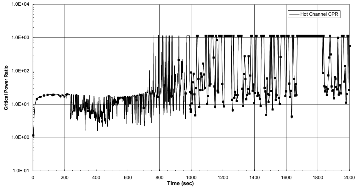
Figure 6.3-15. MCPR, Inside Steam Line Break, 1 GDCS Valve Failure
