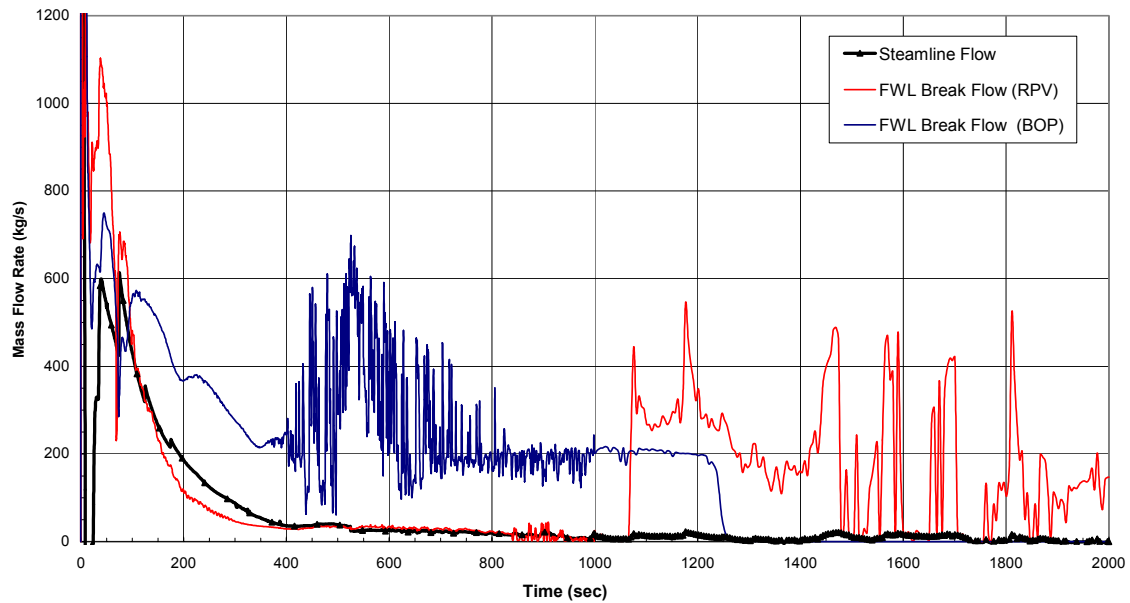
Figure 6.3-11. Steam Line and Break Flow, Feedwater Line Break, 1 GDCS Valve Failure
