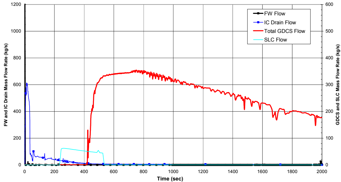
Figure 6.3-21. Flows Into Vessel, Inside Steam Line Break, 1 GDCS Valve Failure
