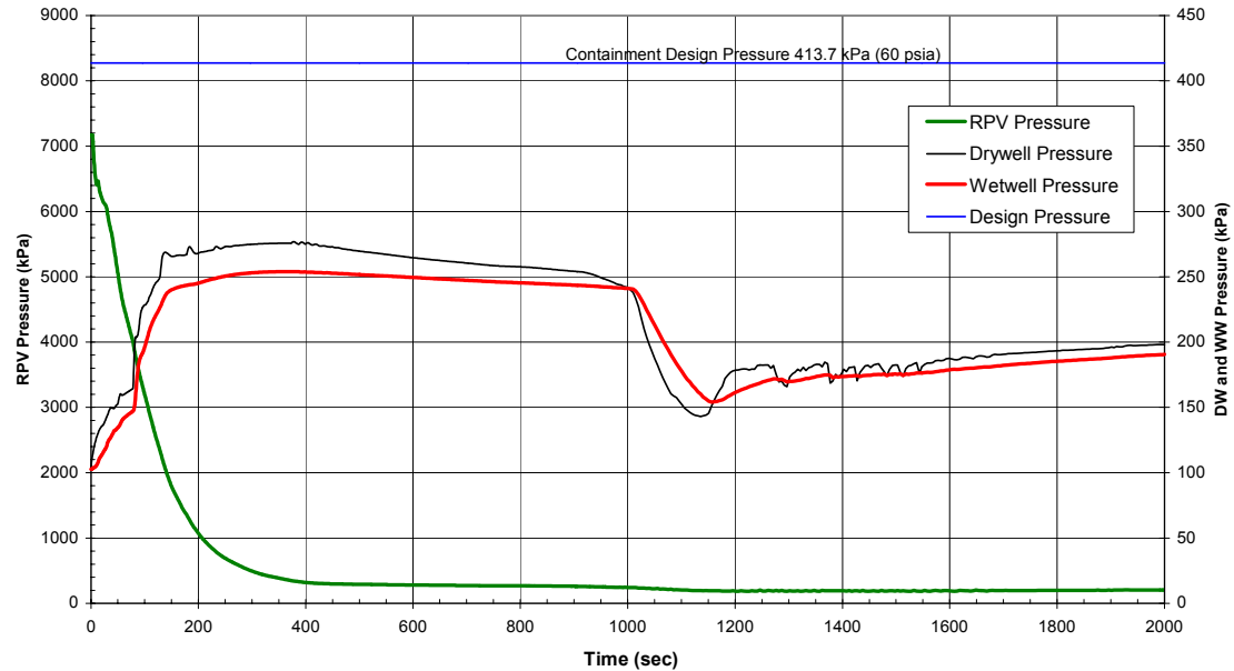
Figure 6.3-34. System Pressures, GDCS Injection Line Break, 1 GDCS Valve Failure
