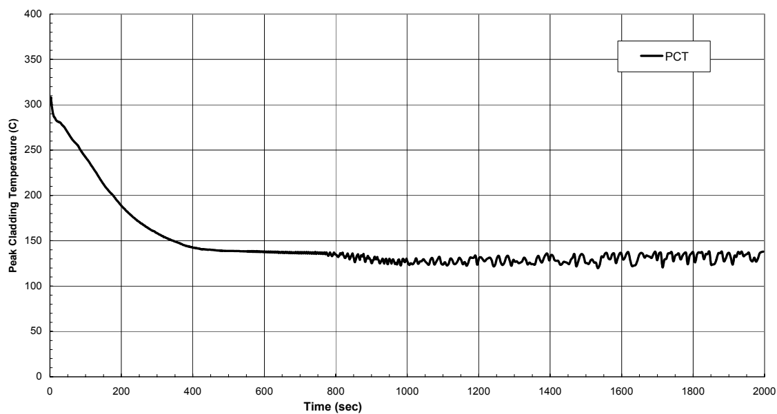
Figure 6.3-30. PCT, Bottom Drain Line Break, 1 GDCS Valve Failure
