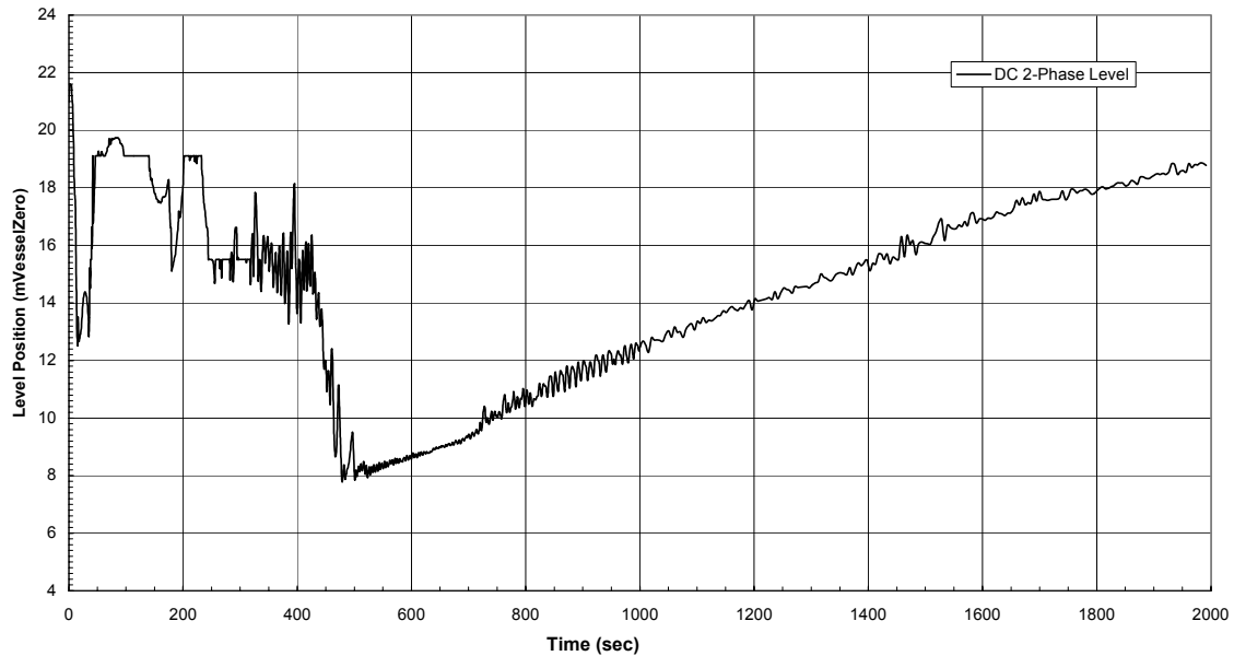
Figure 6.3-17. Downcomer Water Level, Inside Steam Line Break, 1 GDSC Valve Failure
