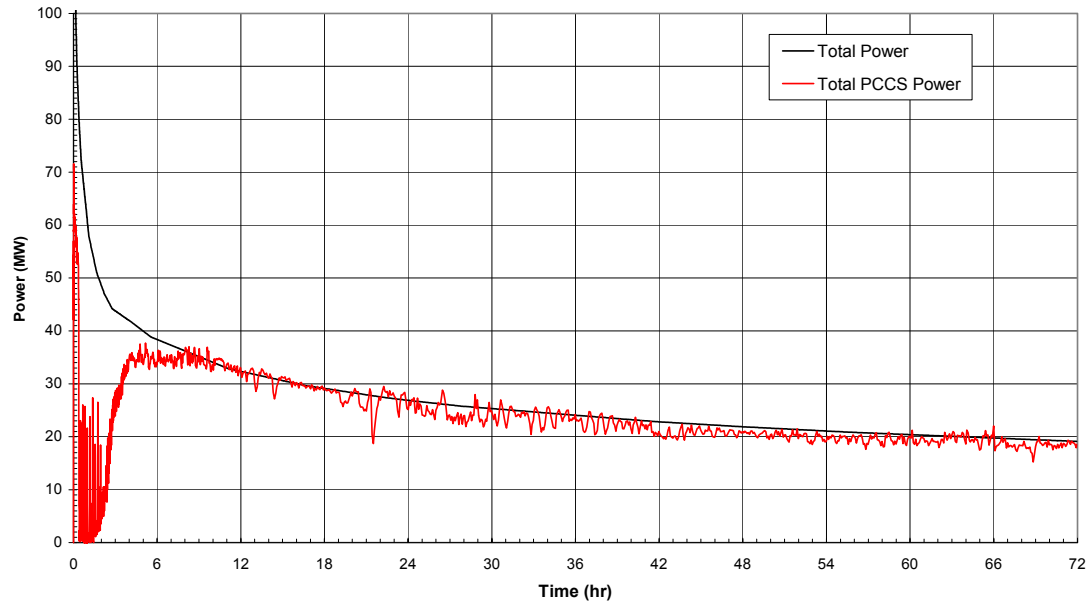
Figure 6.2-11. Feedwater Line Break (Nominal Case) — PCCS Heat Removal versus Decay Heat
