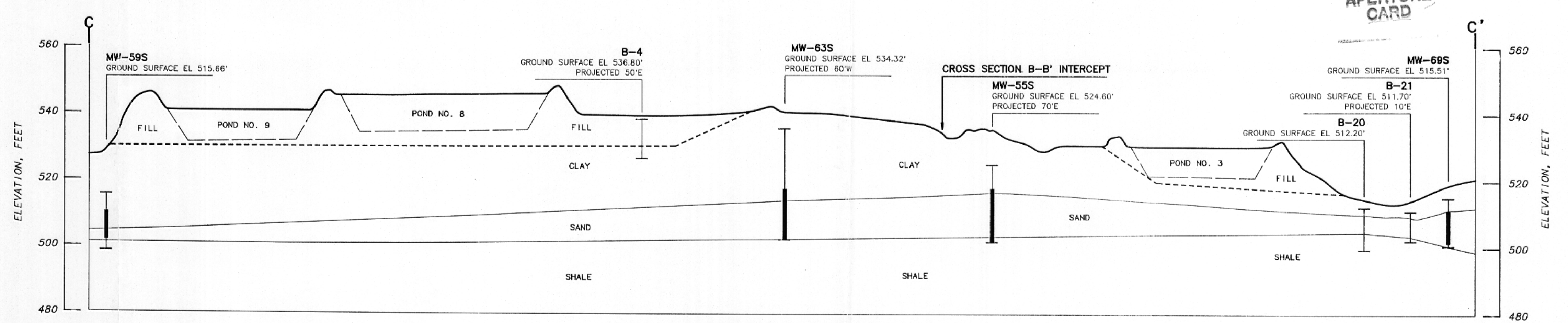
GEOLOGIC CROSS SECTION C-C' (LOOKING WEST)
