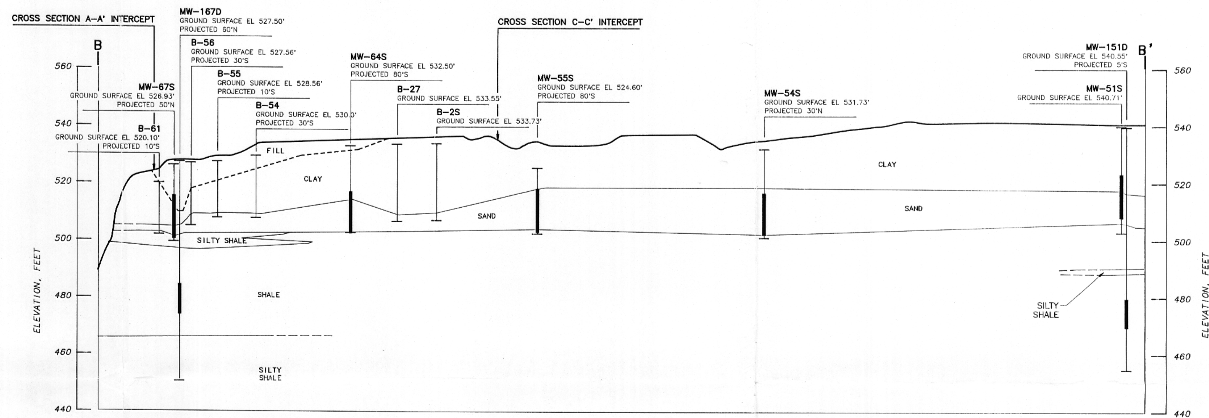
GEOLOGIC CROSS SECTION B-B' (LOOKING SOUTH)
