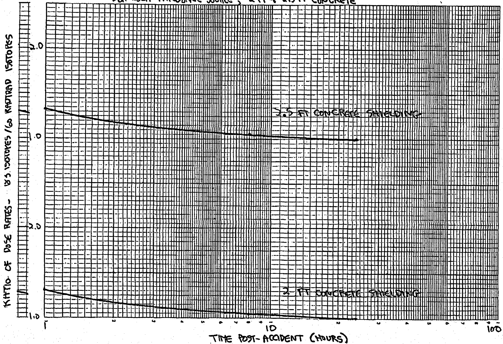
IGA FIGURE 7. RATIO OF DOSE RATES VS TIME POST-ACCIDENT DPA-LOCA AIRBORNE SOURCE ; 2 FT + 2.5 FT CONCRETE
