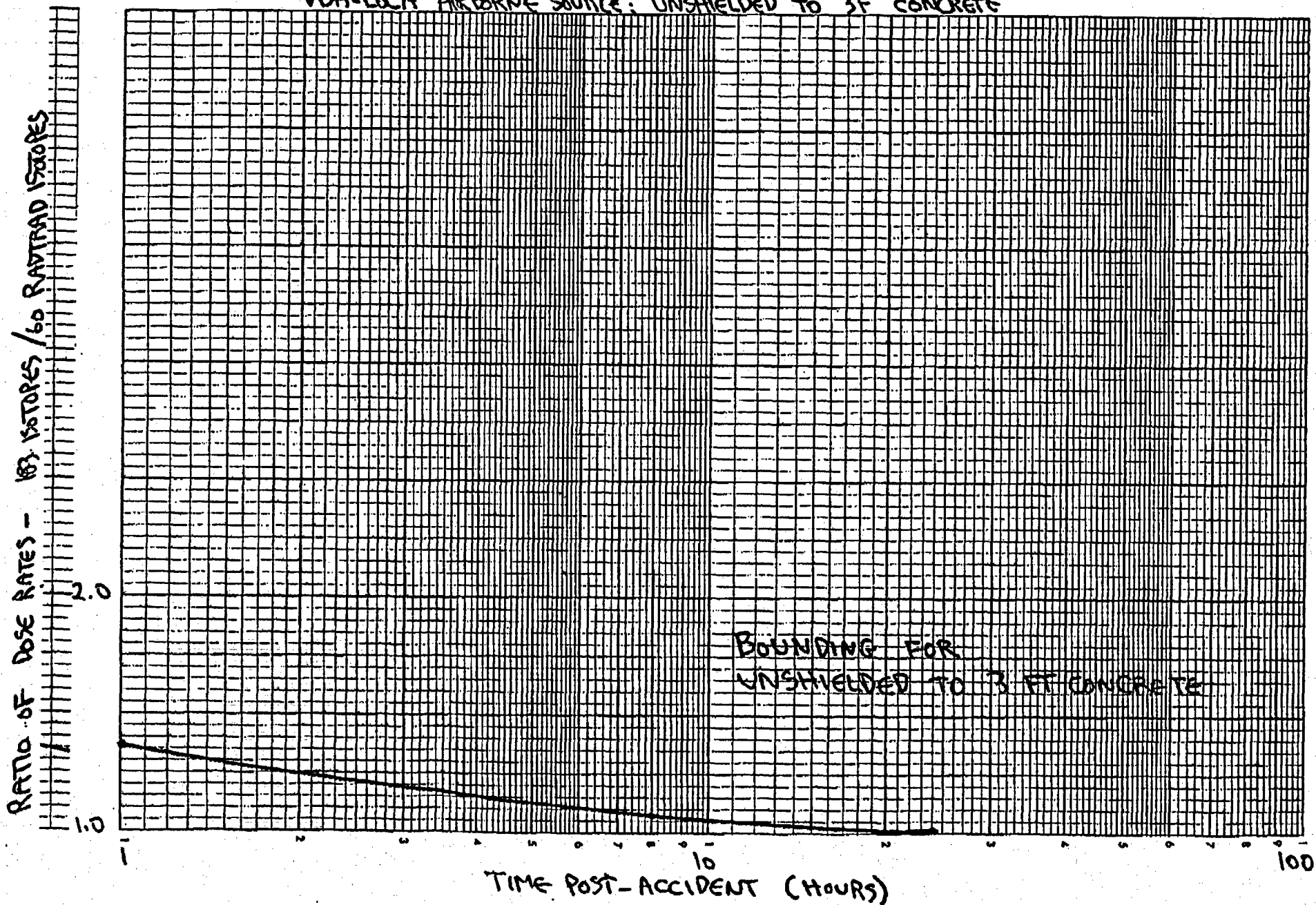
FIGURE 3. RATIO OF DOSE RATES VS. TIME POST-ACCIDENT DPA-LOCA AIRBORNE SOURCE: UNSHIELDED TO 3F CONCRETE
