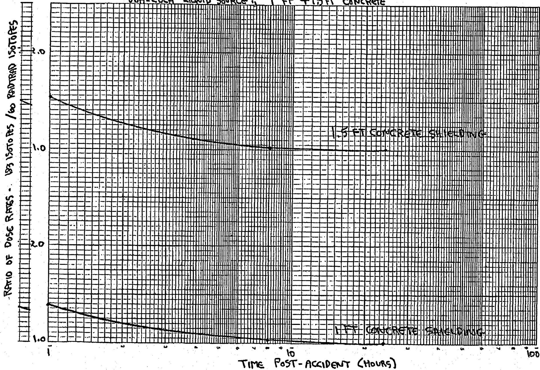
FIGURE 2. RATIO OF DOSE RATES VS TIME POST-ACCIDENT DBA-LOCA LIQUID SOURCE, 1 FT & 1.5 FT CONCRETE
