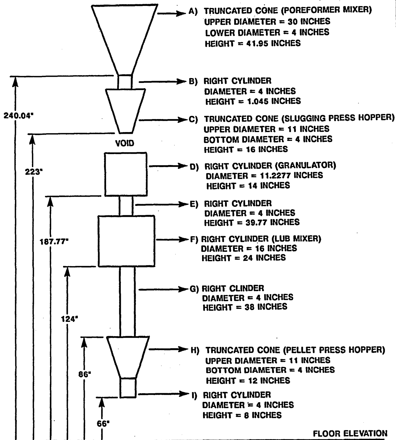
FIGURE II.8.3-13 KENO MODEL FOR PELLETIZING LINE (FOR GENERALIZED GEOMETRY OPTION)
