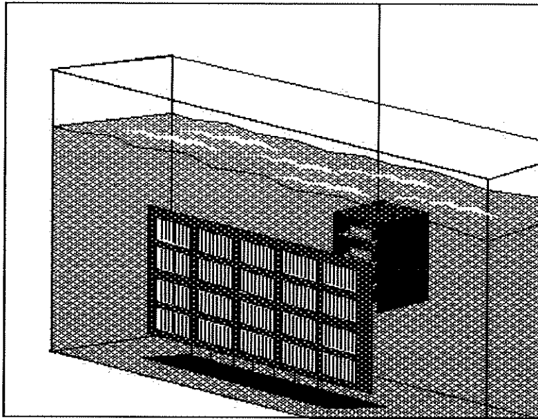
Figure 1 Irradiator. The sources remain in the water at all times. The product to be irradiated is placed in a water-tight container and lowered into the water.
