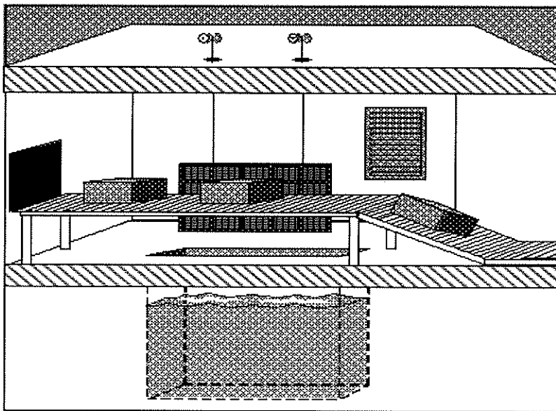
Figure 2 Commercial Wet-Source-Storage Irradiator. The sealed sources are stored in water and raised into the air
