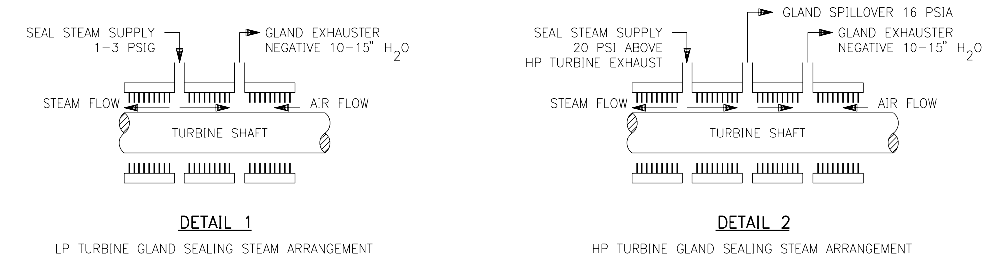
DETAIL 1 LP TURBINE GLAND SEALING STEAM ARRANGEMENT
