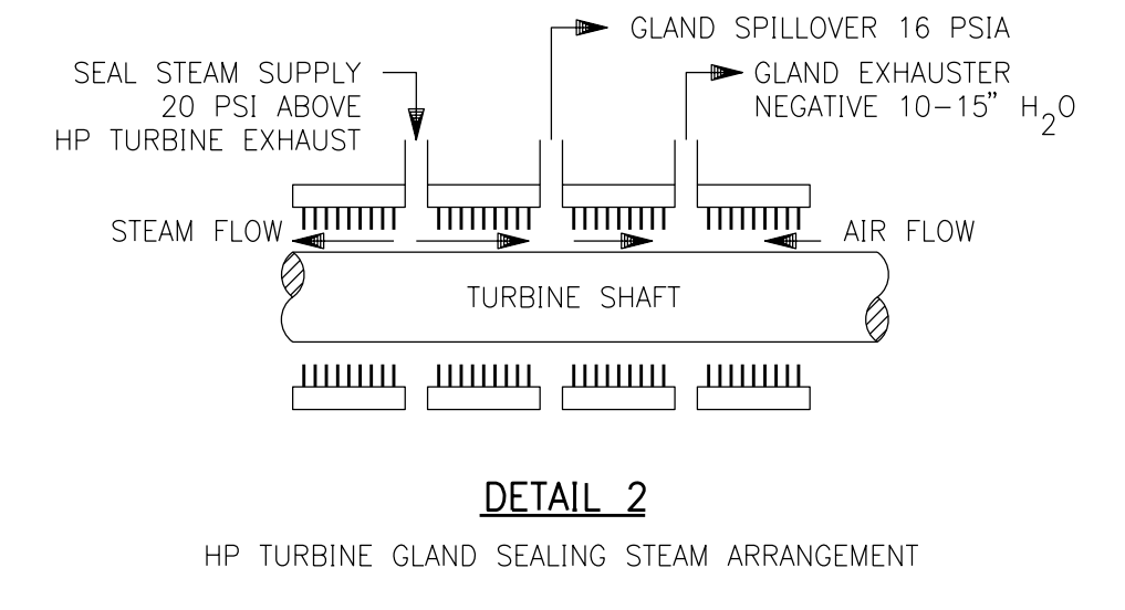
DETAIL 2 HP TURBINE GLAND SEALING STEAM ARRANGEMENT
