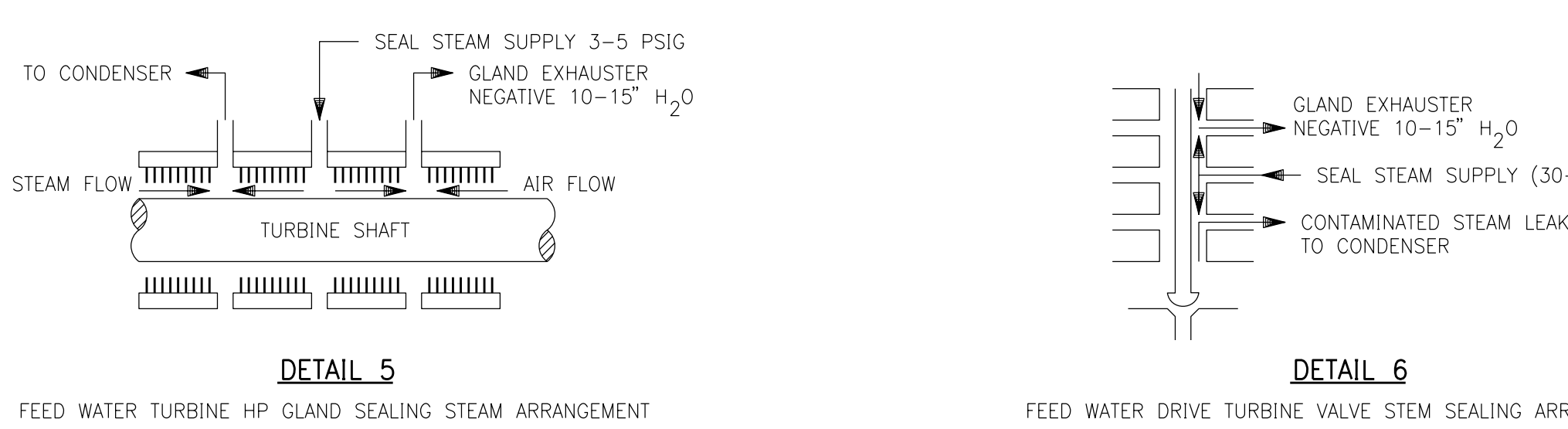
DETAIL 5 FEED WATER TURBINE HP GLAND SEALING STEAM ARRANGEMENT
