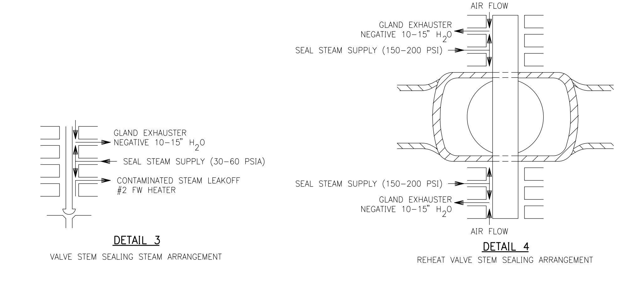
DETAIL 3 VALVE STEM SEALING STEAM ARRANGEMENT
