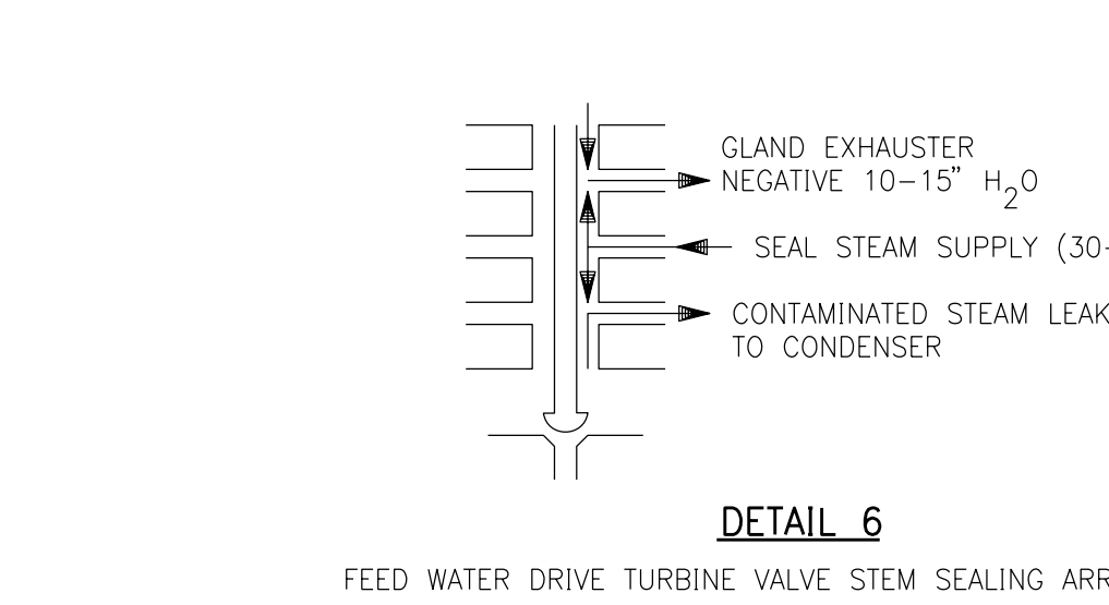
DETAIL 6 FEED WATER DRIVE TURBINE VALVE STEM SEALING ARRANGEMENT
