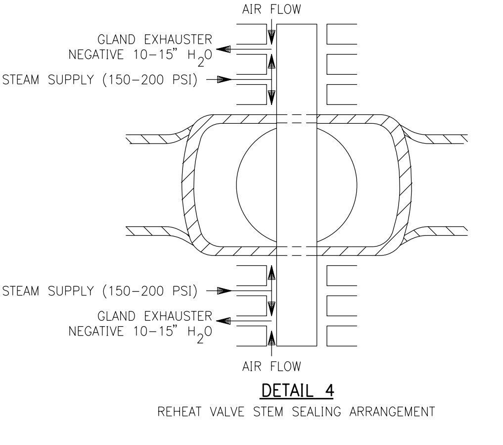
DETAIL 4 REHEAT VALVE STEM SEALING ARRANGEMENT
