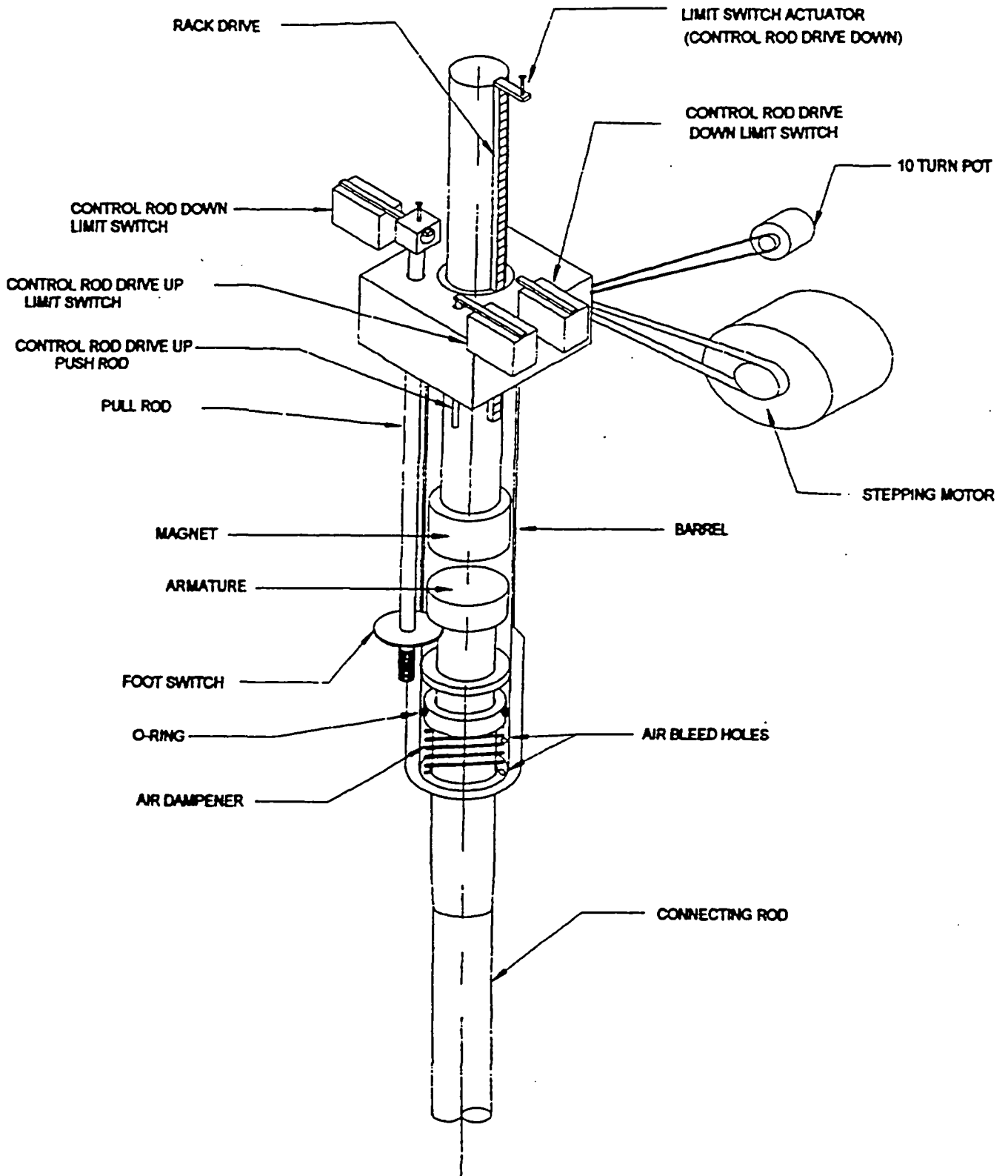
Figure 7.4 Rack-and-Pinion Control Rod Drive (Typical)
