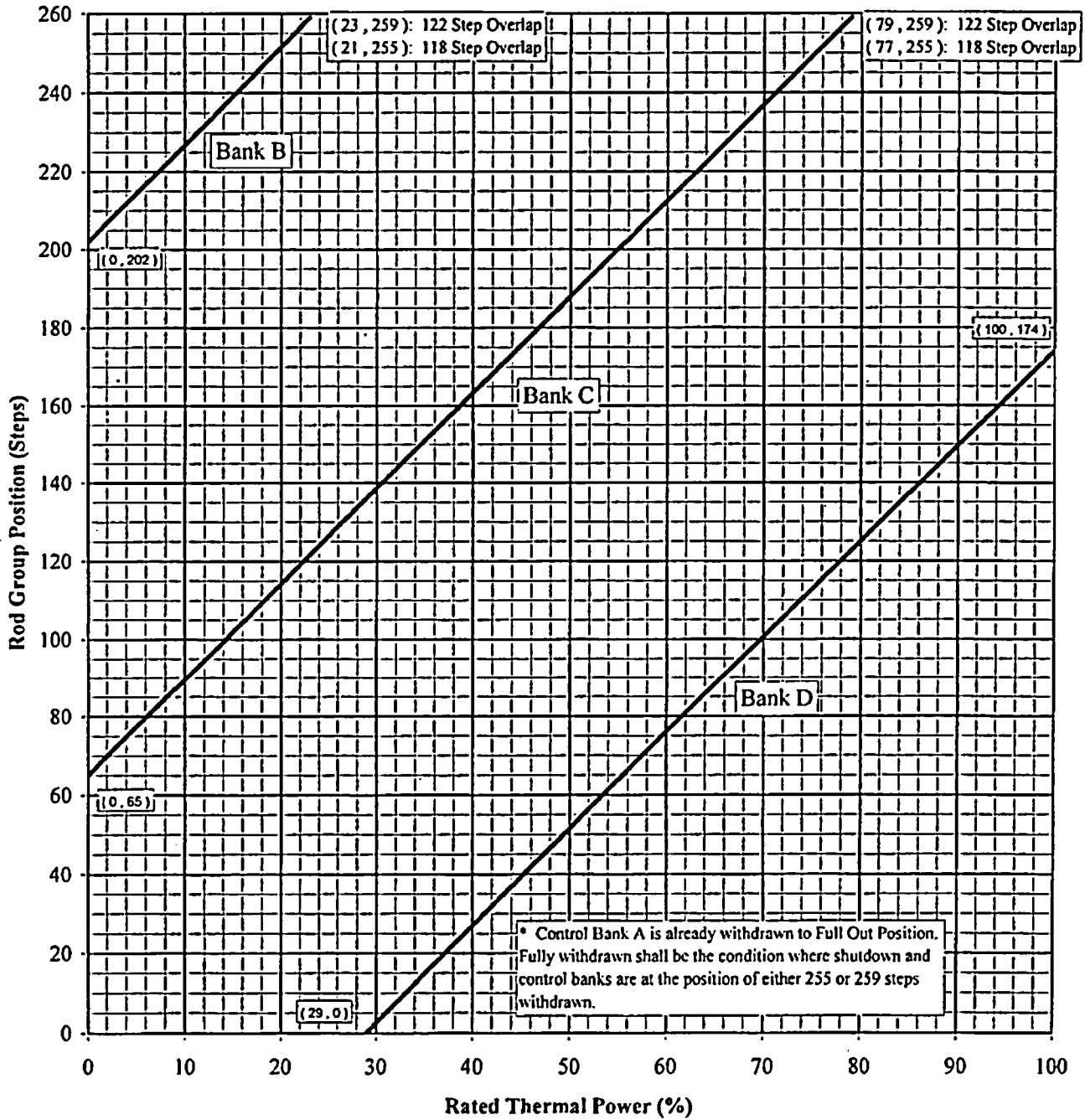
Control Rod Insertion Limits* versus Power Level
