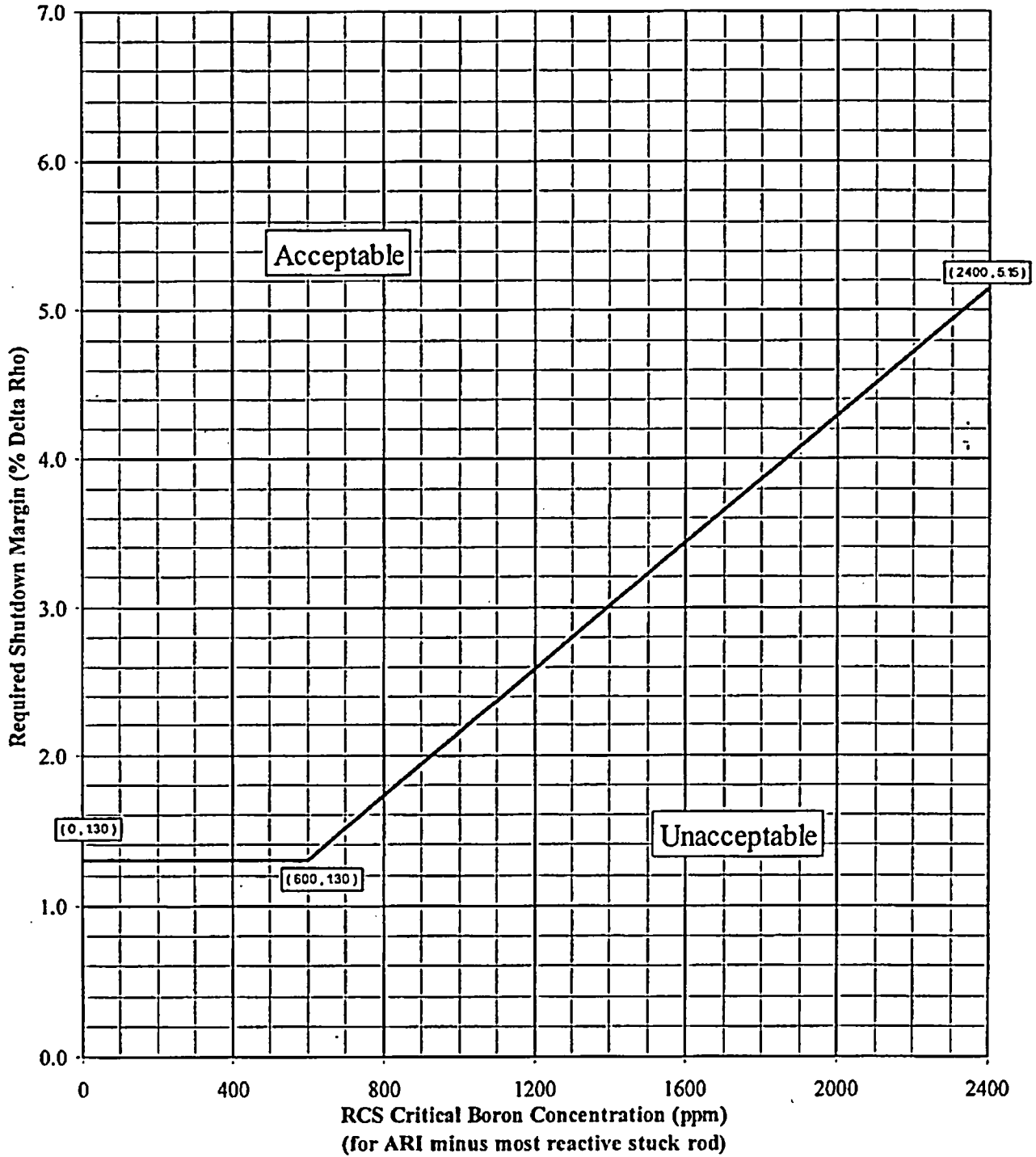
Required Shutdown Margin for Modes 3 & 4
